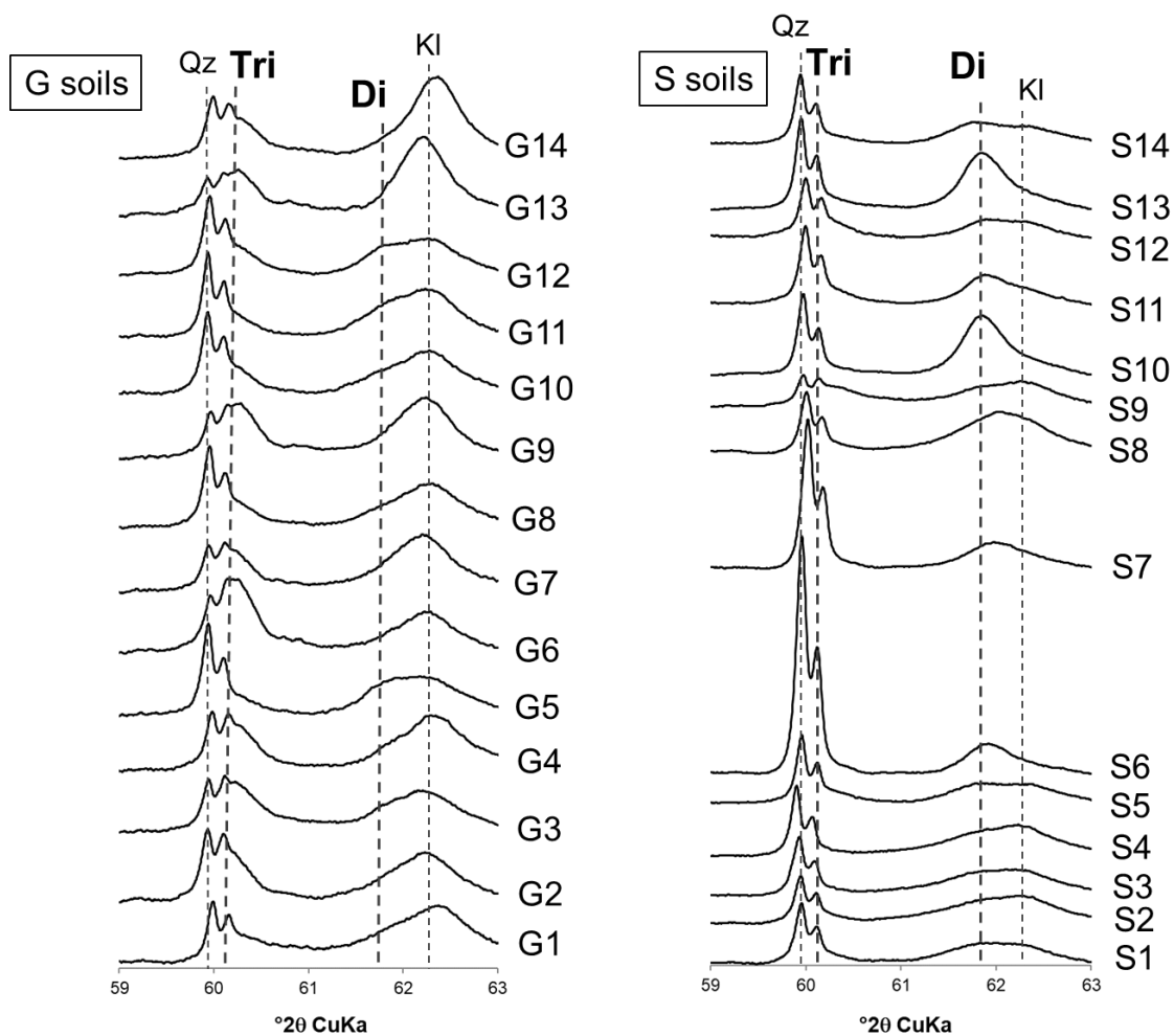
Fig. 2 X-ray diffraction patterns for clay-silt fraction collected from soil samples.
