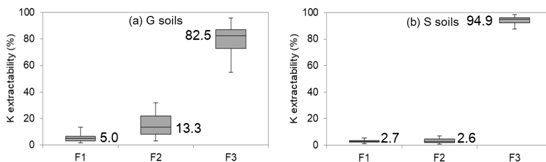
Fig. 3 The extractability of K for (a) G soils and (b) S soils in each fraction. The grey colored boxes describe the range of 25–75th percentiles and the horizontal line means the median value. The vertical lines describe the range of maximum and minimum values.
