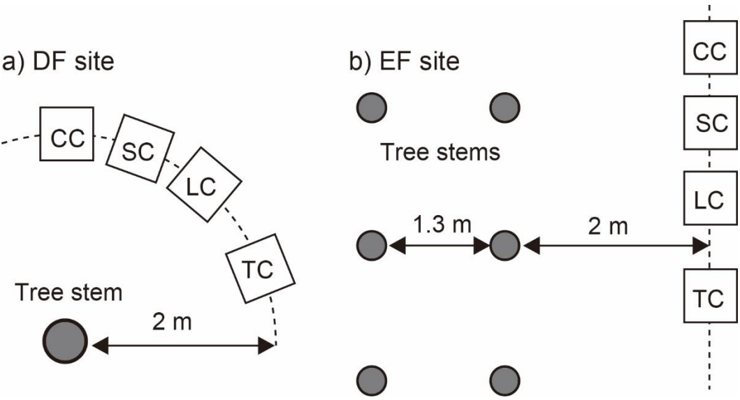
Fig. 1 Layout of collars for control (CC), sampling (SC), litter removal (LC), and trenching (TC) treatments.
