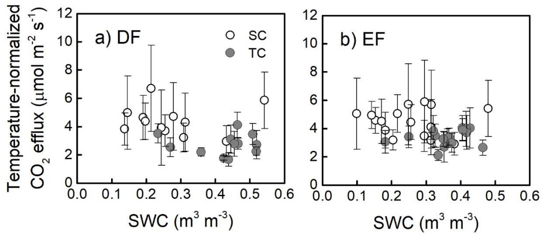
Fig. 5 Temperature-normalized soil CO 2 efflux ( R_b ) against soil water content (SWC) of 5-cm-thick surface soil for SC and TC collars in a) DF (at 14°C) and b) EF (at 12 °C) sites. Mean \pm 1 SD are shown ( n = 5 ).
