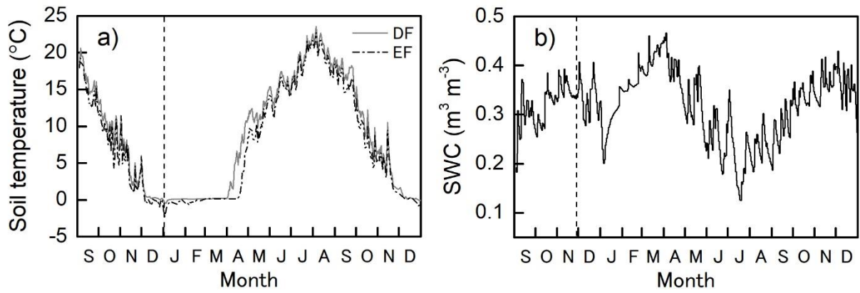
Fig. 2 Seasonal variations in daily mean a) soil temperature ( T_s ) at a depth of 5 cm ( n = 2 ) and b) soil water content (SWC) at a depth of 3 cm ( n = 4 ) from September 2014 through December 2015. SWC was measured at a nearby re-growing forest site.
