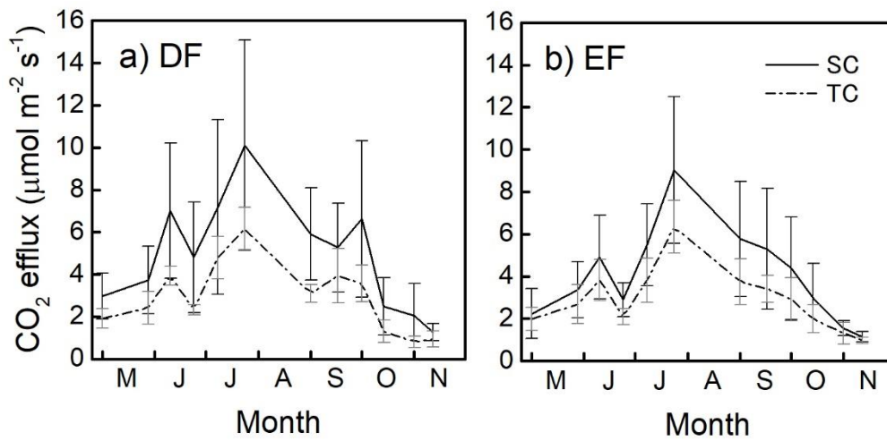
Fig. 3 Seasonal variations in soil \text{CO}_2 efflux measured on SC and TC collars in a) DF and b) EF sites. Mean \pm 1 SD are shown ( n = 5 ).
