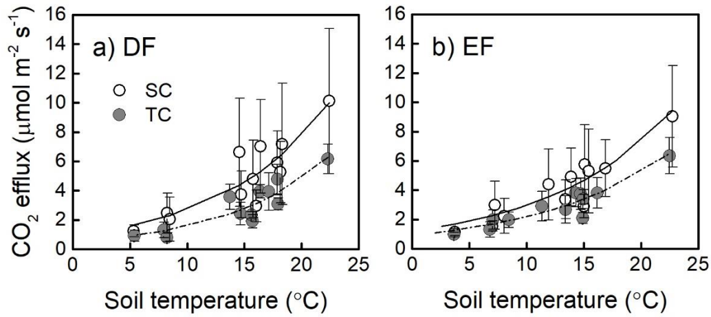
Fig. 4 Relationship between soil CO 2 efflux and soil temperature at a depth of 5 cm for SC and TC collars in a) DF and b) EF sites. Mean \pm 1 SD are shown ( n = 5 ). An exponential equation (Eq. 3) is fitted significantly ( P < 0.001 ).
