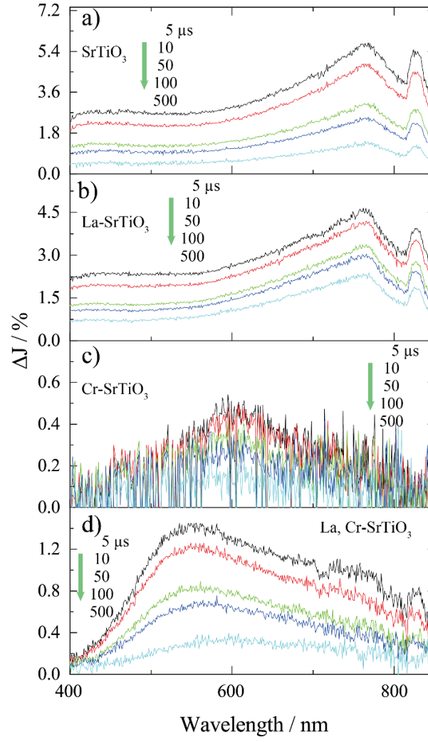
Figure 4. (a) Transient absorption spectra of SrTiO 3 (a), La-SrTiO 3 (b), Cr-SrTiO 3 (c), 3% La, Cr-SrTiO 3 (d) particles irradiated by UV (355 nm) pulsed laser under N 2 gas. The pump energy was 1.0 mJ/pulse, and the repetition rate was 10 Hz.
