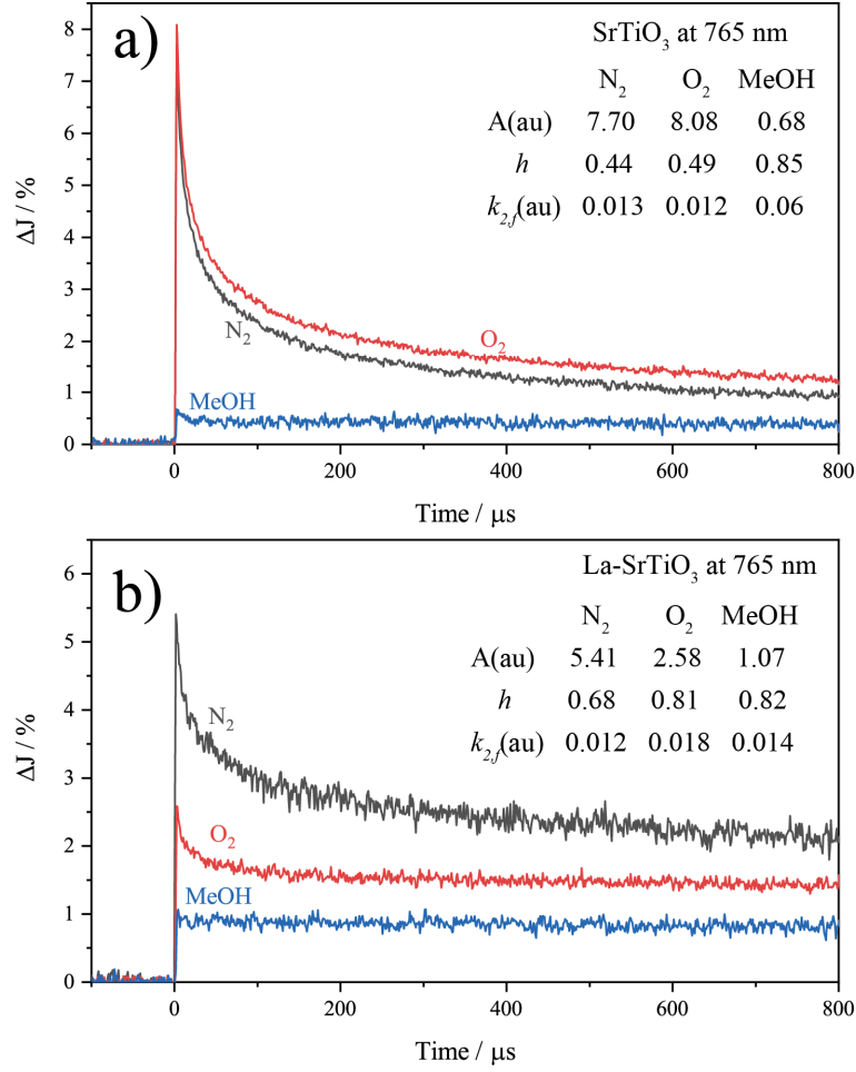
Figure 5. Decay curves of transient absorption of the SrTiO 3 at 765 nm (a), La-SrTiO 3 at 765 nm (b).
