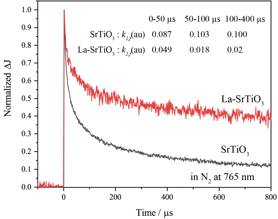
Figure 6. Comparison of the normalized decay curves of the undoped SrTiO 3 and La-SrTiO 3 in N 2 ambient at 765 nm.
