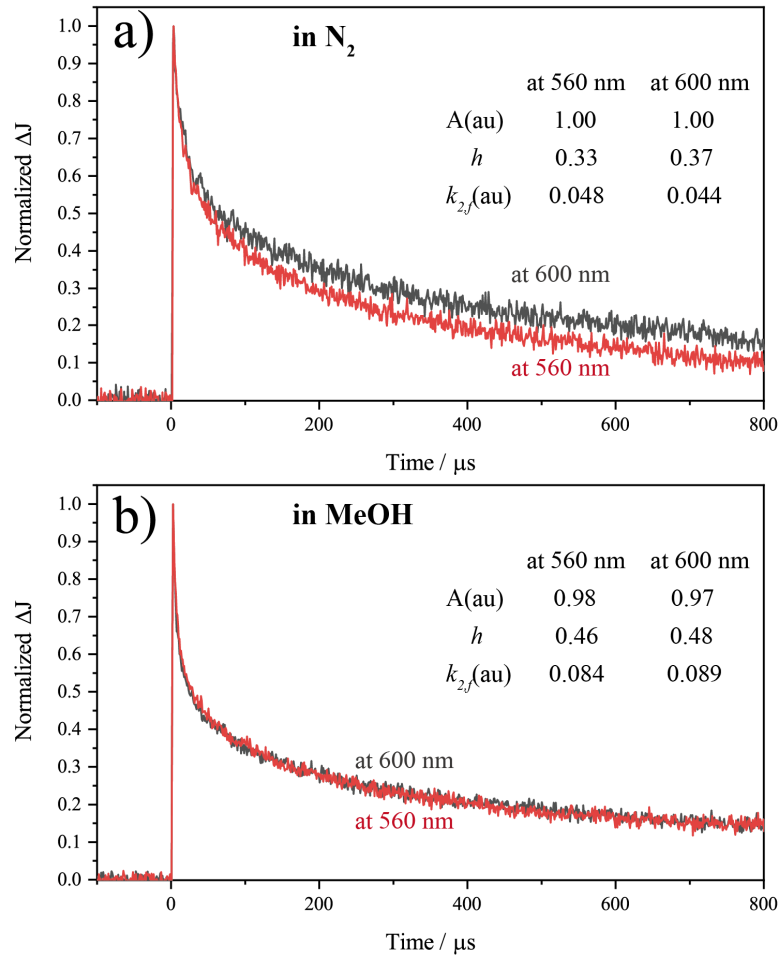
Figure 8. The comparison of 3% La, Cr-SrTiO 3 at 600 and 560 nm in N 2 ambient (a) and MeOH vapor (b).
