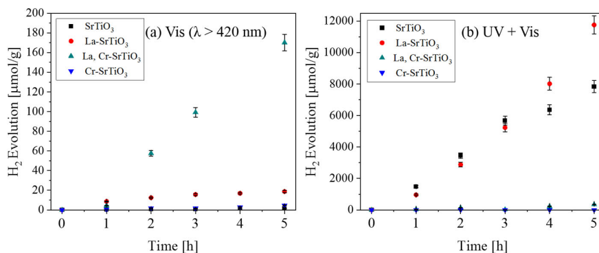
Figure 2. (a) Photocatalytic HER under visible light irradiation (b) UV+Vis light irradiation.
