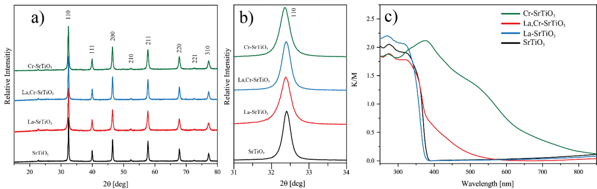
Figure 1. (a) XRD patterns and (b) (110) facet (c) UV-Vis spectra of doped and pure SrTiO_3 .
