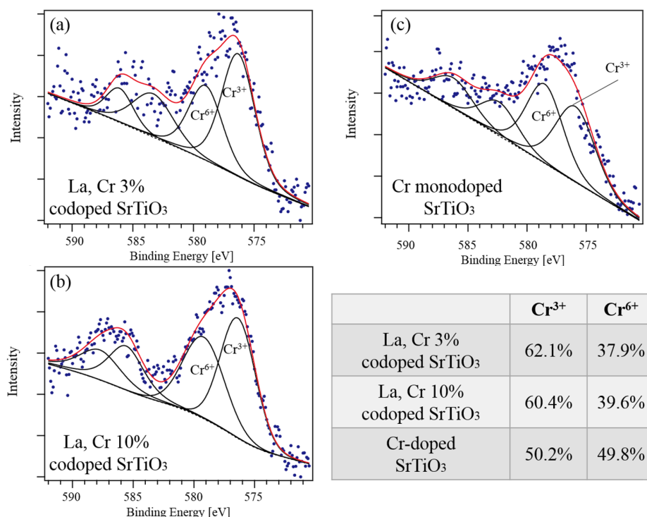
Figure 2. XPS spectra of Cr 2p in the Cr-doped SrTiO 3 and La,Cr-codoped SrTiO 3 .
