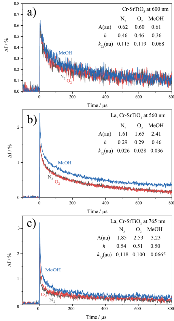
Figure 7. Decay curves of transient absorption of the Cr-SrTiO 3 at 600 nm (a), 3% La, Cr-SrTiO 3 at 560 nm (b) and 765 nm (c).
