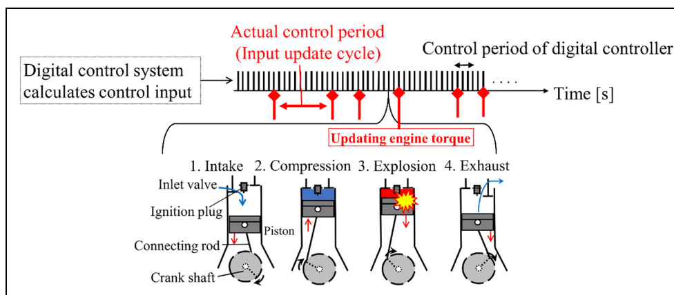
Figure 1. Limitation of the control period due to the mechanism generating engine torque.
