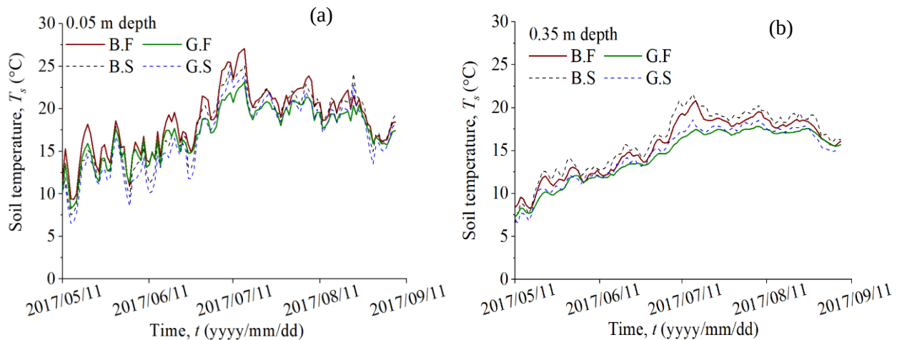
Figure 8.23 Comparison in soil temperature in bare slope and grassed slope.
