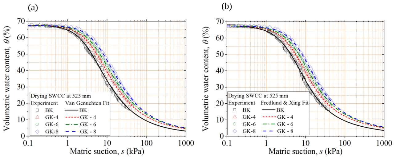
Figure 6.1 Comparisons of measured and fitted SWCCs by (a) Van Genuchten (1980) model, and (b) Fredlund and Xing (1994a) model of bare soil and grassed soils.
