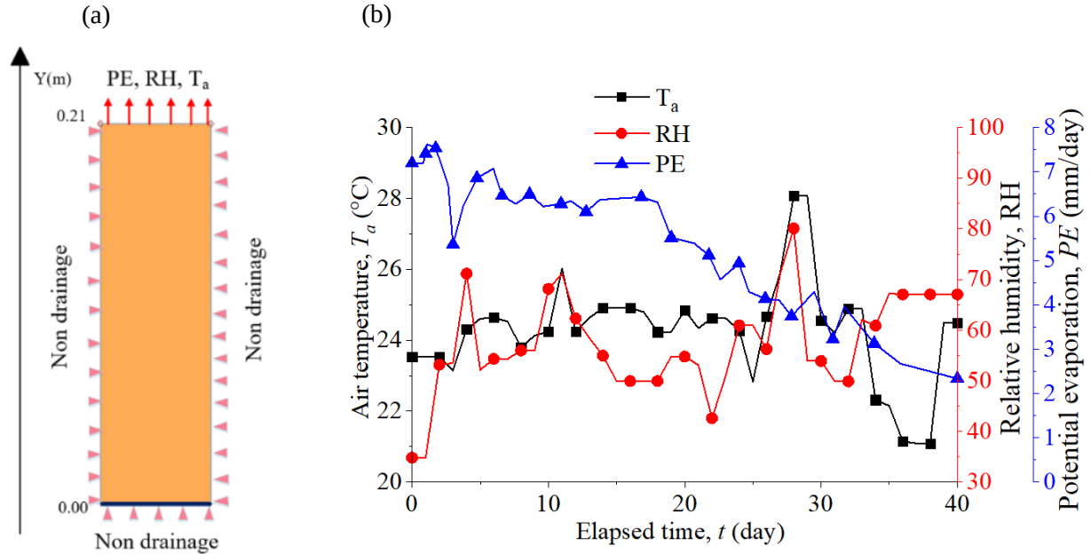
Figure 8.7 (a) Geometry, and (b) boundary conditions of soil columns simulation.
