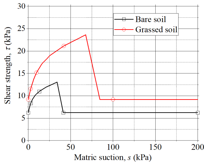
Figure 8.20 Estimations of unsaturated shear strength of bare soil and grassed soil.
