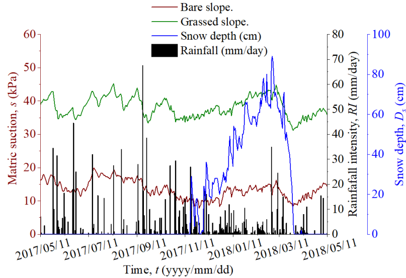
Figure 3.12 Soil suction at 25 cm depth of bare slope and grassed slope.
