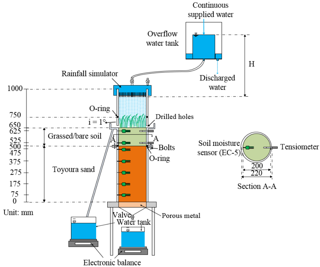
Figure 5.1 Schematic diagram of the column test apparatus.
