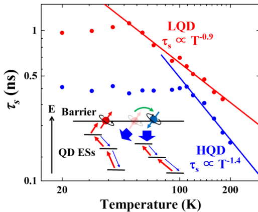
FIG. 6. \tau_s of LQD (red circles) and HQD (blue circles) as a function of temperature. The red and blue solid lines show the T^{-0.9} and T^{-1.4} dependences, respectively. The inset shows a schematic model of electron-spin dynamics at high temperatures. The red and thin blue arrows represent the thermal excitation and relaxation of electron spins among the QDs, respectively. The green and thick blue arrows represent the electron-spin relaxation in the barrier and the reinjection of electron spins from the barrier into the QD ESs, respectively.
