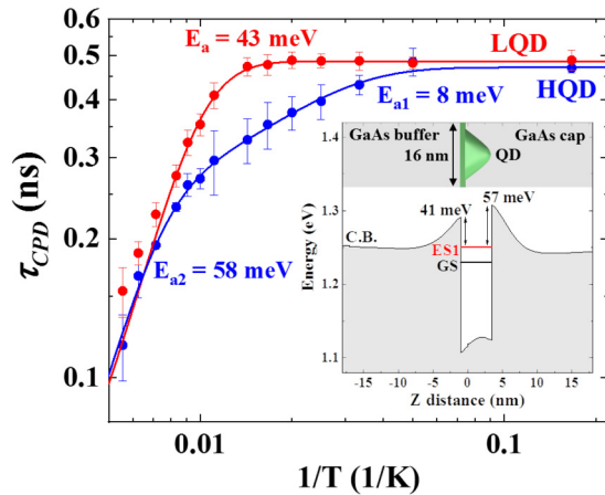
FIG. 3. \tau_{CPD} of LQD (red circles) and HQD (blue circles) as a function of temperature. The red and blue solid lines indicate the Arrhenius fitting results. The inset shows the conduction-band profile and the eigenstates for a QD with a base length of 16 nm along the stacking direction, where the influence of strain on the band structure is considered.
