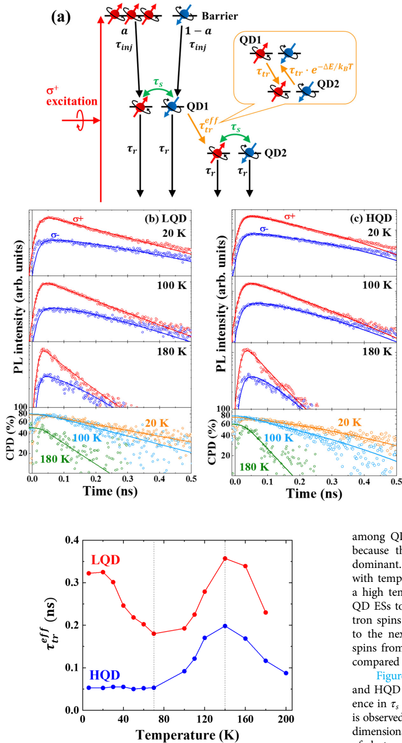
FIG. 5. \tau_{tr}^{eff} of LQD (red circles) and HQD (blue circles) as a function of temperature, deduced from the rate equation fitting.
