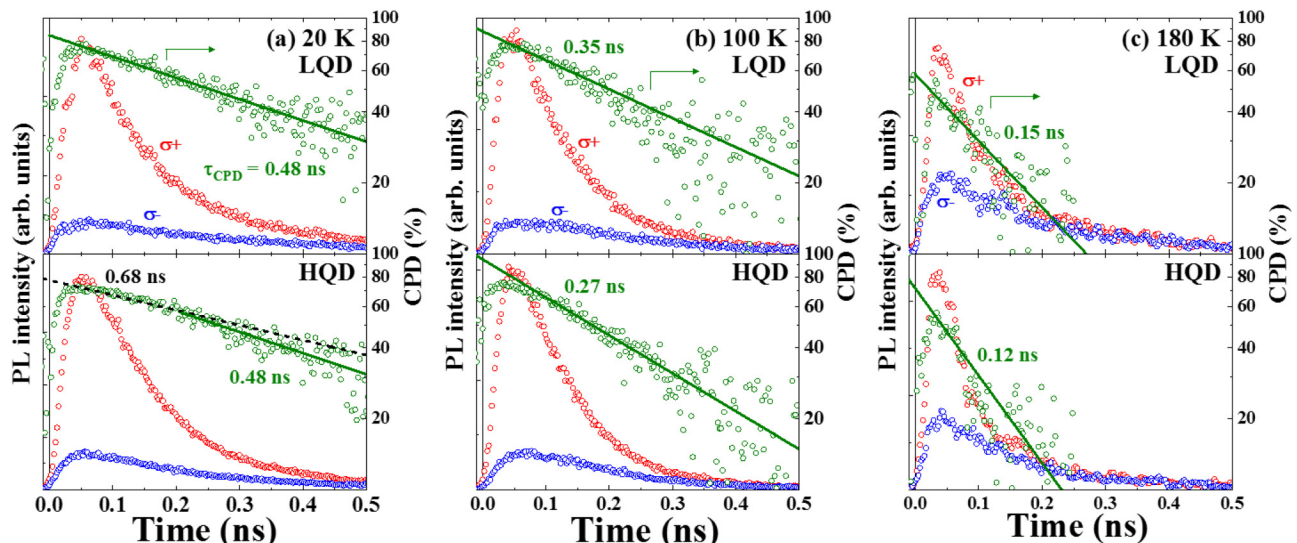
FIG. 2. Circularly polarized PL time profiles and the corresponding CPD for the QD ES (represented by yellow rectangles in Fig. 1) at (a) 20 K, (b) 100 K, and (c) 180 K. The solid lines show the single-exponential decay fittings for the time-dependent CPD. The temporary long CPD decay is seen in the initial time region for HQD at 20 K (the black broken line).
