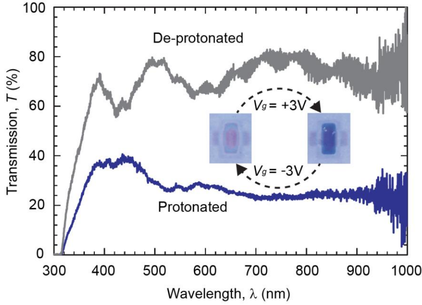
Fig. 2. Optical transmission spectra of the flexible ECT, which is composed of 50-nm-thick ITO, 10-nm-thick ZnO, 20-nm-thick NiO, 250-nm-thick TaO x , 100-nm-thick WO 3 , 10-nm-thick ZnO, and 0.1-mm-thick PET. The optical transmission in the visible light region dramatically decreased after the protonation and it recovered after the de-protonation. The inset shows the photographs of the device. After the protonation (applied V_g = +3V ), the device becomes dark blue whereas the device was transparent at the de-protonation (applied V_g = -3V ).
