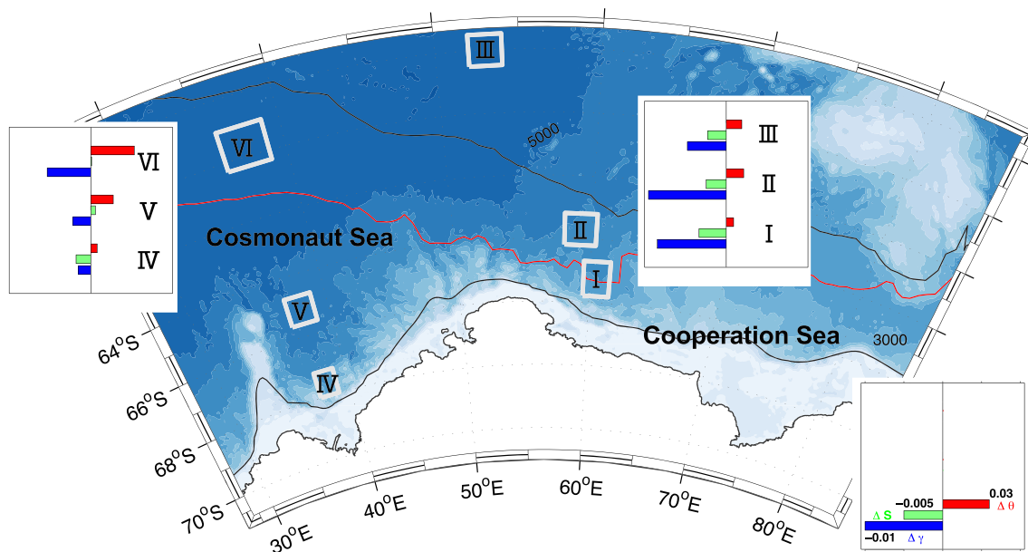
Figure 9. Summary of salinity and temperature trends in the Cooperation and Cosmonaut Seas. Bar charts show the difference between 1974 and 2016 of potential temperature (red) and salinity (green) for the densest water (averaged at 300 dbar above the bottom) and of bottom neutral density (blue) for the Cosmonaut Sea (left) and Cooperation Sea (right) at the location indicated by Roman numeral. The bar chart on the lower-right corner indicates an arbitrary change for each variable as a reference scale.
