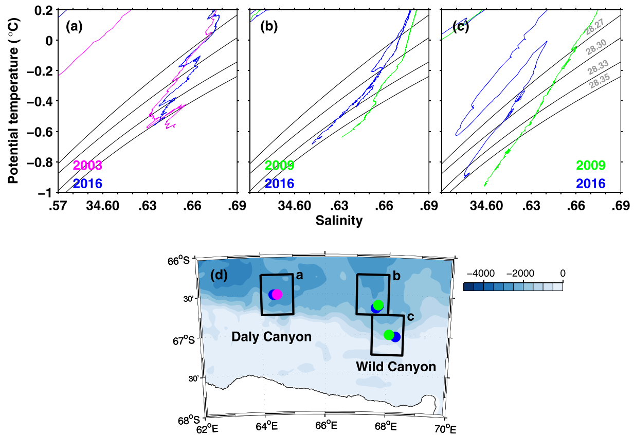
Figure 6. Potential temperature-salinity diagrams in the Cooperation Sea during 2003–2016. Data at the (a) upper continental slope in Daly Canyon, (b) upper continental slope in Wild Canyon, and (c) uppermost slope in the canyon. (d) Spatial distribution of the data (circle). Lines and circles are colored with respect to years.
