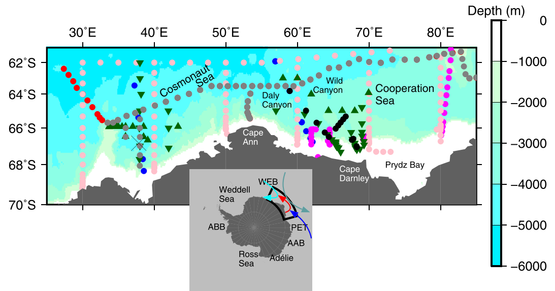
Figure 1. The study area and station locations in the Indian Ocean sector. The inset shows the location of the study area with black square. Symbols denote hydrographic stations in 1974 (blue circle; Conrad), 1996 (red circle; NBP9603), 2008 (green inverted triangle; UM0708), 2009 (green triangle/cyan; UM0809), 2013 (gray; MR12-05), and 2016 (black; KH-16). The white cross at about 38°E, 67°S denotes the location of the bottom temperature mooring. In the inset, WEB is Weddell-Enderby Basin, PET is Princess Elizabeth Trough, AAB is Australia-Antarctic Basin, and ABB is Amundsen-Bellinghousen Basin. Cape Darnley Bottom Water originates from the Cape Darnley Polynya (red arrow), mixed with the westward flowing Antarctic Bottom Water from the AAB through the Princess Elizabeth trough (PET; blue arrow). Weddell Sea deep water recirculates at the eastern margin of the Weddell Gyre (cyan arrow). To the north, the Antarctic circumpolar current carries AABW eastward from the WEB to AAB (green arrow).
