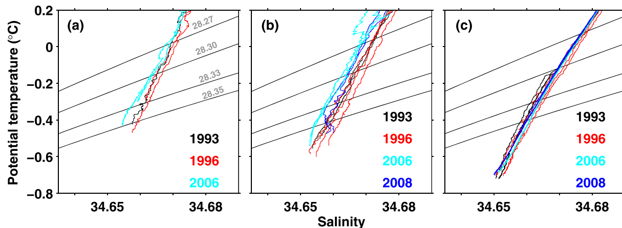
Figure 7. Potential temperature-salinity diagrams along the WHP I6 line (30°E) during 1993–2008. Data at the (a) uppermost continental slope at ~68.5°S, (b) upper slope between 67–68°S, and (c) deep basin between 61.5°S and 63°S.
