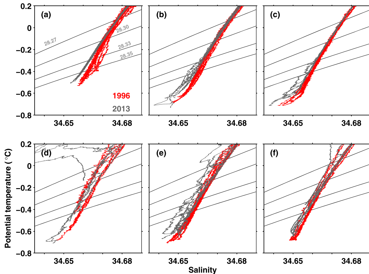
Figure 4. Potential temperature-salinity diagrams in the Cooperation and Cosmonaut Seas along the WHP S4I section for 1996 and 2013 cruises. (a) 62–80°E, (b) 55–62°E, (c) 50–55°E, (d) cross-slope section along 53°E, (e) 40–50°E, (f) 34–40°E. Red lines denote observations in 1996 and gray lines in 2013.
