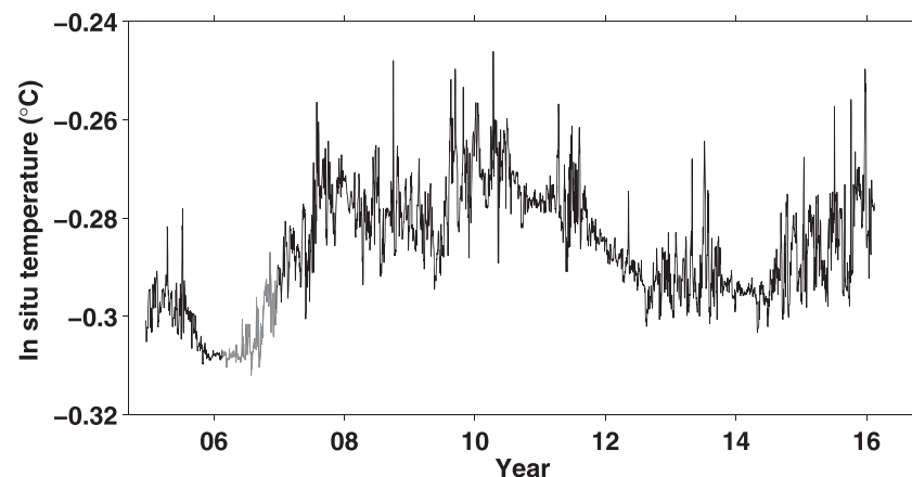
Figure 8. Time series of in situ temperatures (°C) of bottom pressure gauges during 2005–2016 at 37°50'E, 66°51'S in the Cosmonaut Sea. The gray line indicates gap periods where data were substituted with temperatures derived from the sensor attached to the pressure gauge.
