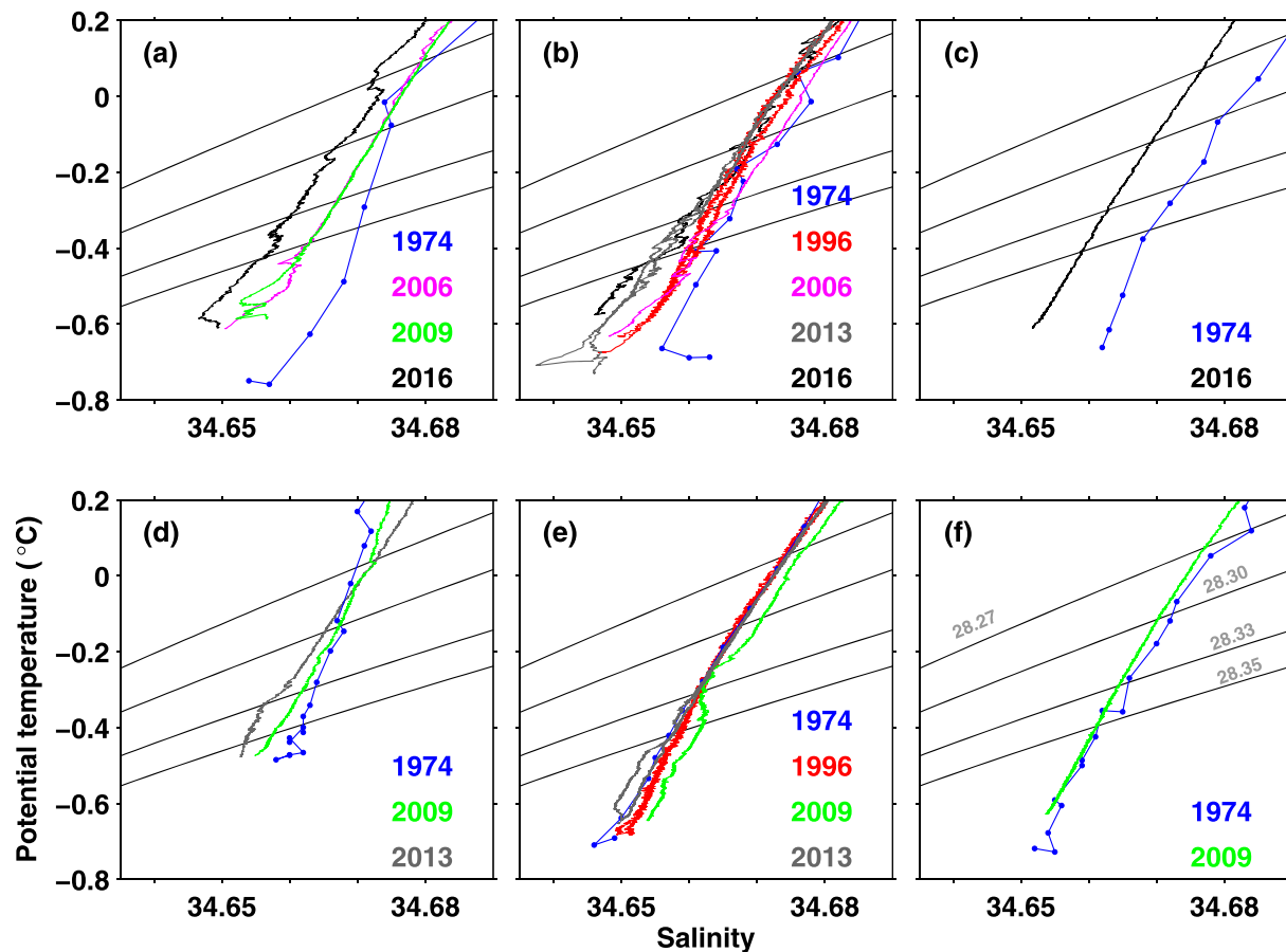
Figure 5. Potential temperature-salinity diagrams in the Cooperation Sea (a–c) and Cosmonaut Sea (d–f) for observations during 1974–2016. (a) 61°E, 65°S, (b) 59°E, 64°S, (c) 53°E, 58°S, (d) 38°E, 68°S, (e) 38°E, 65°S, and (f) 38°E, 60°S. Lines are colored with respect to years.
