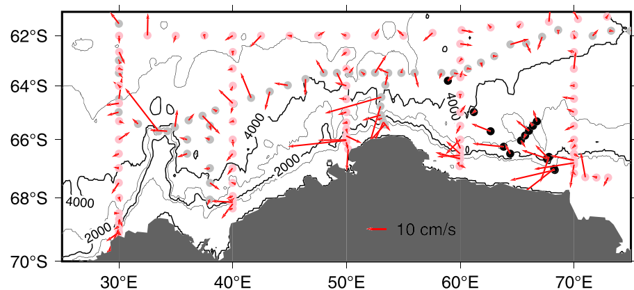
Figure 3. Spatial distribution of bottom velocity vectors. Velocity vectors are averaged for the 50-m-thick layer above the bottom, derived for the BROKE-West (pink dots), MR12-05 (gray dots), and KH16-1 (black dots) cruises.
