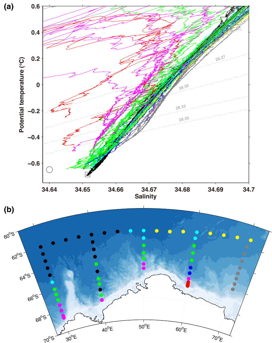
Figure 2. (a) Potential temperature-salinity diagram for BROKE-West section between 30°E and 70°E and (b) distribution of data points with information of varieties of the AABW. Dashed black lines in (a) denote neutral density contours with values shown in gray numerals. Colors denote different fraction of CDBW for bottom 300 dbar average property, calculated based on the three endmembers of CDBW (○), WSDW (□), and LCDW (▽). Cyan indicates the point where CDBW fraction is more than 1% but less than 10%, green above 10%, and magenta the largest fraction among the three endmembers. Red is a transient region where the signal does not fall within the three-endmember triangle. Blue points indicate the point where the fresh signal is seen near the bottom, but vertical average does not show significant CDBW fraction. Gray indicates saltier AABW through the PET. Black denotes that the WSDW fraction is more than 90% and CDBW fraction is less than 1%. Yellow denotes AABW carried by the ACC that do not fall into other categories. See text in details.
