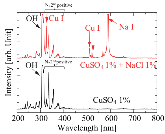
Figure 4. Optical emission spectra when \text{CuSO}_4 solutions at a concentration of 1% were used as the cathode. The lower trace was observed without the NaCl additive. The optical emission intensity of Cu was enhanced by adding 1% NaCl as shown in the upper trace. The discharge current was 90 mA.
