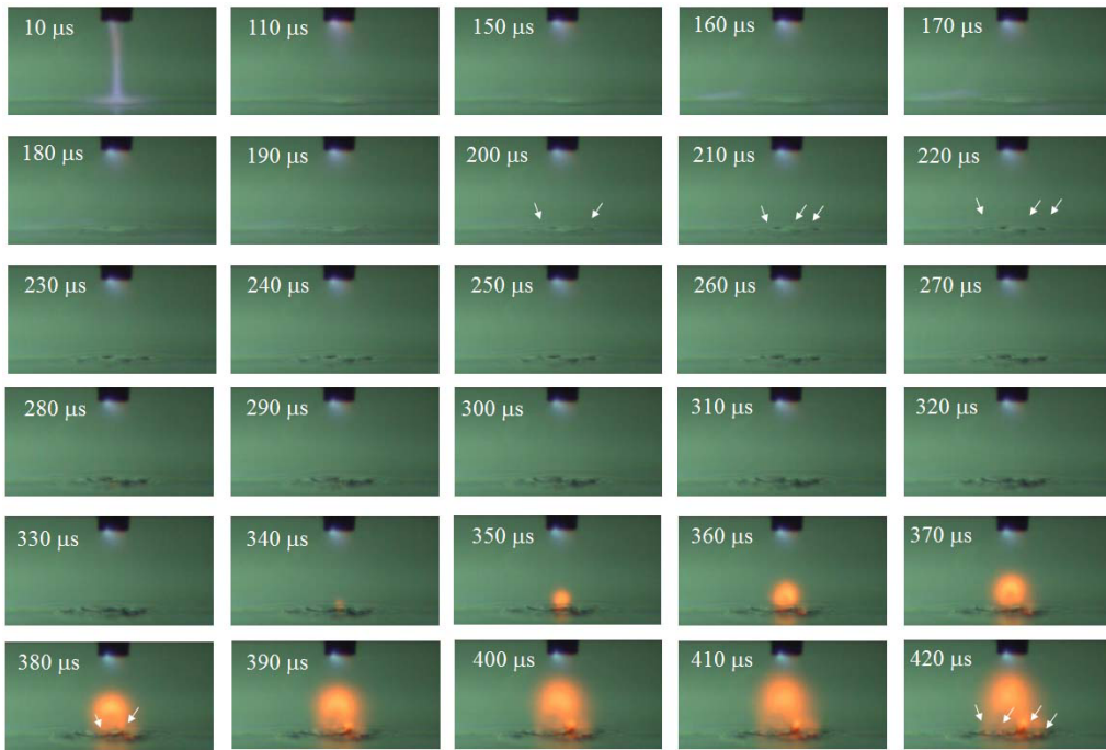
Figure 6. Temporal change in the shape of the liquid cathode surface. The frame rate of high-speed camera is 10^5 fps. Supplementary data are available from stacks.iop.org/PSST/XX/XXXXX/mmedia . (See the movie file spp3.mp4).
