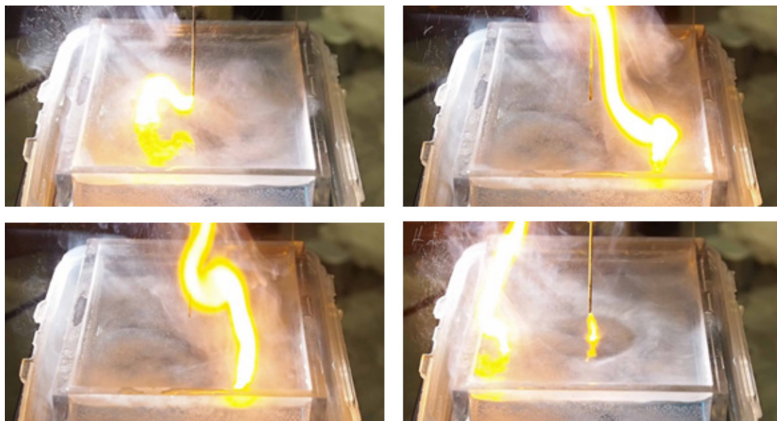
Figure 7. Explosive phenomena observed above the liquid cathode when the distance between the anode and the cathode surface was 10 mm and the discharge current was 120 mA. *Supplementary data are available from stacks.iop.org/PSST/XX/XXXXX/mmedia (See the movie file spp4.mp4).
