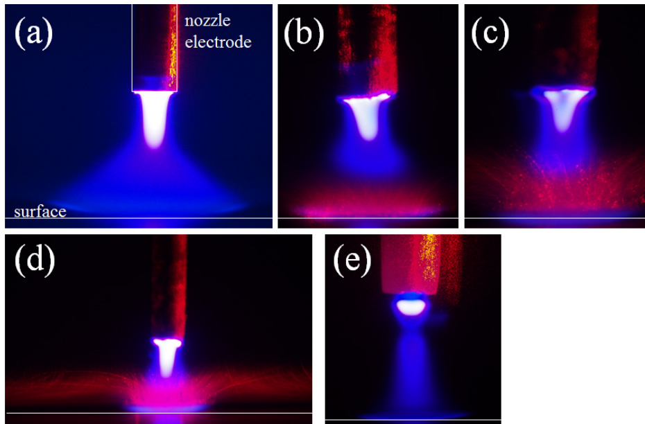
Figure 2. Visualization of droplet generation from liquid cathode surface by laser Mie scattering. (a) tap water, discharge current: 90 mA, (b) 1% NaCl solution, discharge current: 90 mA (c) 5% NaCl solution, discharge current: 90 mA (d) zoom out image of (c), and (e) liquid anode (1% NaCl solution) discharge at discharge current of 30 mA. Movie files as supplementary data are available from stacks.iop.org/PSST/XX/XXXXX/mmedia (See the movie file spp1.mp4).
