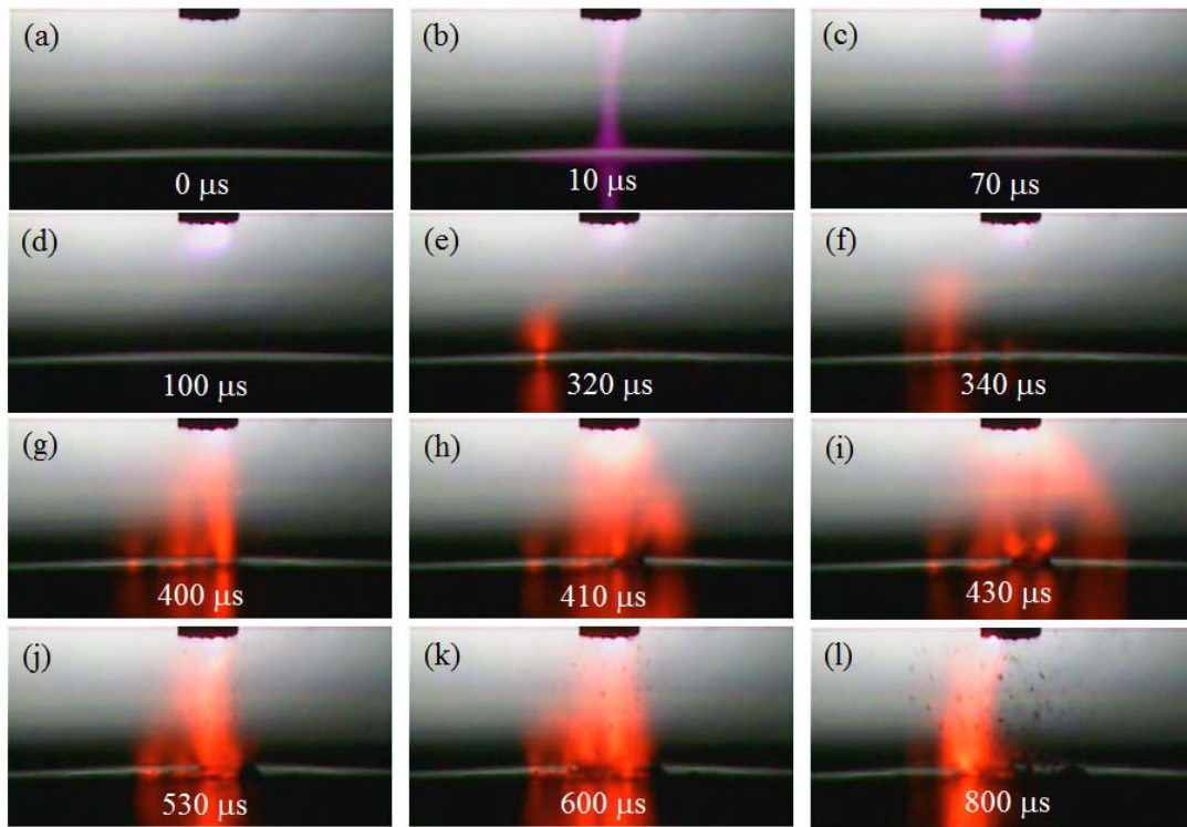
Figure 5. Time evolution of the optical emission of Na on the cathode surface when an atmospheric-pressure glow discharge with a liquid cathode is ignited. The frame rate of high-speed camera is 10^5 fps. * Movie files as supplementary data are available from stacks.iop.org/PSST/XX/XXXXX/mmedia . (See the movie file spp2.mp4).
