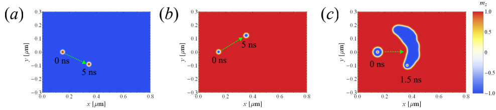
Fig. 3. The time evolution of (a) the Q = +1 skyrmion motion, (b) the Q = -1 skyrmion motion, and (c) the skyrmionium motion in the case of \alpha = 0.02 .
