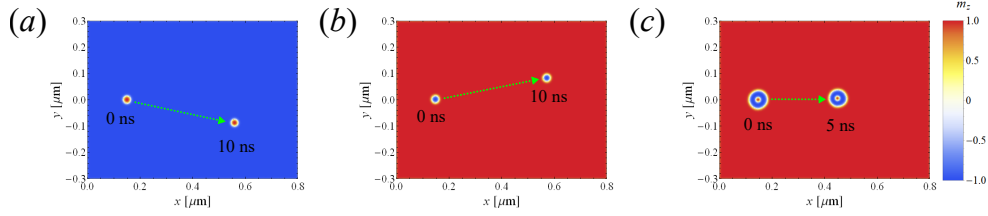
Fig. 2. The time evolution of (a) the Q = +1 skyrmion motion, (b) the Q = -1 skyrmion motion, and (c) the skyrmionium motion in the case of \alpha = 0.2 .
