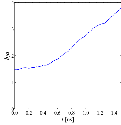
Fig. 5. The time dependence of the ratio between scaling factor a along x -direction and scaling factor b along y -direction in the case of \alpha = 0.02 .
