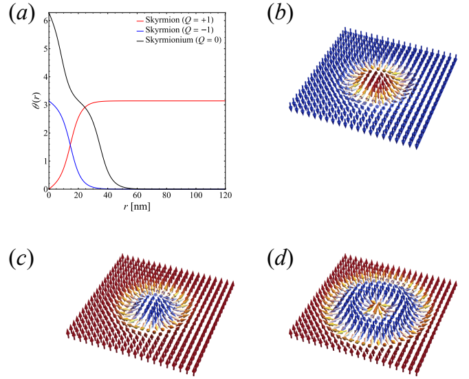
Fig. 1. (a) The angles of \theta(r) obtained using the variational method. The red, blue, and black lines represents \theta(r) of the Q = +1 skyrmion, the Q = -1 skyrmion, and the skyrmionium, respectively. Magnetization structures of (b) the Q = +1 skyrmion, (c) the Q = -1 skyrmion, and (d) the skyrmionium obtained using the above \theta(r) , respectively. In figures (b), (c), and (d), the directions and the colors of arrows represent the magnetization-direction and the magnitude of z -component of magnetization at each point, respectively.
