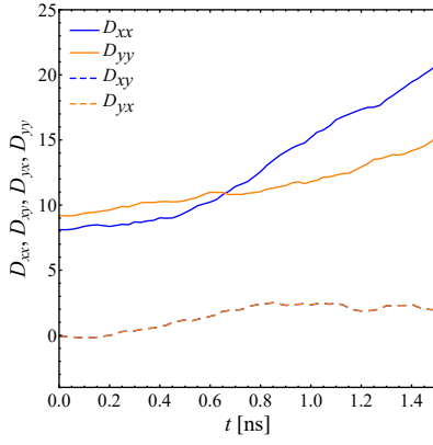
Fig. 4. The time dependence of the components of the dissipative force tensor of the skyrmionium in the case of \alpha = 0.02 . D_{xy} and D_{yx} have the same values.
