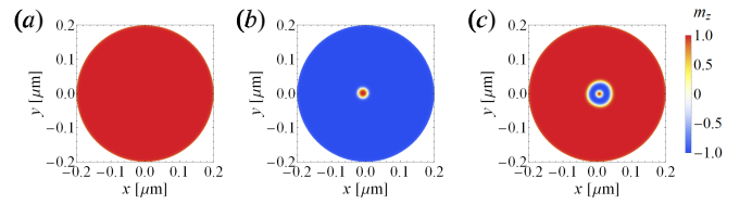
Fig. 6. Snap shots of the process of creating a skyrmionium. (a) The initial state. (b) The state after applying a pulsed magnetic field to the initial state and relaxing. (c) The state after applying a pulsed magnetic field to the state of (b) and relaxing.
