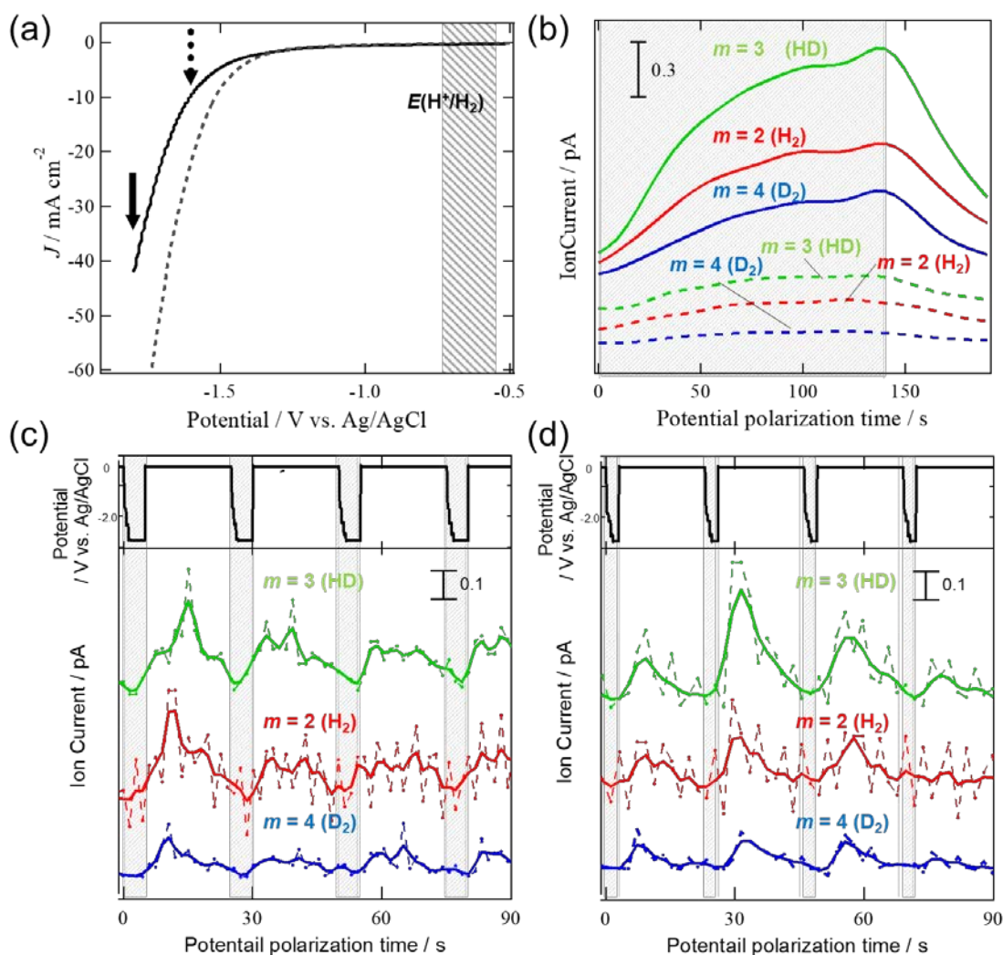
Fig. 2 | (a) Cyclic voltammograms for Ag electrode in 0.5 M Na 2 SO 4 aqueous solutions. The broken and solid lines are obtained in the solution of pure H 2 O and mixed H 2 O / D 2 O, respectively. (b) Electrochemical mass spectra obtained at potential polarization of (broken) -1.6 and (solid) -1.8 V, respectively. The potential was applied for 140 s as indicated as the shadow region. (c and d) Mass spectra obtained with repeated chronoamperometric measurements. The intervals for HER was (c) 5 and (d) 2 sec, respectively.
