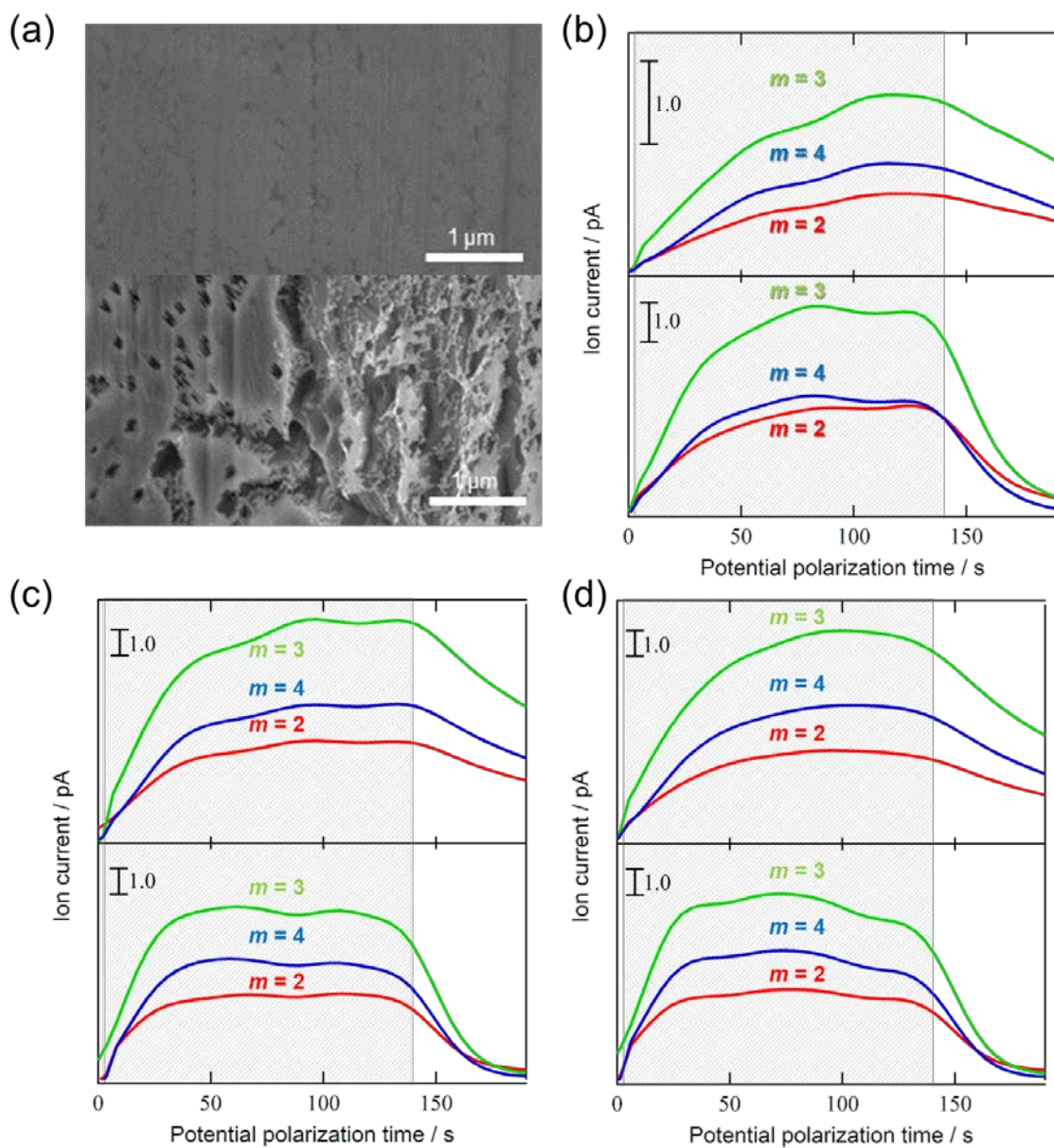
Fig. 3 | (a) SEM images of (upper) smooth and (bottom) roughened Pt surface. (b-d) Electrochemical mass spectra obtained with (upper) smooth and (bottom) roughened Pt electrodes in the mixed solution of \text{H}_2\text{O} and \text{D}_2\text{O} . The applied electrode potentials were (b) -1.6 , (c) -1.8 , and (d) -2.0 V, respectively.
