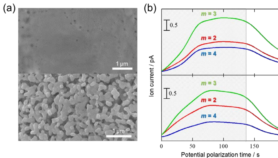
Fig. 4 | (a) SEM images of (upper) smooth and (bottom) roughened Ag surface. (b) Electrochemical mass spectra obtained with (upper) smooth and (bottom) roughened Ag electrodes in the mixed solution of \text{H}_2\text{O} and \text{D}_2\text{O} . The electrode potential was set to -2.0 V.
