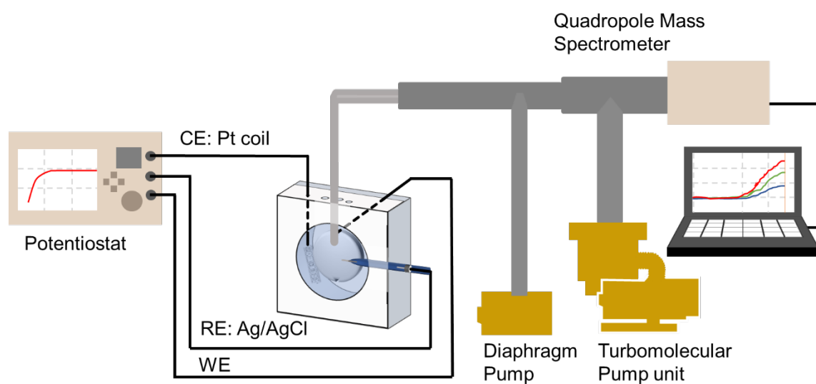
Fig. 1 | Schematic illustration of in-situ electrochemical mass spectrometry system.
