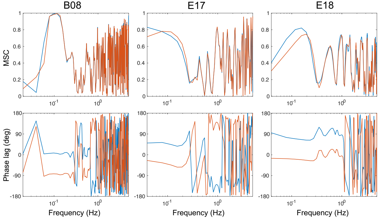
Figure S2. MSCs (top) and phase lags (bottom) at B08 (left), E17 (center), and E18 (right). Blue and orange lines represent the results estimated from the pair of acceleration and OBP and that of velocity and OBP, respectively. Note that the frequency range is the same as Figure 3(a) not 3(b). The MSCs of both acceleration and velocity at B08 are larger than 0.8 at around 0.1 Hz. On the other hand, the phase lag of acceleration is almost 0^\circ at around 0.1 Hz while the one of velocity is about 90^\circ . This result implies that OBP gauges record sea-bottom accelerations at mainly around 0.1 Hz. This relationship does not seem to be maintained at E17 and E18 due to their strong-ground motions in horizontal components (Section 4.2).
