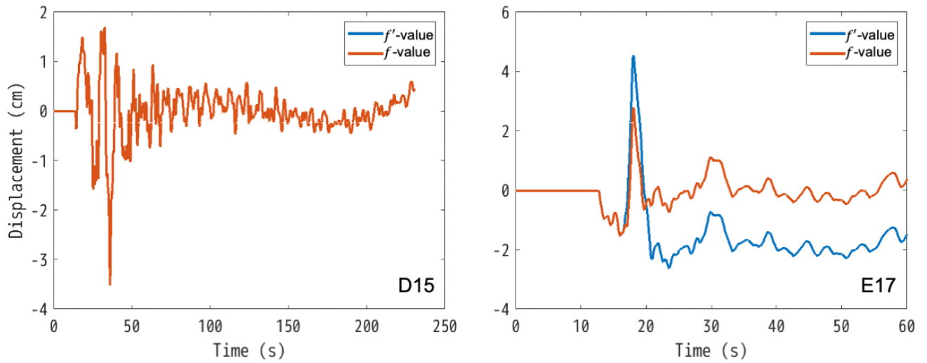
Figure S1. Comparison of the corrected displacement waveforms at stations D15 and E17 between f' -value (blue) and f -value (orange). The residual or static displacements obtained by OBP records for f' -value were 0.2 cm and -1.8 cm at D15 and E17, respectively. The residual displacement can be reproduced by f' -value better than the one with f -value at E17. Because the residual displacement at D15 was negligible, the waveforms with f - and f' -value are nearly identical to each other.
