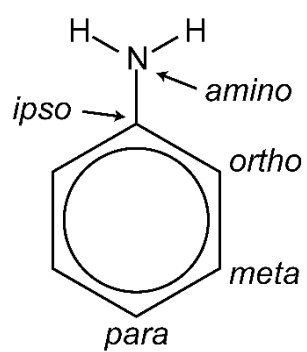
Figure 1. Five distinct protonation sites in aniline ( \text{C}_6\text{H}_5\text{NH}_2 ).
