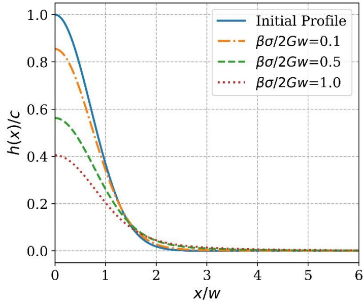
Fig. 4. The deformed shape of a Gaussian bump due to surface stress (dotted lines). The initial shape (without surface stress) is the solid blue line.
