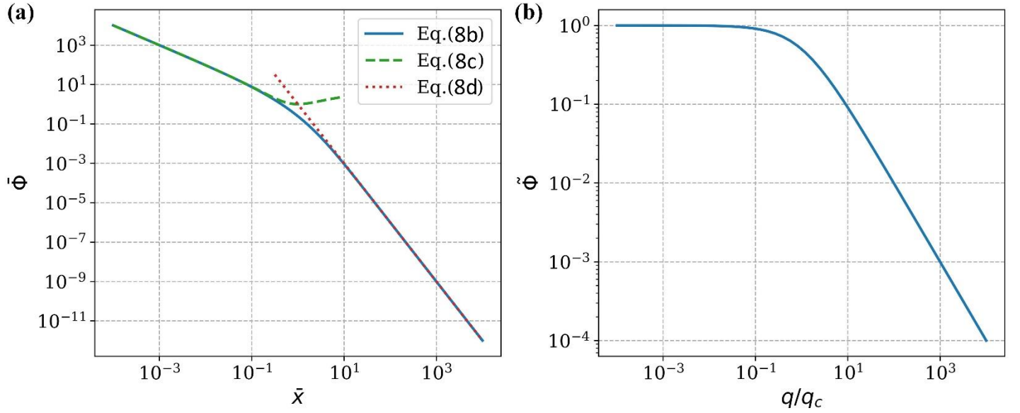
Fig. 2. (a) Normalized transfer function \bar{\phi} = 2\pi\phi/q_c^2 in real space versus normalized radial distance \bar{x} . The asymptotic behavior for small and large \bar{x} (Eq. (8c,d)) are plotted as dashed and dotted lines respectively. (b) Transfer function \tilde{\phi}(\mathbf{q}) in the Fourier space versus q/q_c .
