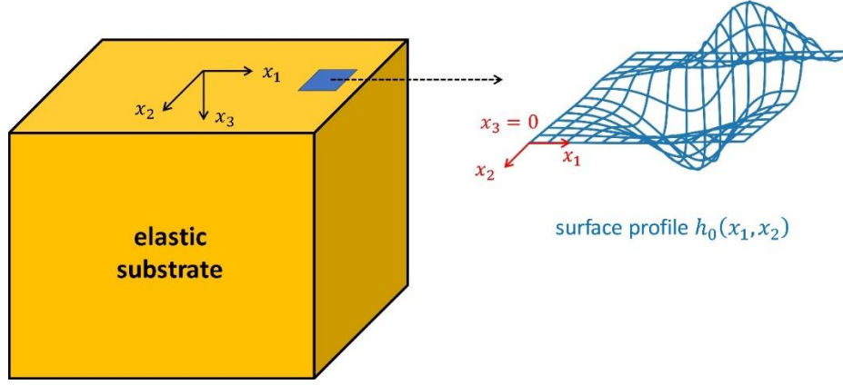
Fig. 1. Our system consists of an elastic substrate that is very large in all its dimensions compared to length scales that characterize surface undulations or structure.
