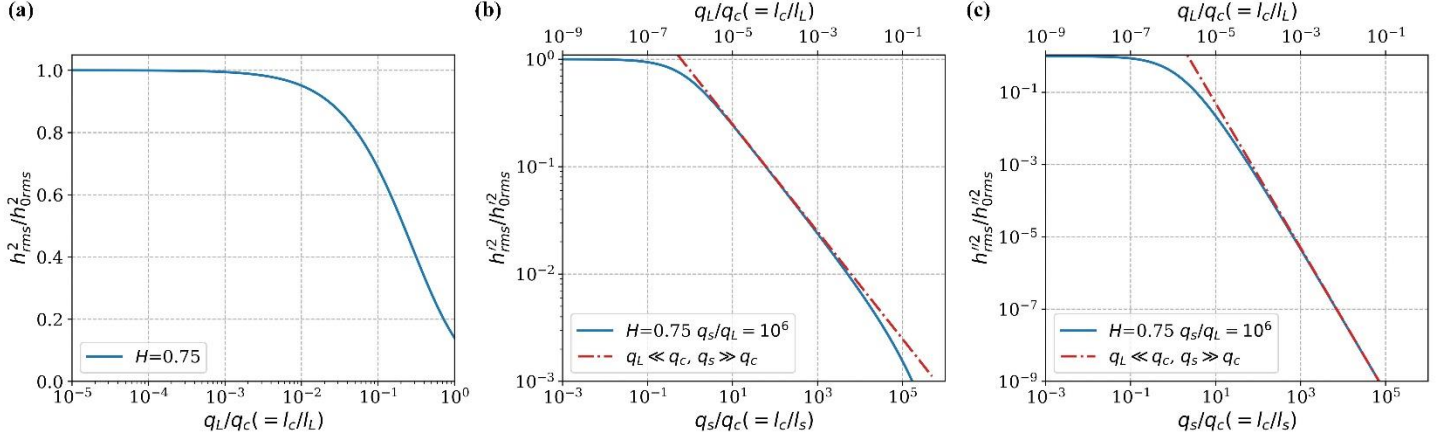
Fig. 6. (a) The ratio of RMS heights is plotted against the elastocapillary number for H = 0.75 . (b) The ratio of RMS slope is plotted against q_s / q_c for H = 0.75 and q_s / q_L = 10^6 . The red dash-dotted line is (25b). (c) The ratio of RMS curvature is plotted against the elastocapillary number for H = 0.75 and q_s / q_L = 10^6 . Blue solid is the exact solution. The red dash-dot curve is (28b).
