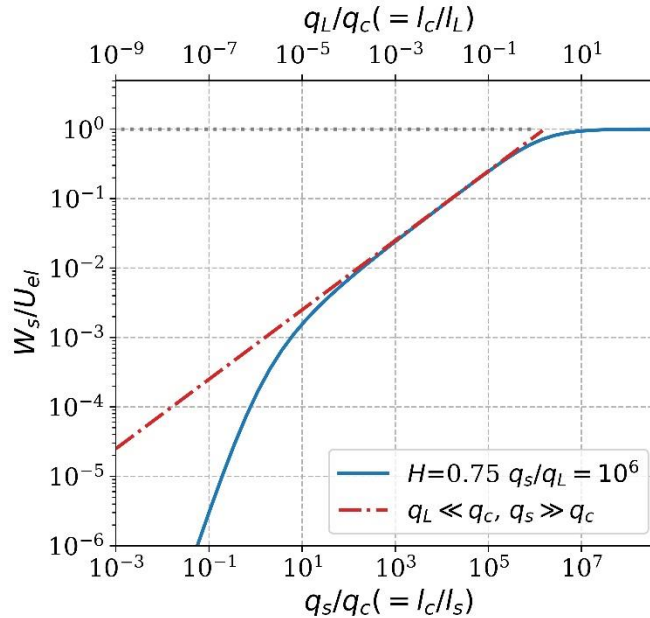
Fig. 7. Ratio of the elastic energy density due to surface tension, W_s , and the elastic energy density U_{el} needed to completely flatten the rough surface in the absence of surface stress plotted against q_s/q_c for the case of H = 0.75 and q_s/q_L = 10^6 .
