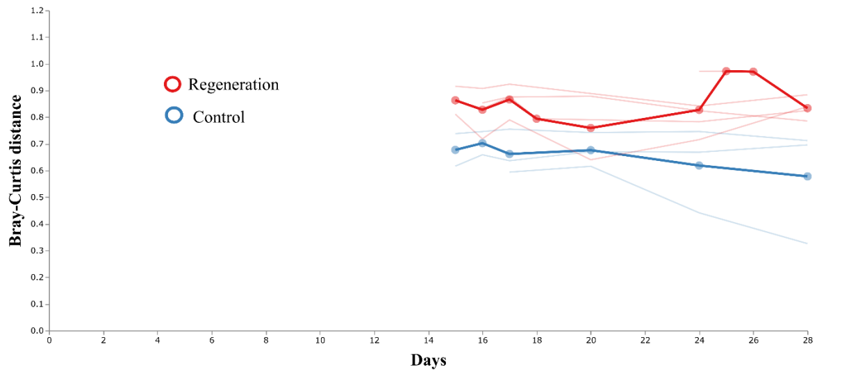
Fig. 4.8. Bray-Curtis distances of fecal microbiota from time-point zero to other time-points. Red and blue colored bold lines were mean Bray-Curtis distances from time point zero to other time points in regeneration group and control group, respectively. Pale colored lines showed each specimen.
