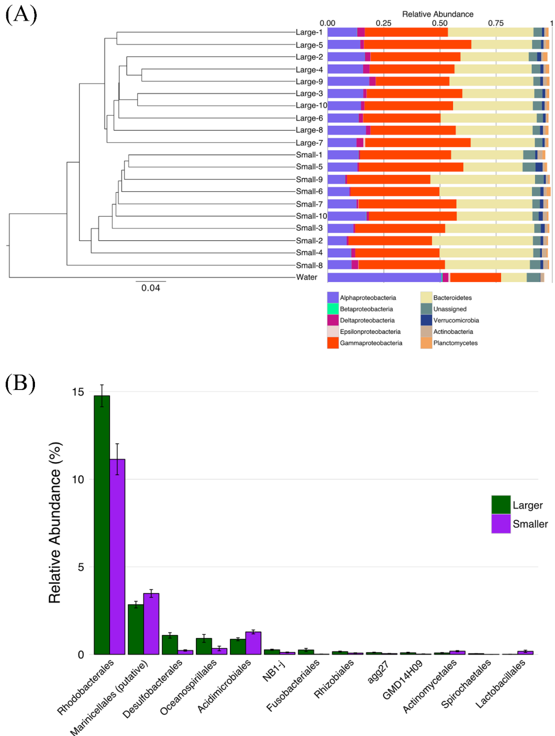
Fig. 1.2. The microbiota of larger and smaller sea cucumbers feces are different. (A) The larger and the smaller sea cucumbers clustered individually, and seawater sample differed from sea cucumber samples. (B) Ranking of the order level abundances in fecal microbiota of the larger (green) and the smaller (purple) individuals. Only significant taxa were shown in this bar plot; Rhodobacterales, Desulfobacterales and Oceanospirillales were significantly more abundant in the larger individuals, Marinicellales, Acidimicrobiales were more abundant in the smaller individuals.
