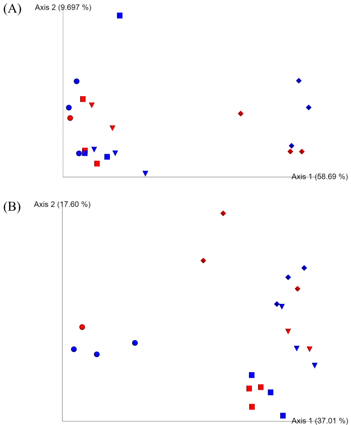
Fig. 4.5. Beta diversity analyses of eukaryotic communities in the caged mariculture experiment. Red and blue colored symbols are regeneration group and controls, respectively. Sphere-shaped samples were collected in April, and cylinders were in May, and cones were in June, and diamonds were in July. December samples were excluded due to limited number of eukaryotic reads. (A) Bray-Curtis PCoA plot. (B) Unweighted UniFrac PCoA plot.
