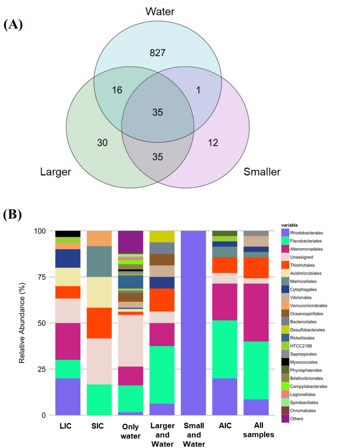
Fig. 1.4. Core fecal microbiota of cultured juvenile Apostichopus japonicus . (A) Venn diagram of core microbiota, and (B) the order level bacterial structure.
