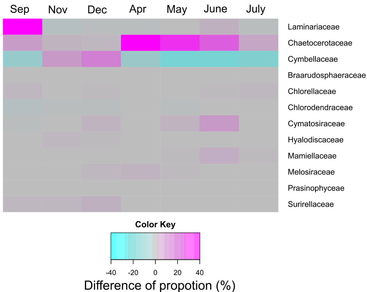
Fig. 3.3. Difference of proportion of 12 families based on LEfSe. Difference of relative abundance of 12 families identified by LEfSe between fecal and sediment samples by sampling month was shown in the heat map. Row names were families, and column names were months from September 2016 to July 2017. Magenta and cyan colors indicate families which were more abundant in feces than in sediments and more abundant in sediments than in feces, respectively.
