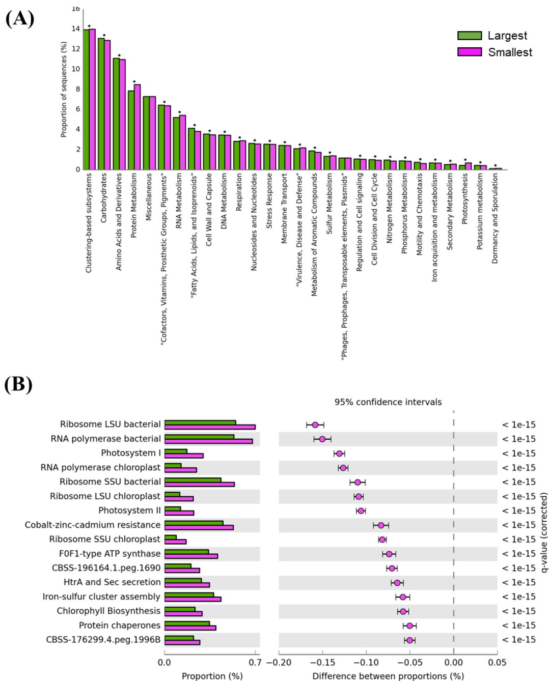
Fig. 1.6. Comparative metagenomic analyses at subsystem level 1 and 3. (A) Bar plot shows proportions of sequences for each functional feature at subsystem level 1. The largest indicated by green and the smallest indicated by purple color. Significantly different proportion of a feature between groups is indicated by an asterisk, respectively. (B) Only more abundant features in the smallest sea cucumbers are displayed. Green bars indicate the largest sea cucumber and purple indicate the smallest sea cucumber. Proportion (left side) means a possible abundance of microbes possessing each functional feature, and difference between proportions (= effect sizes) for each feature is indicated by a green dot. For this analysis, features were filtered by q value < 0.05 and effect size > 0.05 . These functions were associated with ribosome, RNA polymerase and photosystems.
