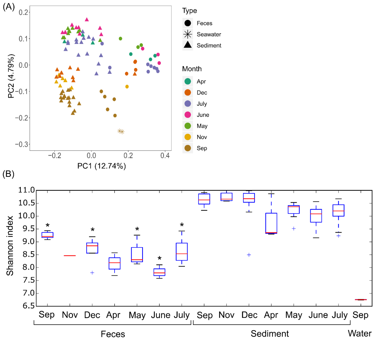
Fig. 2.4. Bacterial diversity analyses in the Menagawa site. (A) Unweighted UniFrac analysis was performed based on phylogenetic tree using 8000 of subsampled reads. The PCoA 2D plot shows fecal, sediment and seawater microbiota in the Menagawa. Different shapes of samples indicate different sample types (i.e. feces, sediment, seawater), and samples were colored by months. Significant difference of UniFrac distance was confirmed by permutational multivariate analysis of variance (PERMANOVA) (FDR-corrected p < 0.05 ). (B) Using the same number of subsampled reads, Shannon index of bacterial community diversity from sea cucumber fecal and sediment samples considering their sampling months was calculated. Asterisks show significant differences between mean Shannon indices within fecal and sediment samples in each month. Significance was evaluated based on 999 Monte Carlo permutation test with false discovery rate [false discovery rate (FDR)-corrected p < 0.05 ].
