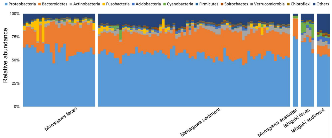
Fig. 2.3. Bacterial community structures (phylum level) of sea cucumber feces and their habitat's sediment and seawater. The Bar plot shows relative abundance of the top 10 phyla. Unassigned and under top 10 phyla were combined into others.
