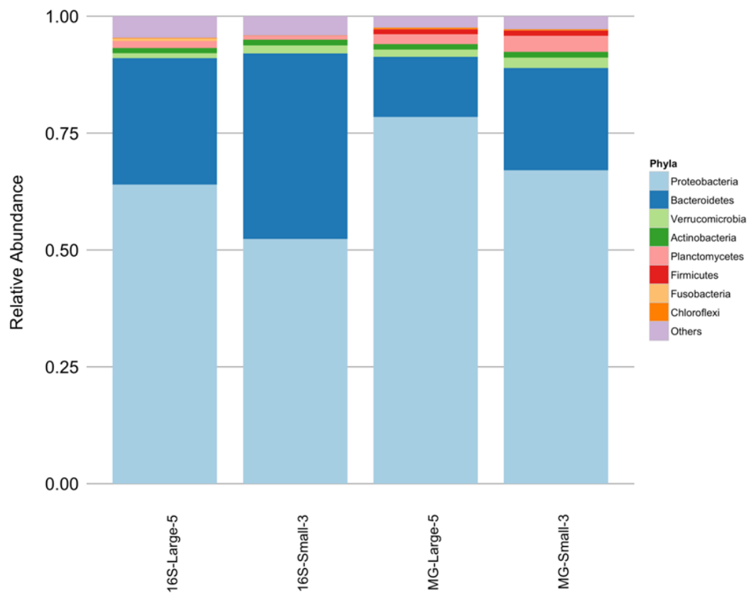
Fig. 1.5. Taxa comparison of representative fecal bacterial communities between 16S rRNA gene and shotgun metagenomic sequencing analyses. The largest and the smallest sea cucumbers were compared at phylum level. We used reference database Greengenes and GenBank for 16S rRNA gene-based analysis and metagenomic analysis, respectively.
