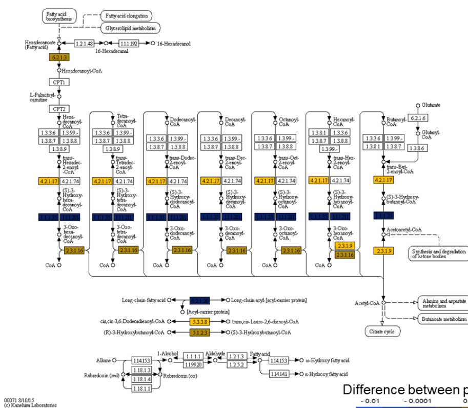
Fig. 1.8. Continued. (B) n-Phenylalkanoic acid degradation and (C) fatty acid metabolism cluster.
