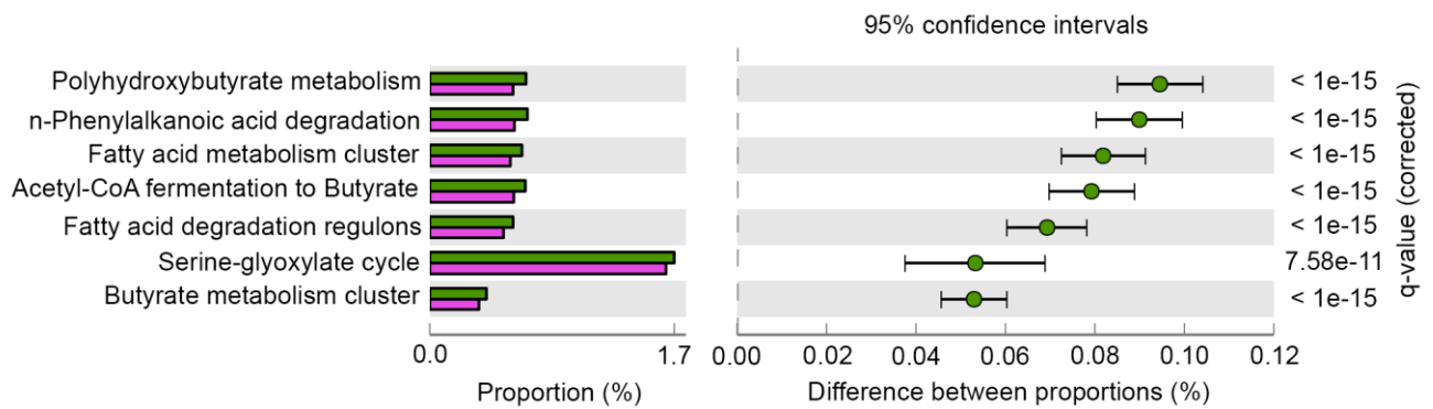
Fig. 1.7. An extended error bar plot showing more abundant features in the largest sea cucumbers. Green bars indicate the largest sea cucumber and purple indicate the smallest sea cucumber. Proportion (left side) means a possible abundance of microbes possessing each functional feature, and difference between proportions (= effect sizes) for each feature is indicated by a green dot. For this analysis, features were filtered by q value (0.05) and effect size (0.05). Relative abundances of metagenomic reads related to polyhydroxybutyrate (PHB) metabolism and butyrate metabolism were more abundant in the largest individual.
