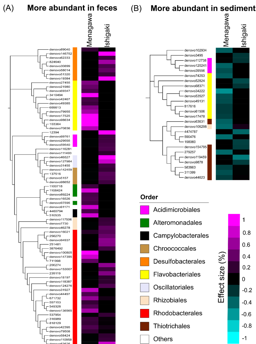
Fig. 2.7. Dendrogram-connected heatmaps of LefSe-identified OTUs of Ishigaki July and Menagawa July samples. Difference of mean proportion of each OTU between feces and sediments was calculated [= effect size (%)] using samples collected in the Ishigaki site in July and the Menagawa site in July. More vivid magenta and cyan corresponds to more abundant OTUs in feces and in sediments, respectively. Y axis were aligned by Maximum-Likelihood tree of representative reads of each OTU. Color bars show order level affiliation of each OTU. Unassigned and minor taxa (more abundant OTUs in feces or sediments than the other at one time only) were combined into others. (A) The heatmap shows OTUs which were more abundant in fecal microbiota than in sediment microbiota. (B) The heatmap shows OTUs which were more abundant in sediment microbiota than in fecal microbiota.
