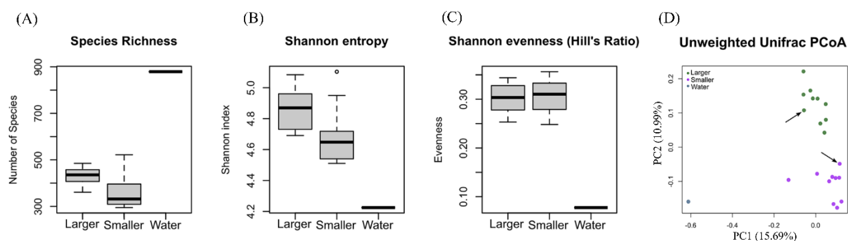
Fig. 1.3. Microbial diversity comparisons between larger and smaller Apostichopus japonicus individuals. (A) species richness, (B) Shannon index, (C) evenness, and (D) unweighted UniFrac-based 2D PCoA plot was based on all OTUs from the larger, the smaller sea cucumbers and seawater. Percent variation expected were PC1 15.69%, PC2 10.99%. Samples indicated with arrows were used for functional metagenomic analysis. The larger sea cucumbers, the smaller ones, and seawater sample are indicated in green, purple, and blue, respectively.
