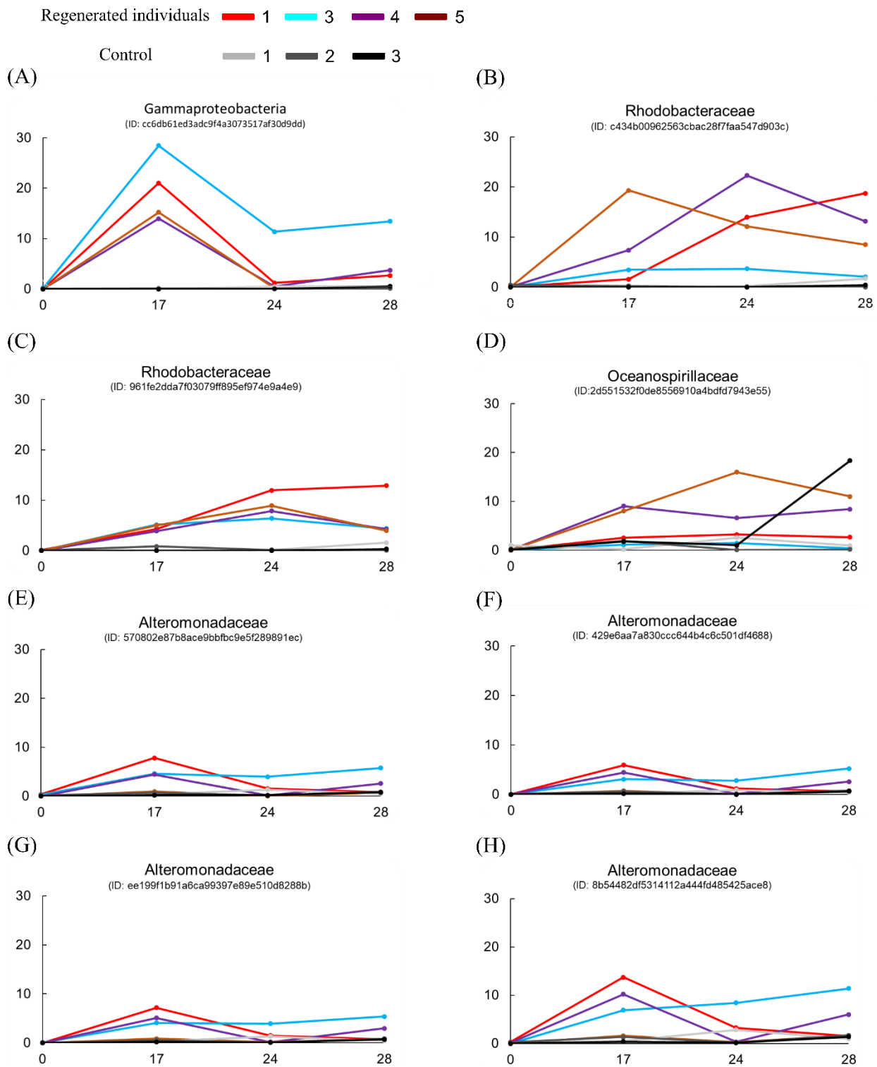
Fig. 4.10. Dynamics of relative abundance of key features based on the heatmap analysis. Eight key features were shown in (A)~(H), respectively. X axis is days, and Y axis is relative abundance (%) of each feature.
