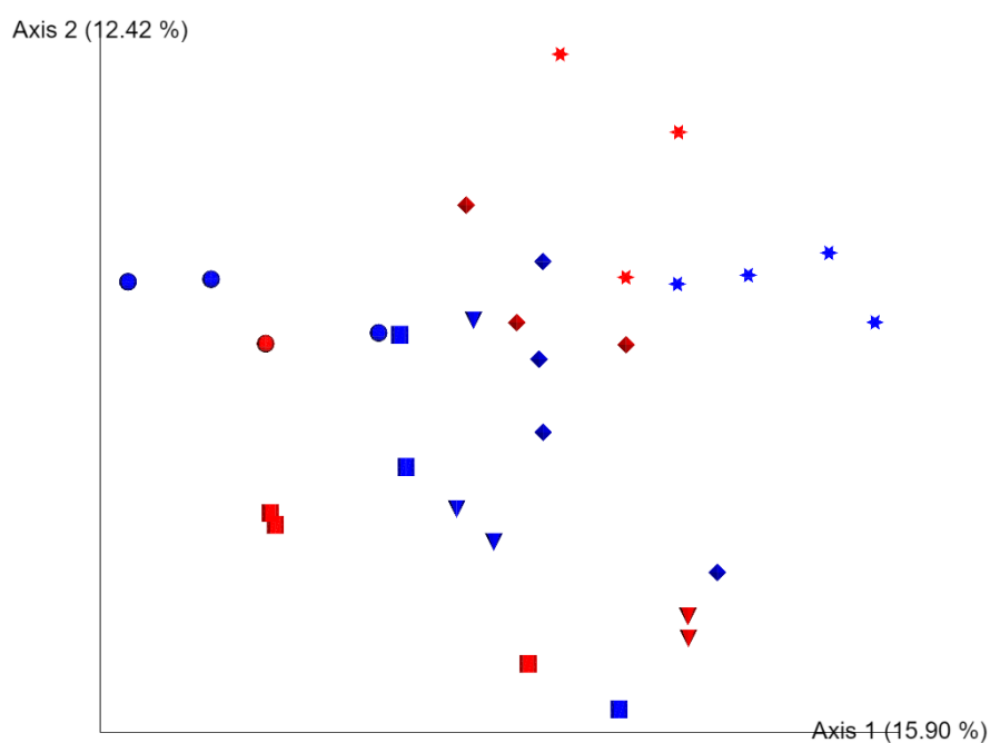
Fig. 4.4. Beta diversity analyses of the bacterial communities in the caged mariculture experiment. Red and blue colored symbols are regeneration and control groups, respectively. Star-shaped samples were collected in December, when we removed sea cucumber guts. Sphere-shaped samples were collected in April, and cylinders were in May, and cones were in June, and diamonds were in July. (A) Bray-Curtis PCoA plot. (B) Unweighted UniFrac PCoA plot.
