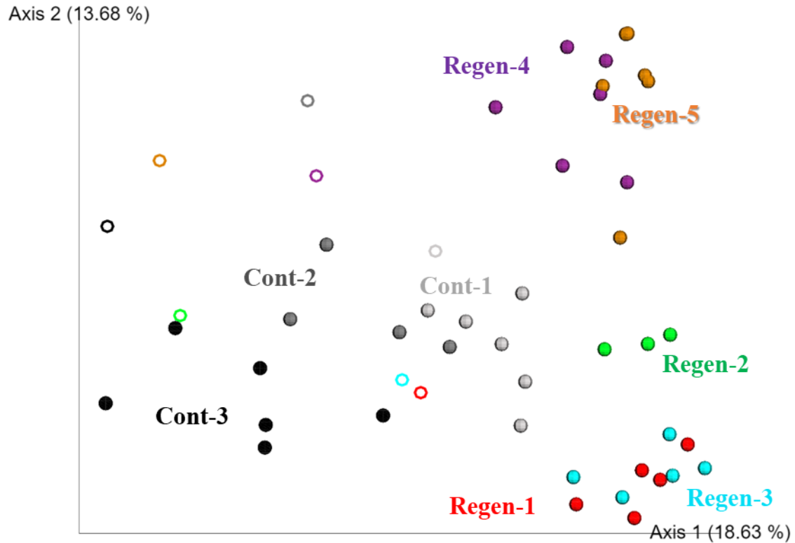
Fig. 4.6. Unweighted UniFrac distance-based 2D PCoA in the laboratory feeding experiment. Specimens in the regeneration group were indicated by “Regen-” and colored by different bright colors. Specimens in the control group were indicated by “Cont-” and in monochrome. Closed-circle samples are collected after regeneration, and open-circle samples are collected before evisceration.
