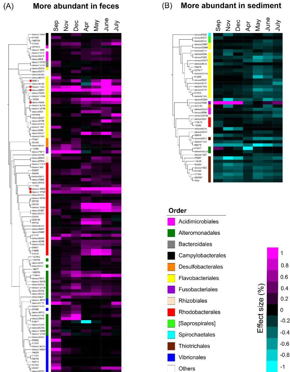
Fig. 2.5. Dendrogram-connected heatmaps of LEfSe-identified OTUs of the Menagawa site. Difference of mean relative abundance of each OTU between feces and sediments were calculated [= effect size (%)]. More vivid magenta and cyan corresponds to more abundant OTUs in feces and sediments, respectively. X axis of the heatmaps were aligned by time series of sampling. Y axis were aligned by the maximum-likelihood tree of representative reads of each OTU. Color bars show order level affiliation of each OTU. Unassigned and minor taxa (more abundant OTUs in feces or sediments than the other at one time only) were combined into others. The fecal sample in November was excluded from LEfSe analysis due to limited available samples ( N=1 ). (A) The heatmap shows OTUs which were more abundant in fecal microbiota than in sediment microbiota. Red circles indicate six representative OTUs which were more abundant in feces than in sediments in the months of September and December in 2016, and May, June and July in 2017 based on LEfSe. (B) The heatmap shows OTUs which were more abundant in sediment microbiota than in fecal microbiota.
