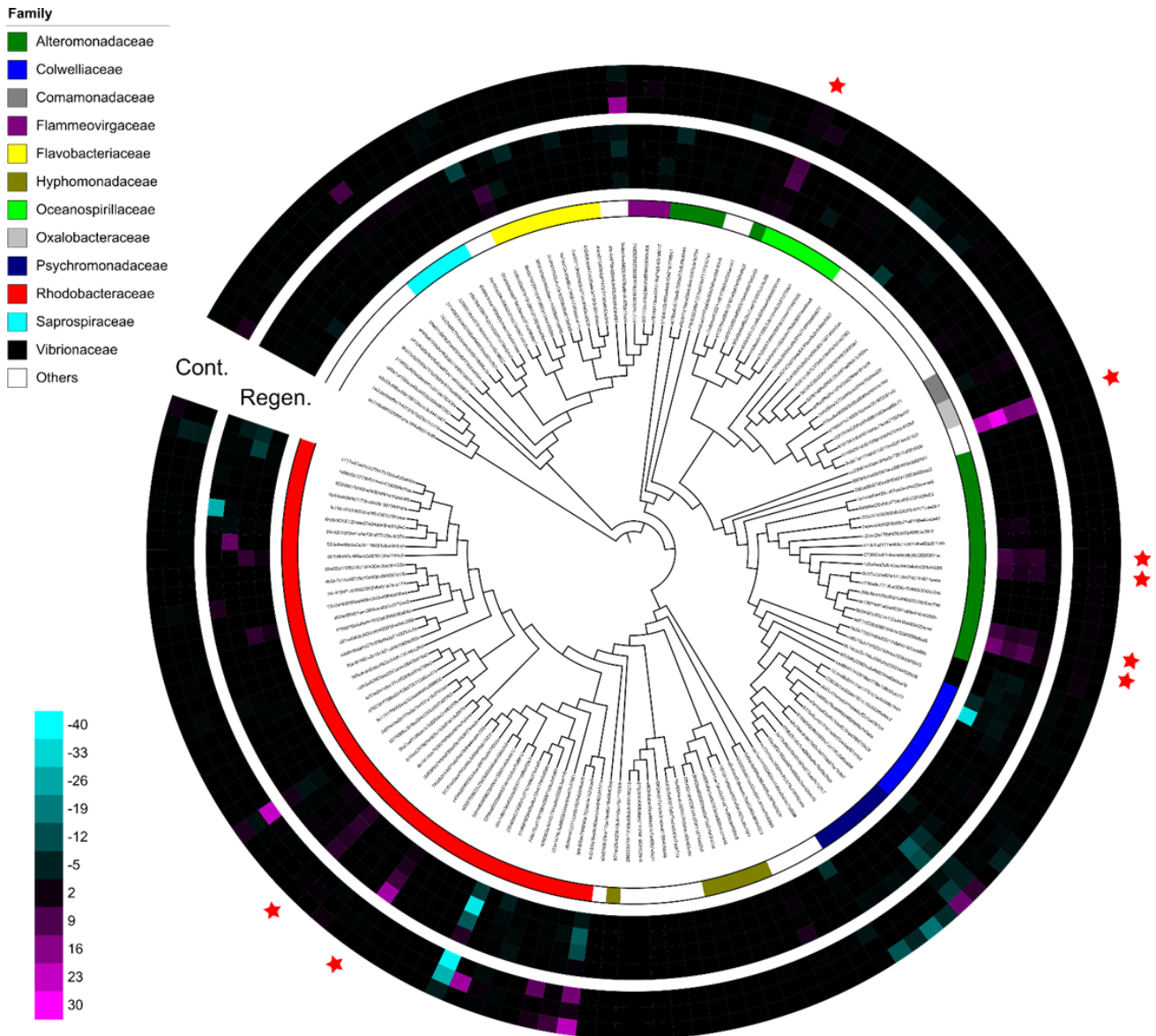
Fig. 4.9. Dendrogram-connected heatmaps features in the laboratory feeding experiment. Difference of relative abundance of features with > 500 reads between time-point zero and time-point 17 was calculated. The heat maps show four individuals from the regeneration group and three individuals from the control group, and specimen “Regen-2” was excluded due to limited number of samples. More vivid magenta corresponds to more abundant OTUs in time-point 17 than in time-point 0, and more vivid cyan corresponds to more abundant OTUs in time-point 0 than in time-point 17. Features were aligned by a maximum-likelihood tree of representative reads of each feature. The color bar shows family level affiliation of each feature. Unassigned and minor taxa were combined into others. Red stars indicate key features whose relative abundance was increased after evisceration in regeneration group.
