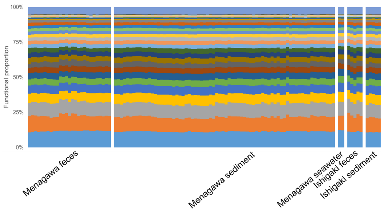
Fig. 2.9. Functional proportion of individual bacterial communities based on KEGG pathway.
