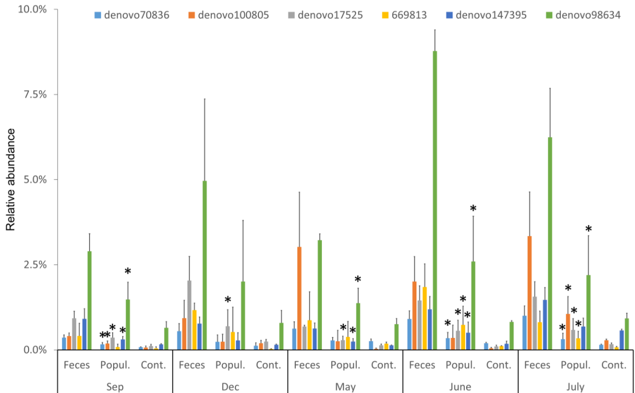
Fig. 2.8. Relative abundance of six representative OTUs by feces, host-populated sediments and controls. We selected the six representative OTUs based on LEfSe analysis in the Menagawa site. The bar plot shows mean relative abundance of the OTUs between those in feces, those in sediments where sea cucumbers were densely populated (host-populated sediments, i.e. Popul.) and those in sediments with no record of habitation (controls, i.e. Cont.). Error bars indicate standard errors. Bars marked by asterisks indicate the relative abundance of host-populated sediments which were significantly higher than those of control sediments in sampling months (Welch's t test, FDR-corrected p < 0.05 ).
