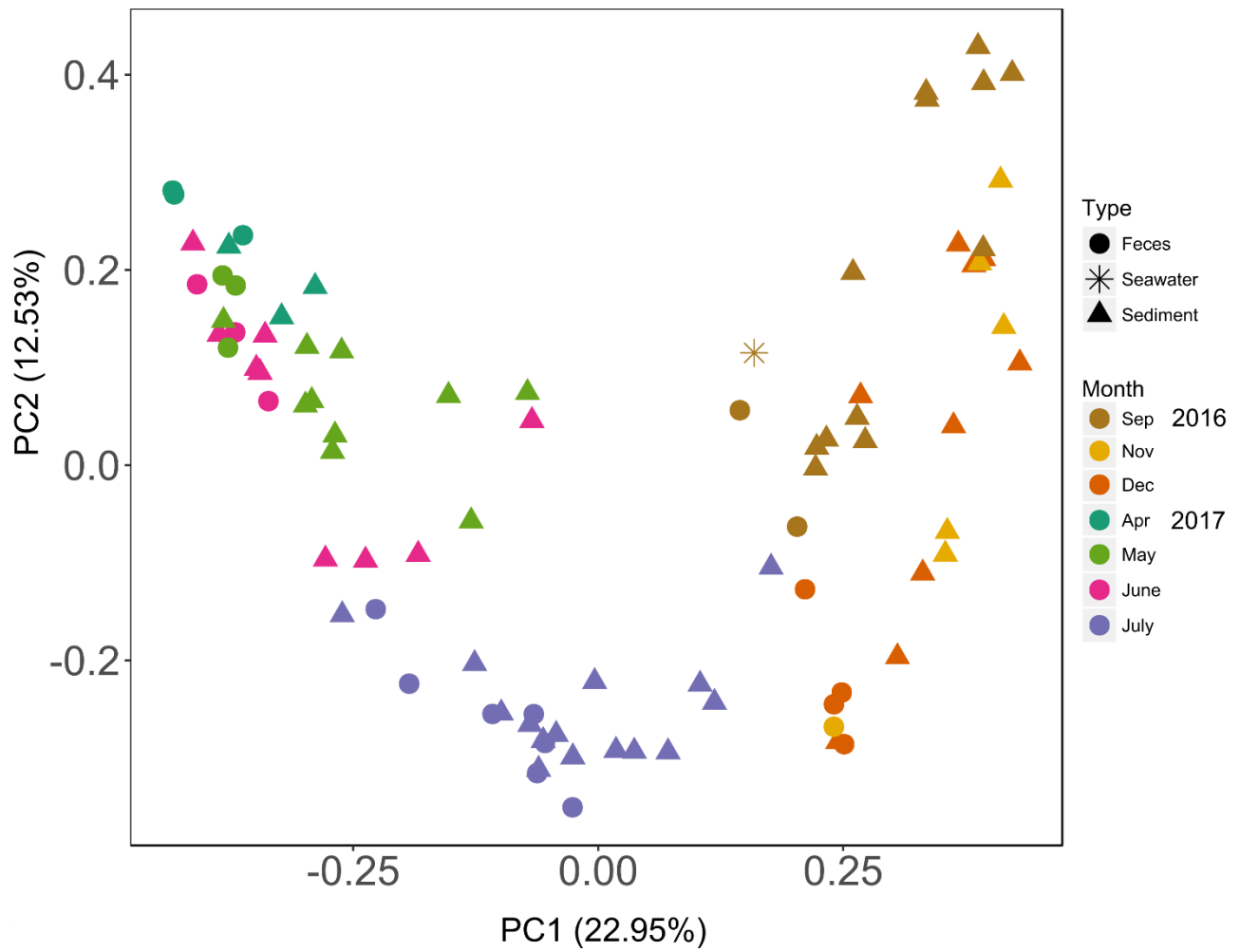
Fig. 3.1. Bray-Curtis-based 2D PCoA plot. The PCoA plot shows eukaryotic communities of sea cucumber's feces and environmental samples. Different shapes of samples indicate different sample types (i.e. feces, sediment, seawater). Samples were colored by sampling month.
