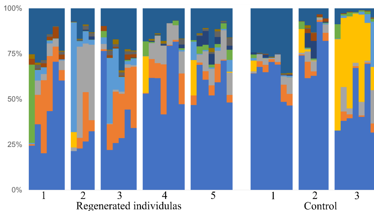
Fig. 4.7. Family Composition of bacterial communities. Top 10 families were shown in the bar plot. Minor taxa and unassigned reads were clustered into others.
