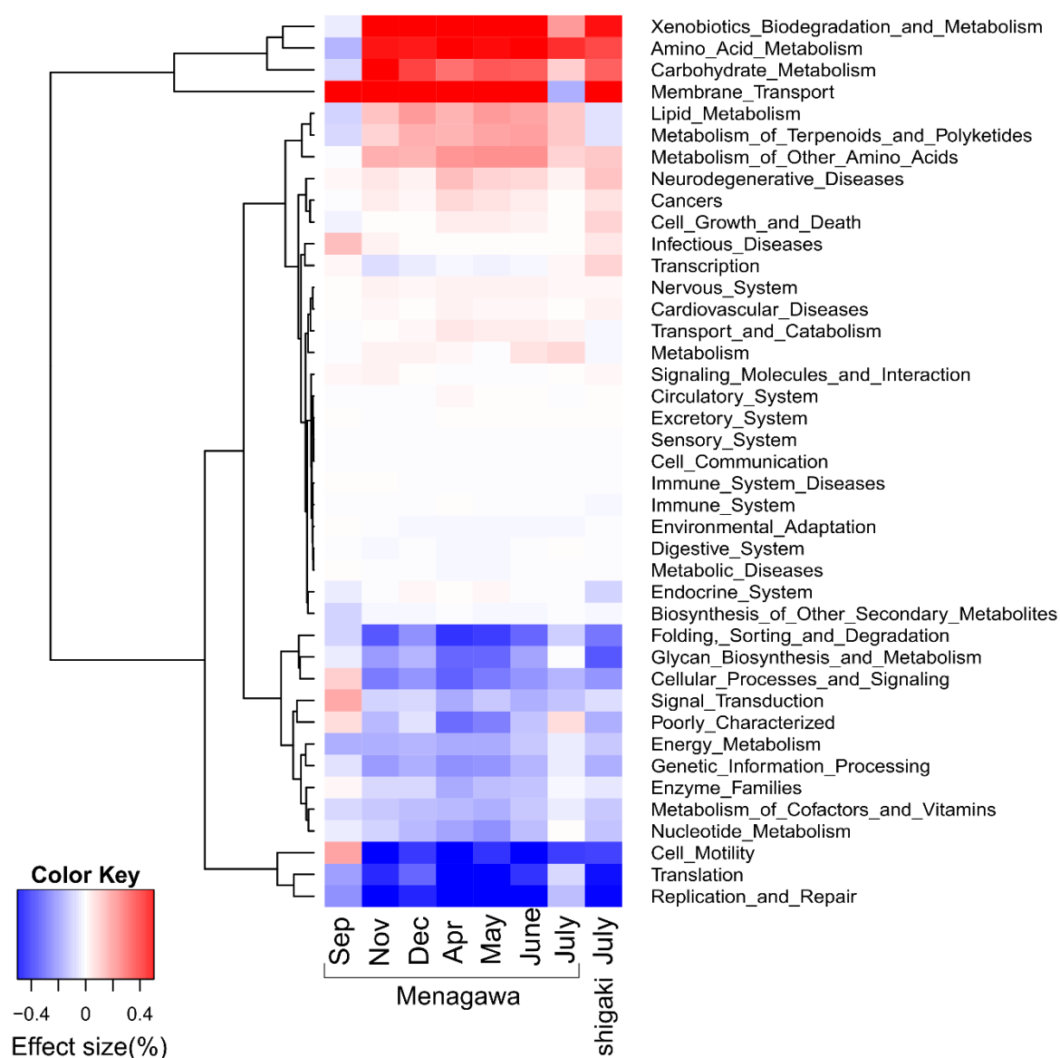
Fig. 2.10. Frequency of predicted KEGG functions. Row names indicate KEGG functions, and column names indicate sampling points. Difference of gene frequencies between feces and sediments was calculated [= effect size (%)]. Red and blue colors indicate functions which were more abundant in feces than in sediments and more abundant in sediments than in feces, respectively.
