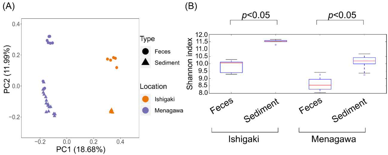
Fig. 2.6. Bacterial diversity analyses of Ishigaki July and Menagawa July samples. (A) Unweighted UniFrac analysis was performed based on phylogenetic tree using 8000 of subsampled reads. The 2D PCoA plot shows fecal and sediment microbiota in the Ishigaki site in July and in the Menagawa site in July. Circles indicate fecal samples, and triangles are sediment samples. Ishigaki samples were colored by orange, and Menagawa samples were colored by dark purple. Significant difference of UniFrac distance was confirmed by PERMANOVA (FDR-corrected p < 0.05 ). (B) Using the same number of subsampled reads, we compared bacterial community diversity (Shannon index) from sea cucumber fecal and sediment samples considering their geographical locations. Mean Shannon indices between fecal and sediment samples in each habitat were compared and evaluated based on 999 Monte Carlo permutation test with false discovery rate (FDR-corrected p < 0.05 ).
