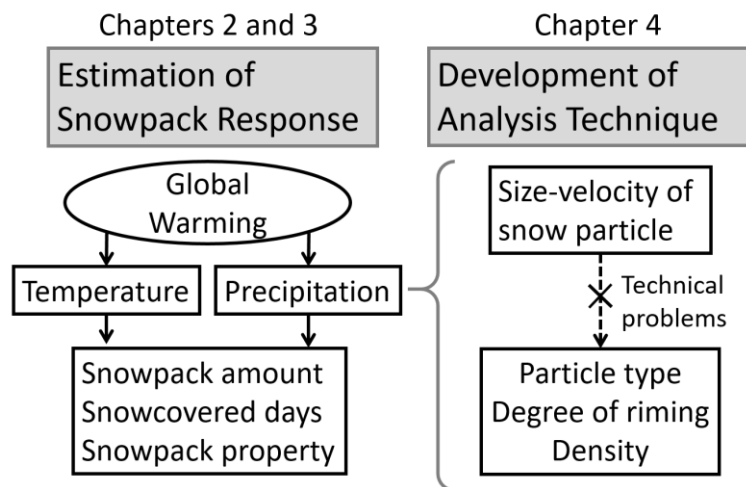
Fig. 1.2. A schematic chart describing how the global warming affects snowpack and what can be diagnosed from precipitation particles' size-velocity distribution.
