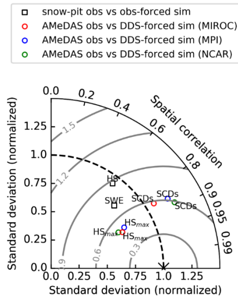
Fig. 3.8. Taylor diagram showing the comparison between simulated and observed parameters. Black squares show the comparison between the HS and SWE values obtained by snow-pit observation and those obtained by observation-forced simulation. Colored circles show comparisons between the seasonal-maximum HS ( HS_{max} ) and the snow-covered days (SCDs) obtained from AMeDAS observations and those obtained from the DDS-forced simulation in the present climate. Red, blue, and green denote the boundary conditions of MIROC, MPI, and NCAR, respectively. The standard deviations and the root mean square errors (RMSEs) of the simulations are normalized by the standard deviations of the observations. Concentric gray lines centered on the reference point (indicated by a cross mark) show RMSE.
