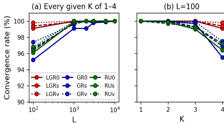
Fig. 4.2. (a) The convergence rate as a function of sample size L for every number of PDF elements K from 1 to 4 and (b) the convergence rate as a function of K in experiments with L = 100 . The line color and type are as per the legend inside of panel (a)
