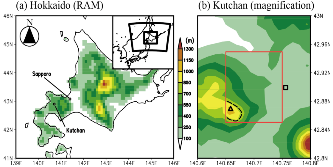
Fig. 2.2. (a) Surface height above the sea level given to the regional atmospheric model (RAM) and the location of Hokkaido in the upper right and (b) realistic topography with about 1-km resolution. Outer and inner black solid line in a window of (a) shows RAM's domain calculated and a domain of (a), respectively. The locations of top of Mt. Annupuri (the top; 1,300 m a.s.l.) and AMeDAS station (the base; 173 m a.s.l.) are respectively indicated with an open triangle and square in (b). Black dashed line in (b) shows an 800 m level of height corresponding to the hillside of the mountain slope. Red rectangle in (b) shows the RAM's grid cell of which meteorological data are imposed to the SNOWPACK model. The color-scale is shown between the panels.
