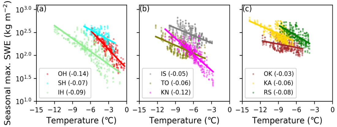
Fig. 3.10. Scatterplots of the 10-year mean of seasonal-maximum SWE versus the 10-year mean of air temperature in DJF under the present climate for all the DDS grid points in the (a) OH, SH, and IH sub-regions, (b) IS, TO, and KN sub-regions, and (c) OK, KA, and RS sub-regions. Colors as in Fig. 3.1a/Table 3.1. The best-fitting line is superimposed for each dataset, with its slope [(1/Q)(dQ/dT)] in Eq. (3.2) given in the legend.
