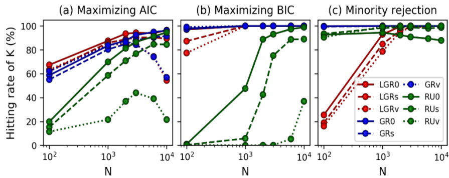
Fig. 4.5. Hitting rate of K estimated (a) by maximizing Akaike Information Criterion (AIC), (b) by maximizing Bayesian Information Criterion (BIC), and (c) by minority rejection method.
