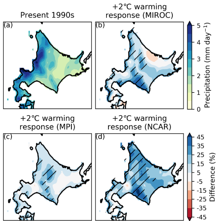
Fig. 3.4. (a) Bias-corrected 10-year mean daily precipitation in DJF in the present climate and its difference with the precipitation predicted for the +2°C global warming climate scenario using the DDS of the boundary conditions of (b) MIROC, (c) MPI, and (d) NCAR. The hatched areas denote statistical significance at the 5% level.
