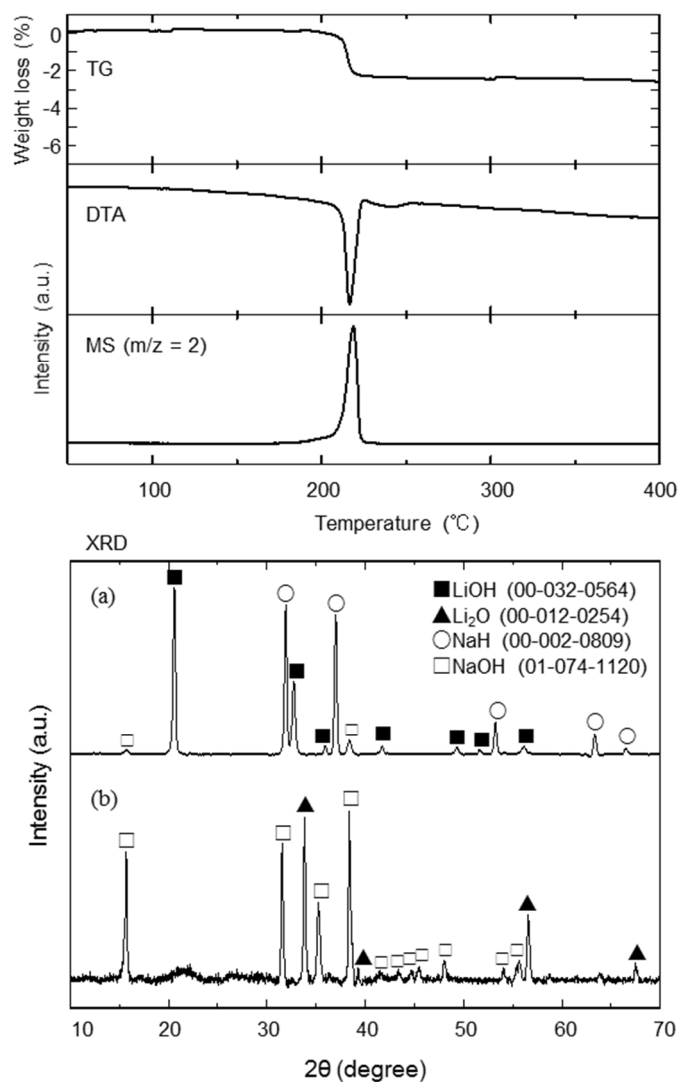
FIGURE 2 TG-DTA-MS and XRD profiles of NaH + LiOH with 1 : 2 molar ratio, (a): after milling and (b) after heating to 400 ^{\circ}\text{C} .
