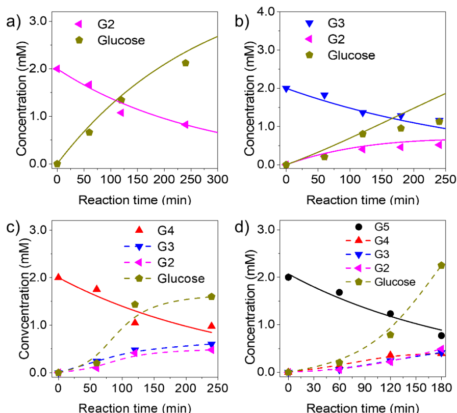
Figure 3.5. Time dependent conversion of cello-oligosaccharides and evolution of products in the presence of H-beta. Reaction conditions: 1 \mu mol cello-oligosaccharides (G2-G5), 5 mg H-beta, 0.5 mL H_2O , 0.5 MPa Ar, 413 K. a) G2, b) G3, c) G4, d) G5.
