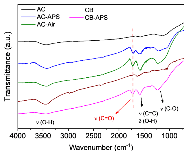
Figure 4.4. FTIR spectra of various carbon catalysts.
