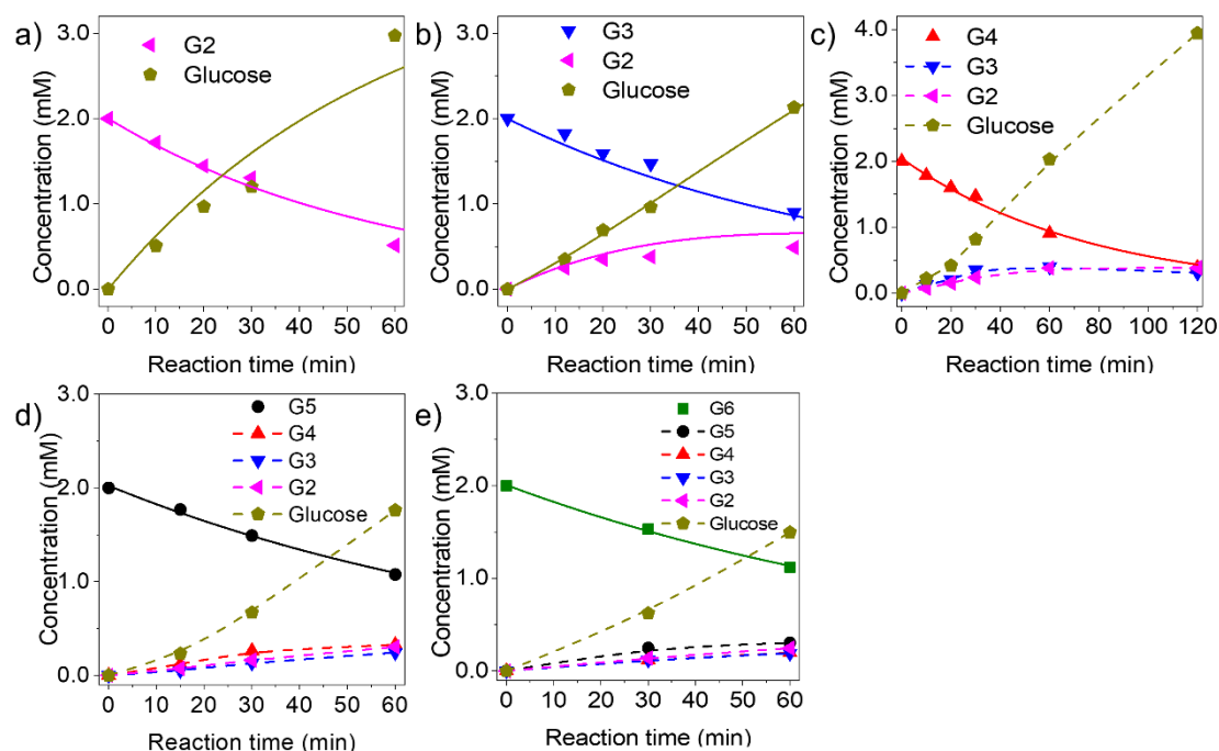
Figure 3.4. Time dependent conversion of cello-oligosaccharides and evolution of products in the presence of Amberlyst 70. Reaction conditions: 1 \mu\text{mol} cello-oligosaccharides (G2-G6), 5 mg Amberlyst 70, 0.5 mL \text{H}_2\text{O} , 0.5 MPa Ar, 413 K. a) G2, b) G3, c) G4, d) G5, e) G6.
