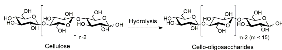
Figure 1.5. Partial hydrolysis of cellulose to water-soluble cello-oligosaccharides.
