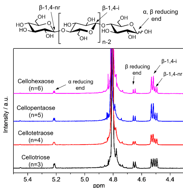
Figure 2.13. ^1\text{H} NMR spectra of the anomeric region of individual cello-oligosaccharides in \text{D}_2\text{O} .
