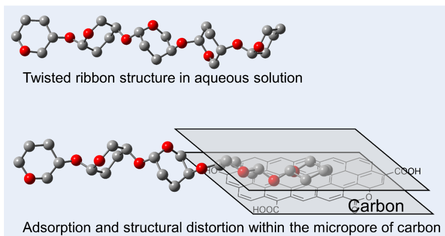
Figure 3.12. Illustration showing the twisted ribbon structure of cellopentaose in water and the proposed structural change during the adsorption on carbon surface. For clarity the hydroxyl groups are not shown and only the pyranose rings are depicted linked by \beta -1,4-glycosidic bond.
