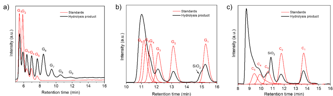
Figure 2.4. HPLC chromatogram of hydrolysis products and \beta -1,4 linked cello-oligosaccharide standards. a) Column: Amino NH 2P-40 3E; b) Column: Sugar SH-1011; c) Column: Phenomenex Rezex RPM-Monosaccharide Pb++. Reaction conditions: 0.175 g MMC (S/C = 6.5), 40 min, 0.75 \text{ mL min}^{-1} water, 1 h mix milling.
