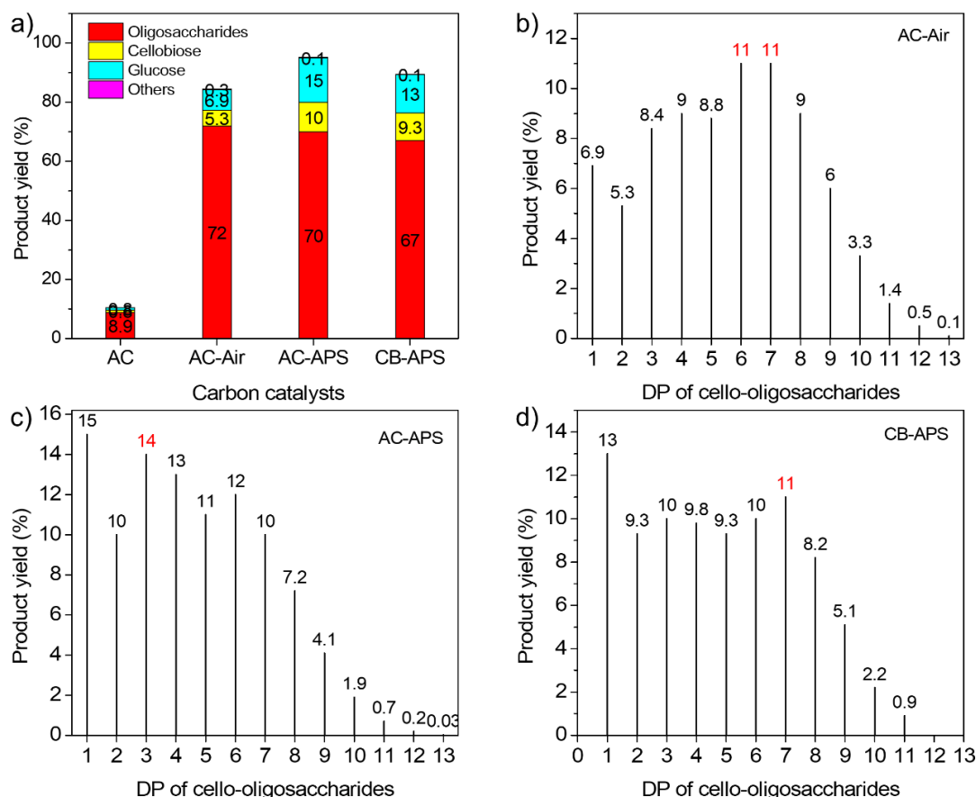
Figure 4.9. Total yield of products determined by HPLC analysis after cellulose hydrolysis by using different catalysts a). Products distribution measured by MALDI TOF MS over AC-Air b), AC-APS c), and CB-APS d). Reaction condition: 0.175 g MMC, 473 K, distilled water (0.75 mL min -1 ), SV 70 h -1 .
