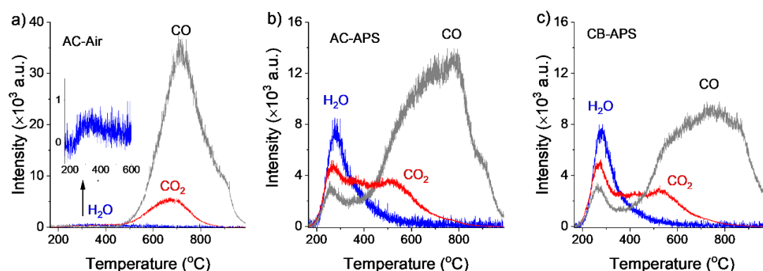
Figure 4.6. TPD mass spectra of carbon catalysts (50 mg), a) AC-Air, b) AC-APS, c) CB-APS.
