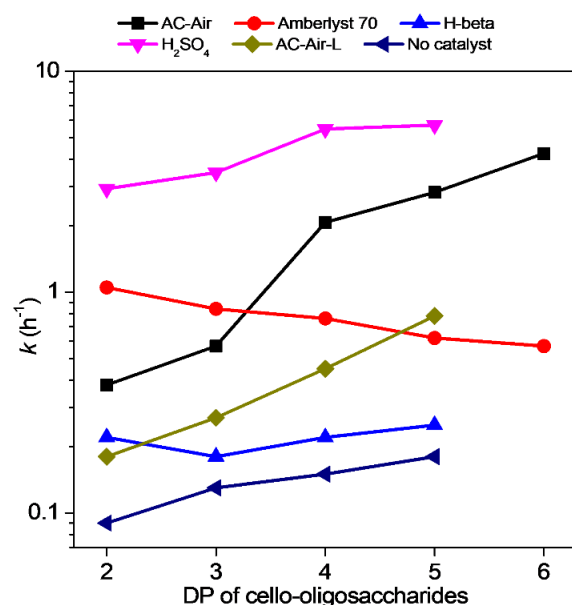
Figure 3.3. Comparison of change in rate constant for hydrolysis of cello-oligosaccharides in the presence of various acid catalysts. Reaction conditions: 1 \mu mol cello-oligosaccharides (G2-G6), 5 mg solid catalyst or 6.4 \mu mol H 2 SO 4 , 0.5 mL H 2 O, 0.5 MPa Ar, 413 K.
