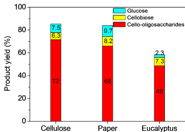
Figure 2.9. Product yields for real biomass hydrolysis. Reaction conditions: 0.175 g mix-milled substrate (S/C = 6.5), 473 K, 40 min, 0.75 mL min -1 water, 1 h mix milling.
