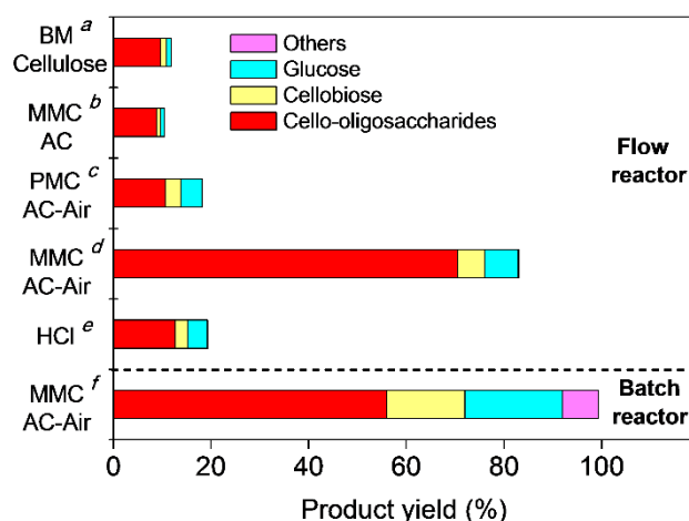
Figure 2.6. Yield of products after hydrolysis of cellulose. Reaction conditions for flow reactor: 453 K, 40 min, 0.75 mL min -1 distilled water. a) 0.150 g ball milled cellulose. b) 0.175 g cellulose mix-milled with AC (substrate to catalyst ratio S/C= 6.5). c) 0.175 g cellulose physically mixed with AC-Air (S/C = 6.5). d) 0.175 g cellulose mix-milled with AC-Air (S/C = 6.5). e) 0.150 g ball milled cellulose, 0.012 wt. % HCl aqueous solution instead of water. f) Reaction conditions for batch reactor: 0.374 g cellulose mix milled with AC-Air (S/C = 6.5), 40 mL distilled water, 453 K, 20 min.
