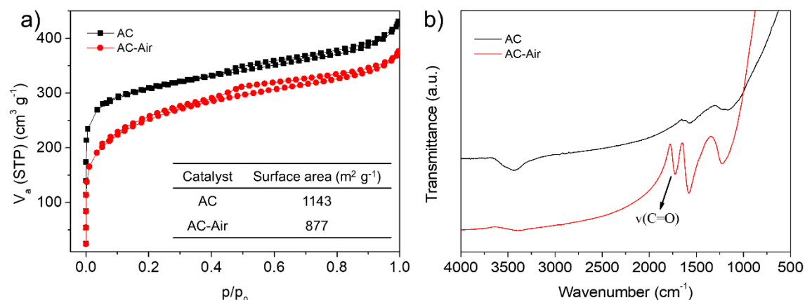
Figure 2.3. Characterization of AC and AC-Air, (a) N 2 adsorption isotherms, (b) FTIR spectra.
