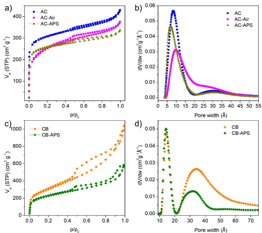
Figure 4.3. a) N 2 adsorption isotherms of parent and modified carbon AC materials, b) pore size distribution of parent and modified carbon AC materials, c) N 2 adsorption isotherms of parent and modified carbon CB materials, d) pore size distribution of parent and modified carbon CB materials.
