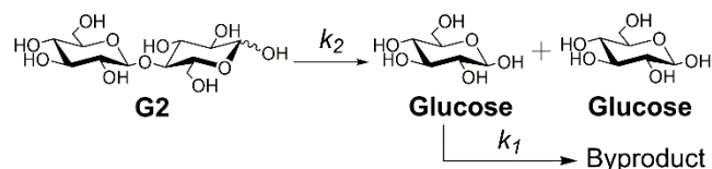
Scheme 3.1. Reaction pathway during hydrolysis of cellobiose.
