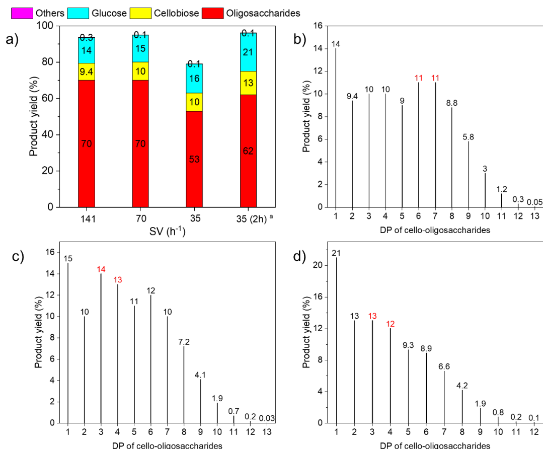
Figure 4.10. a) Cellulose hydrolysis HPLC results over AC-APS with different SV, b) Products distribution under SV of 141 h -1 , c) 70 h -1 , d) 35 h -1 . a Hydrolysis of cellulose was performed for 2 h. Reaction condition: 0.175 g MMC-AC-APS, 473 K, distilled water (0.75 mL min -1 ).
