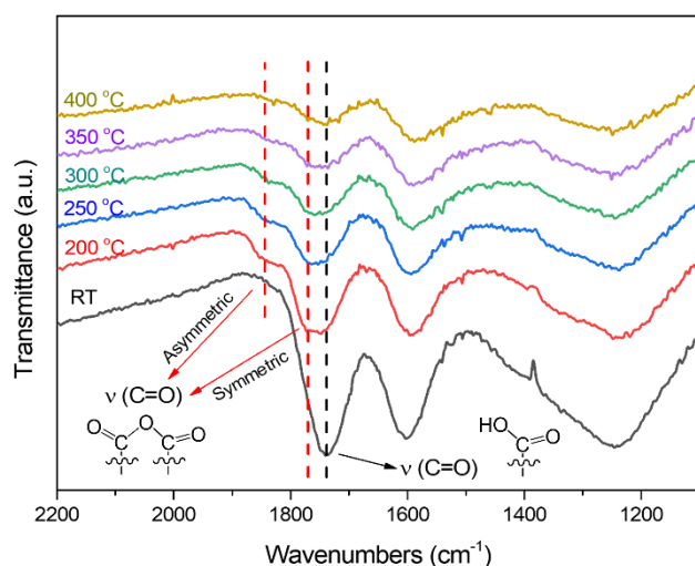
Figure 4.8. DRIFTS spectroscopy of AC-APS catalyst.
