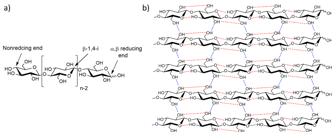
Figure 1.1. a) Elementary structure of a cellulose chain. b) Illustration showing hydrogen bonding in the extended cellulose structure.
