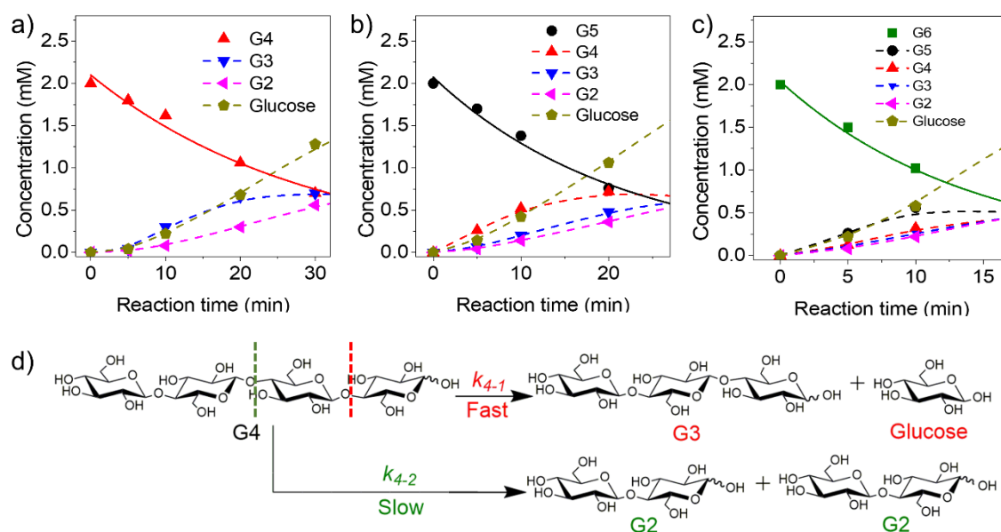
Figure 3.9. Close-up of reaction profiles shown in Figure 3.2 to illustrate the evolution of products from a) G4, b) G5, c) G6 over AC-Air catalyst. d) Scheme showing the pathway for hydrolysis of either the terminal glycosidic linkages or the internal glycosidic linkage in G4.
