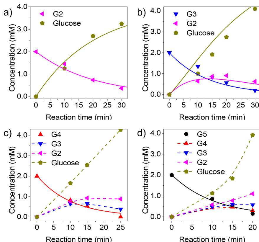
Figure 3.6. Time dependent conversion of cello-oligosaccharides and evolution of products in the presence of \text{H}_2\text{SO}_4 . Reaction conditions: 1 \mu\text{mol} cello-oligosaccharides (G2-G5), 6.4 \mu\text{mol} \text{H}_2\text{SO}_4 , 0.5 mL \text{H}_2\text{O} , 0.5 MPa Ar, 413 K. a) G2, b) G3, c) G4, d) G5.
