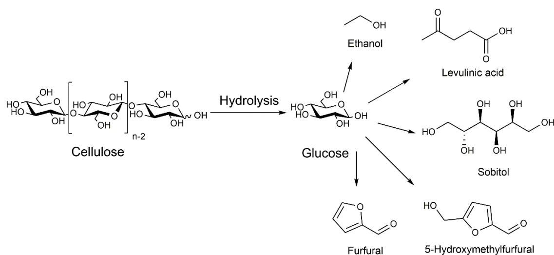
Figure 1.2. Hydrolysis of cellulose to glucose and its subsequent conversion of value-added chemicals.
