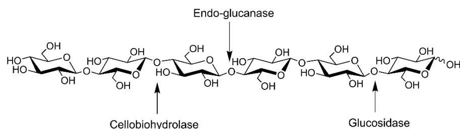
Figure 1.6. Scheme showing glycosidic bonds targeted by different enzymes during cellulose hydrolysis.
