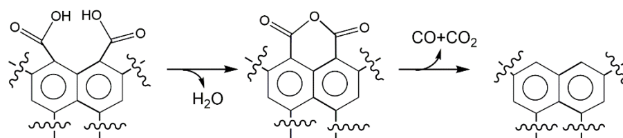
Figure 4.7. Decomposition process of two adjacent carboxylic acid on carbon catalyst during the thermal treatment.
