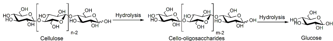
Figure 2.1. Cello-oligosaccharides are formed as intermediates in cellulose hydrolysis.
