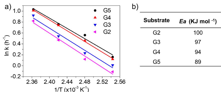
Figure 3.11. Arrhenius plot a) of cello-oligosaccharides hydrolysis on H 2 SO 4 and the calculated activation energy b).
