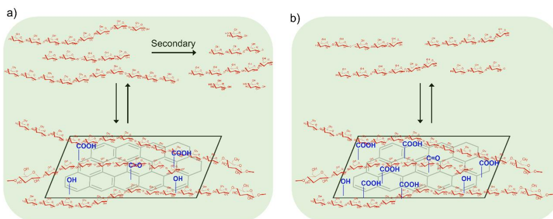
Figure 4.1. Scheme showing influence of surface acid site density on the surface of carbon catalyst over cello-oligosaccharide product distribution. a) Low density of acid sites leads to the formation of large oligosaccharides, which undergo secondary hydrolysis. b) High density of acid sites directly produces small cello-oligosaccharides and their secondary hydrolysis can be avoided.
