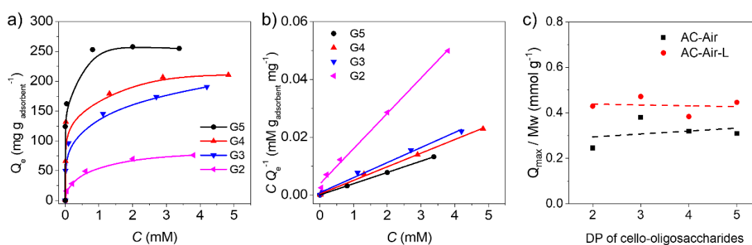
Figure 3.7. Adsorption of cello-oligosaccharides (G2-G5) on AC-Air: a) Adsorption isotherms, b) Langmuir plot derived from equation (3. 13). c) Plot showing maximum molar concentration of cello-oligosaccharides over AC-Air and AC-Air-L at saturation condition.
