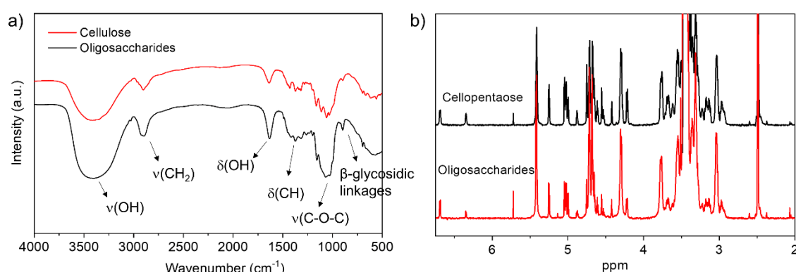
Figure 2.12. Characterization of precipitated oligosaccharides, a) FTIR spectra, b) ^1\text{H} NMR spectra in \text{DMSO-d}_6 .
