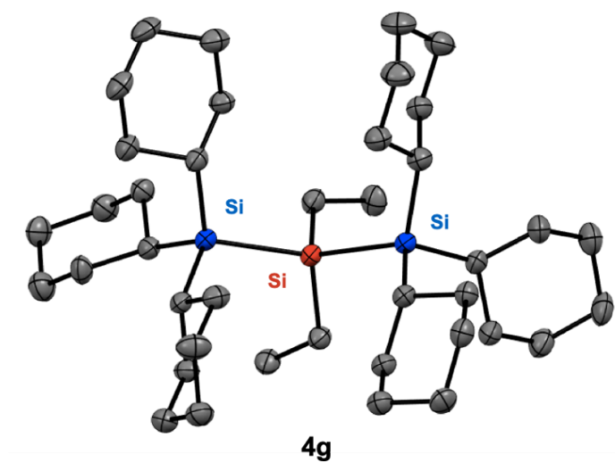
Figure 2. Crystal Structure of 4g with Thermal Ellipsoids at 50% Probability. Hydrogen atoms are omitted for clarity. Color Code: Grey: Carbon; Blue: Silicon derived from a silylborane; Red: Silicon derived from a silyl electrophile.
