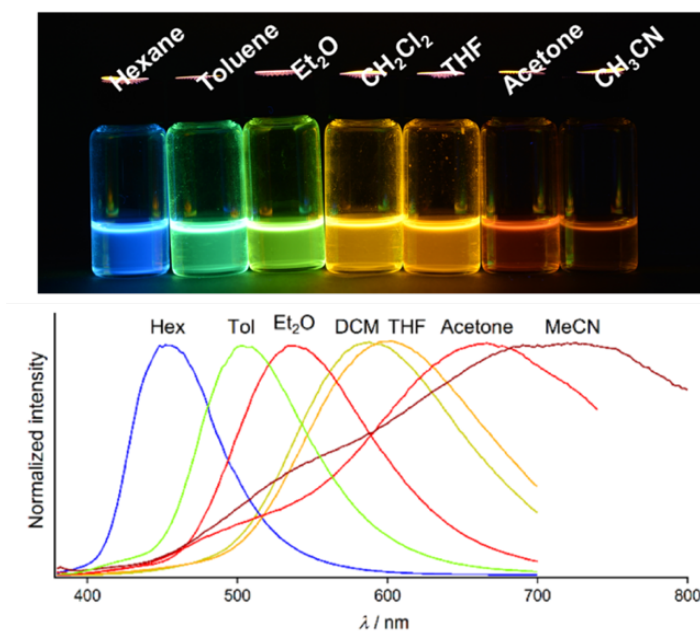
Figure 2. Photograph and Emission Spectra of 3i in Various Solvents under Irradiation from UV light ( \lambda_{\text{ex}} = 365 nm; 10 \mu\text{M} ).
