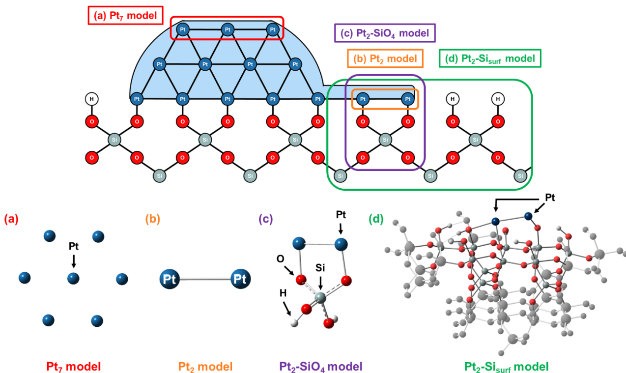
Figure 1. Computational models of the activity of the Pt/MCM-41 catalyst. (a) \text{Pt}_7 model, (b) \text{Pt}_2 model, (c) \text{Pt}_2\text{-SiO}_4 model, and (d) \text{Pt}_2\text{-Si}_{\text{surf}} model. The atomic coordinates of the gray-colored atoms are fixed during the structure optimization.
