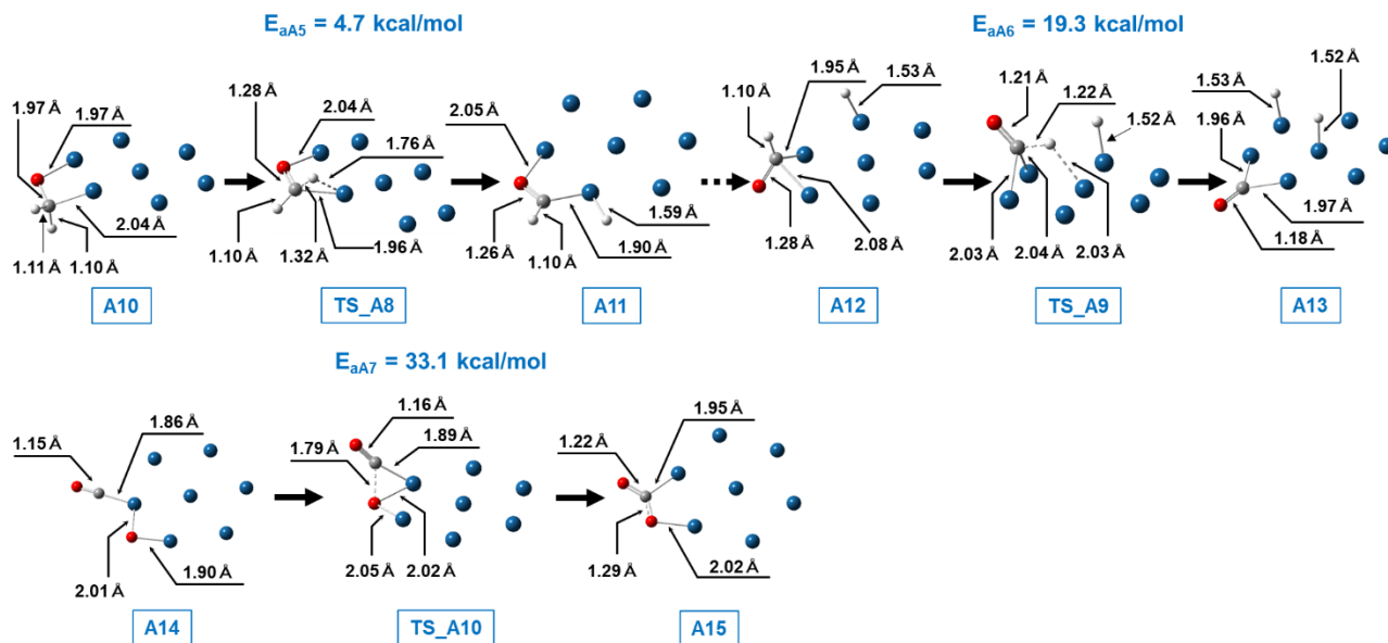
Figure 15. Optimized structures of a reactant, intermediates, transition states and a product of CO 2 generation from HCHO on the edge area of the Pt 7 model. White ball: hydrogen, gray ball: carbon, red ball: oxygen, blue ball: platinum
