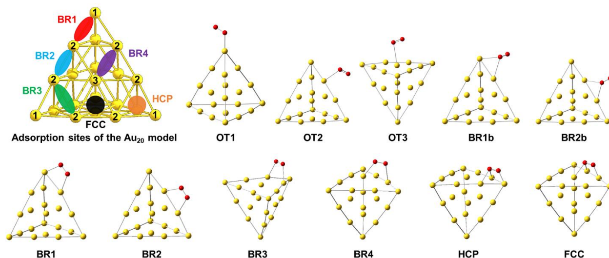
Figure 10. Adsorption sites of the \text{Au}_{20} model (numbers on each Au atom represent OT1 site, OT2 site and OT3 site, respectively), and examples of adsorption structures of \text{O}_2 on each adsorption site. Yellow ball: gold, red ball: oxygen.
