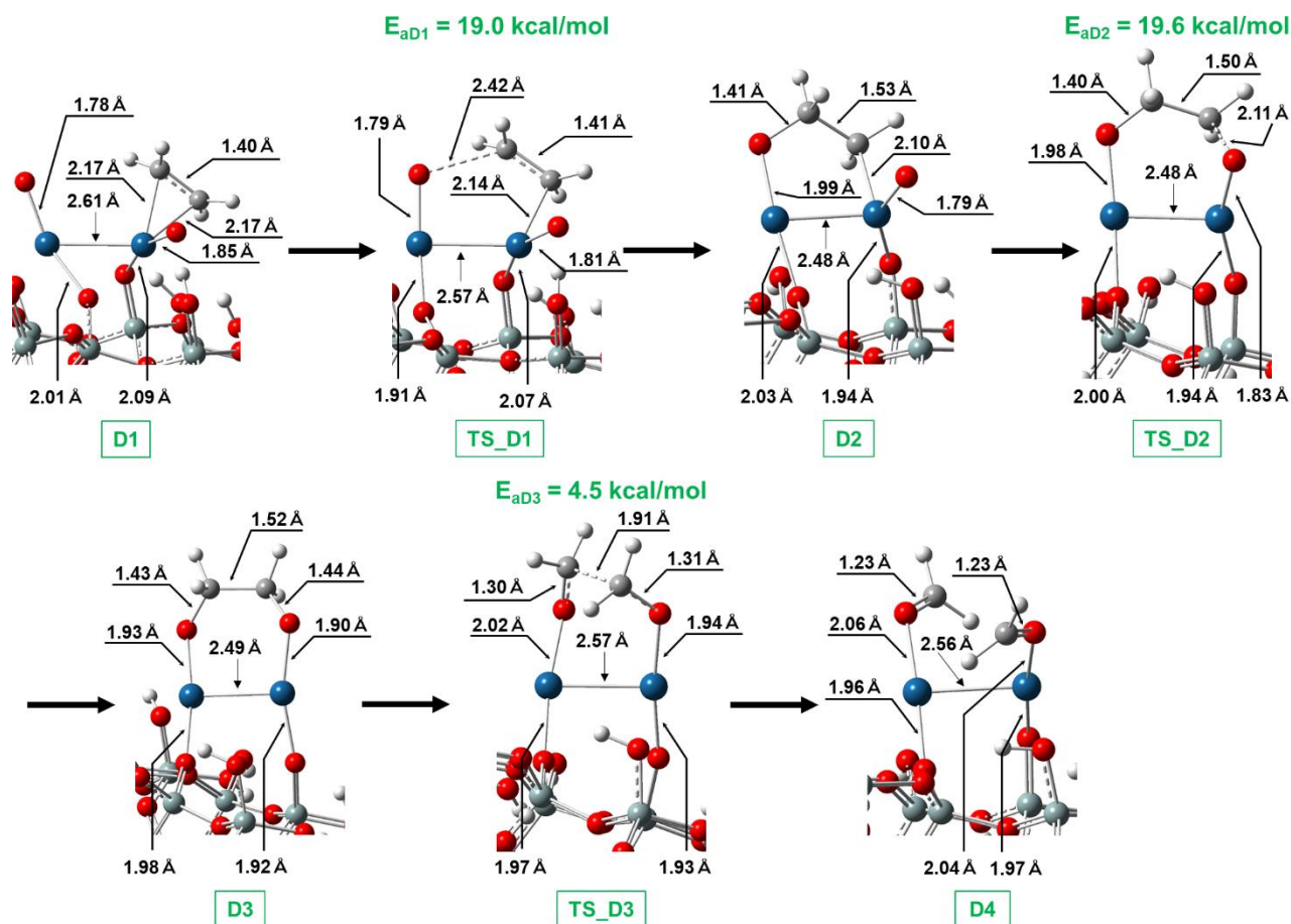
Figure 9. Optimized structures of the reactant, intermediate, transition, and product states of the HCHO generation on the \text{Pt}_2\text{-Si}_{\text{surf}} model. White: hydrogen, gray: carbon, red: oxygen, blue: platinum, green: silicon.
