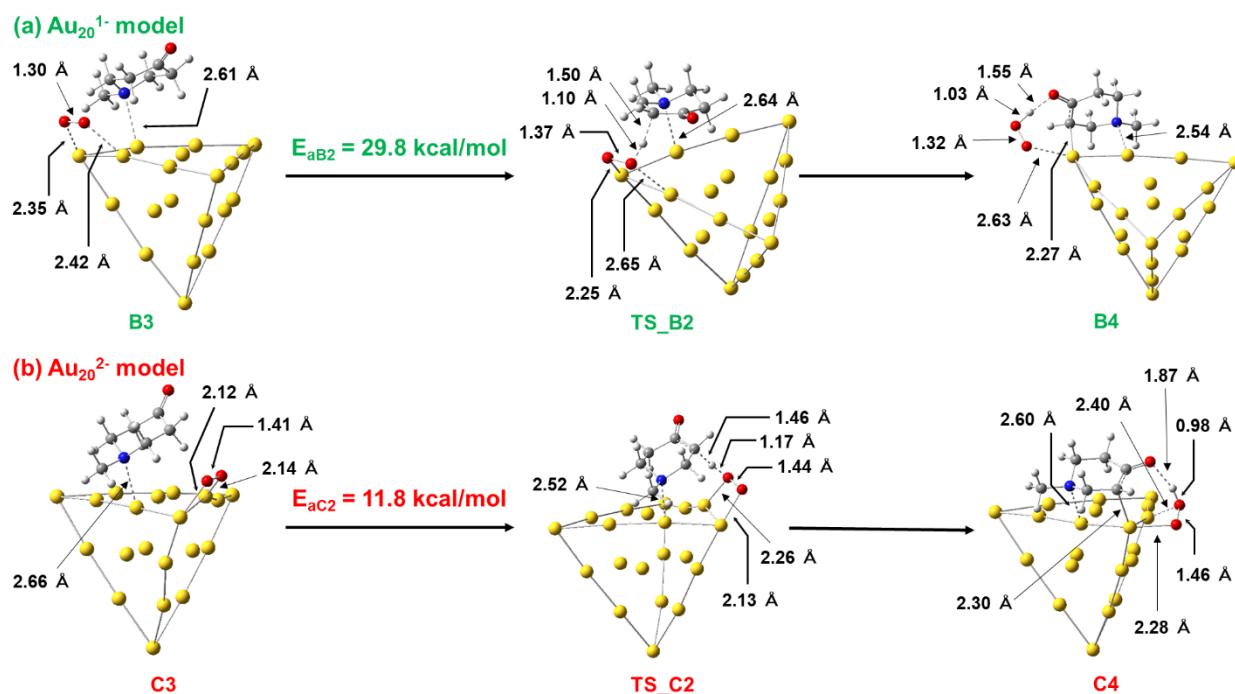
Figure 11. Optimized structures of the reactant, product and transition states of indirect \alpha -C-H bond activation at the 1 st step of the reaction on the (a) Au 20 1- model and (b) Au 20 2- model. Red ball: oxygen, blue ball: nitrogen, gray ball: carbon, white ball: hydrogen, yellow ball: gold.
