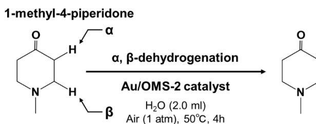
Scheme 1. Reaction scheme of \alpha , \beta -dehydrogenation of 1-methyl-4-piperidone on the Au/OMS-2 catalyst 16
