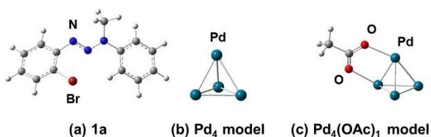
Figure 1. Computational models. (a) 1-(2-bromo)-3-methyl-3-phenyltriazene ( 1a ), (b) \text{Pd}_4 model, (c) \text{Pd}_4(\text{OAc})_1 model. White: hydrogen, gray: carbon, blue: nitrogen, dark red: bromide, blue green: palladium, red: oxygen.
