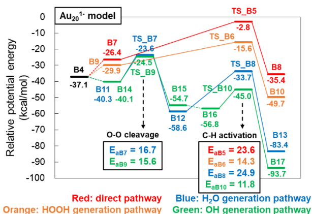
Figure 16. Potential energy diagram of \beta _C-H bond activation at the 2nd step of the reaction on the \text{Au}_{20}^{1-} model. Red line: direct pathway, orange line: HOOH generation pathway, blue line: H 2 O generation pathway, green line: OH generation pathway. Reference point of relative potential energies is defined as the sum of the energies of the isolated species: \text{Au}_{20}^{1-} , \text{O}_2 , and 1-methyl-4-piperidone.
