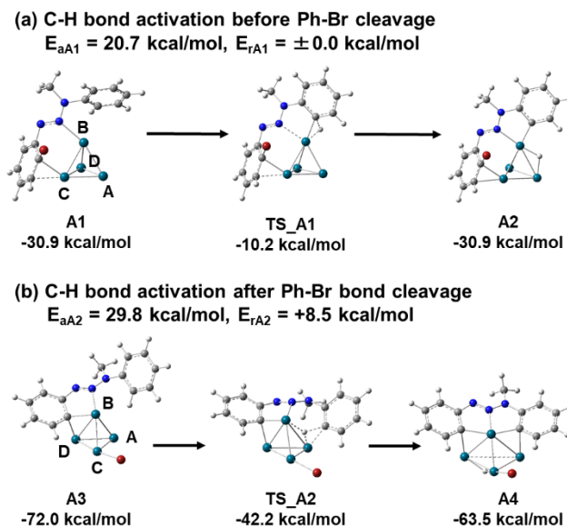
Figure 2. C-H bond activation pathways on the \text{Pd}_4 model. (a) C-H bond activation before Ph-Br bond cleavage, (b) C-H bond activation after Ph-Br bond cleavage. Numbers under structure names represent relative potential energies. Reference point of relative potential energy is sum of potential energies of isolated \text{Pd}_4 and 1a molecule. White: hydrogen, gray: carbon, blue: nitrogen, dark red: bromide, blue green: palladium.
