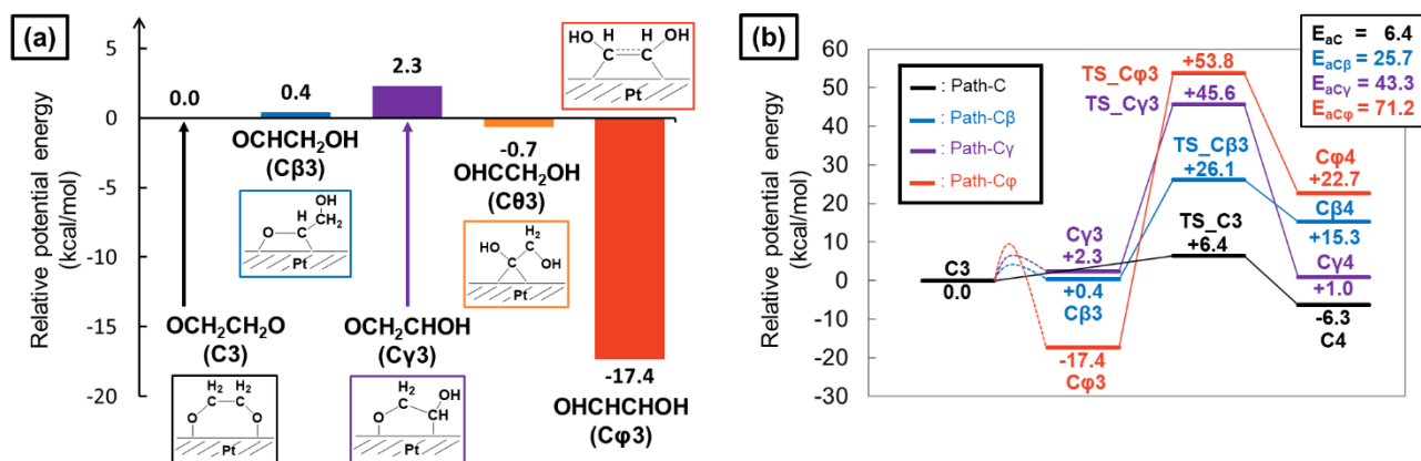
Figure 14. (a) Potential energy of the structural isomers of the ethylene dioxide relative to ethylene dioxide intermediate (C3). The Pt 2 -SiO 4 model was used for the computational model. (b) Potential energy diagram of the C-C σ-bond cleavage from the isomers. Black: reaction from C3 (Path-C), blue: reaction from Cβ3 (Path-Cβ), purple: reaction from Cγ3 (Path-Cγ), red: reaction from Cφ3 (Path-Cφ).
