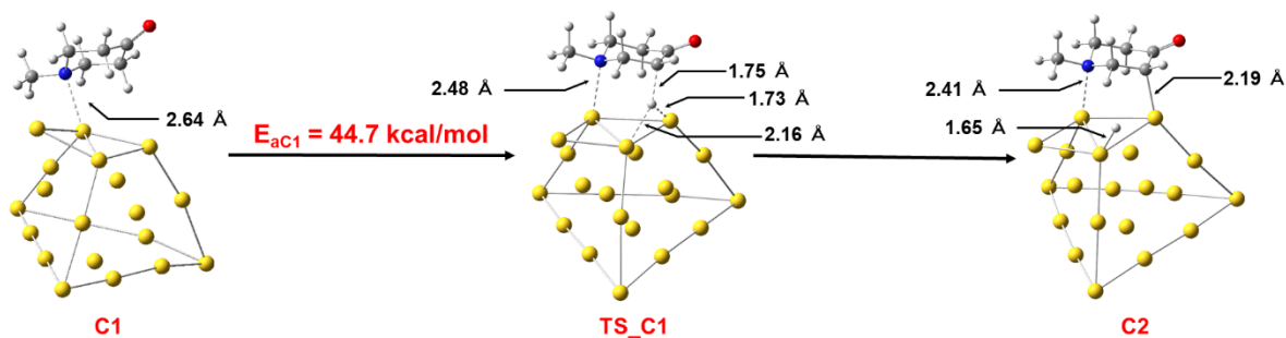
Figure 7. Optimized structures of the reactant, product and transition states of the direct \alpha _C-H bond activation at the 1st step of the reaction on the (a) \text{Au}_{20}^{0\pm} model, (b) \text{Au}_{20}^{1-} model and (c) \text{Au}_{20}^{2-} model. Red ball: oxygen, blue ball: nitrogen, gray ball: carbon, white ball: hydrogen, yellow ball: gold.
