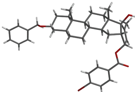
The structure of 22 determined by X-ray crystallographic analysis.
