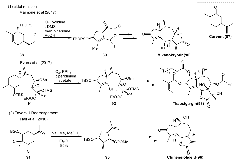
Scheme 2-1.
