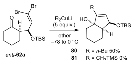
Scheme 3-1.
