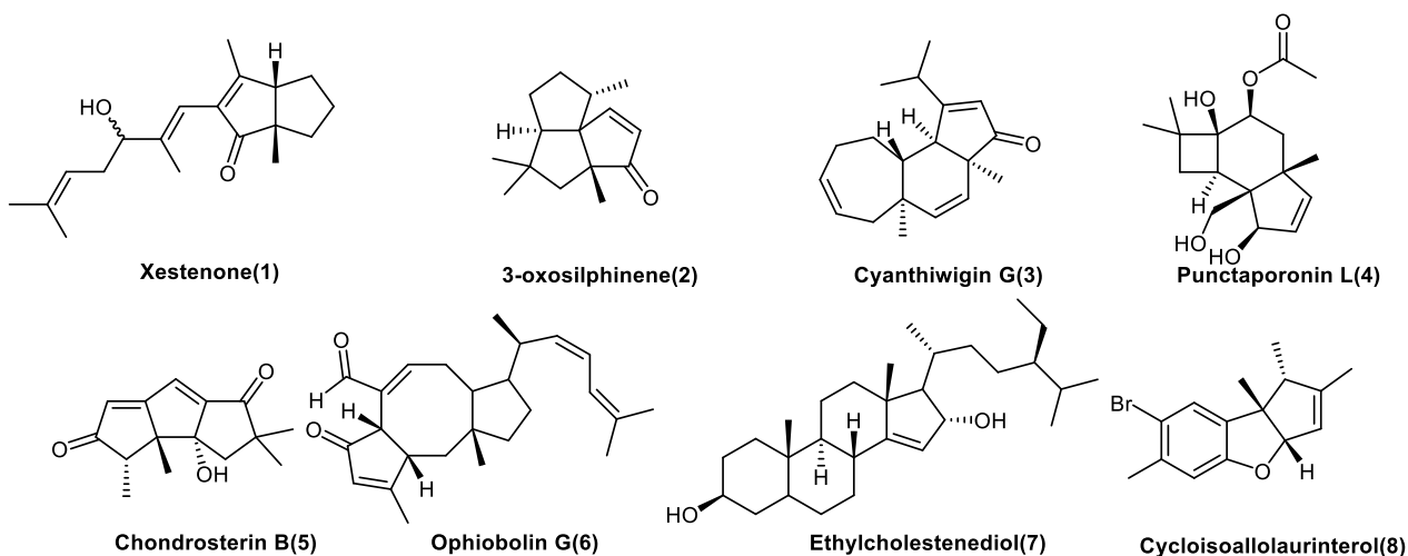
Scheme 1-1.
