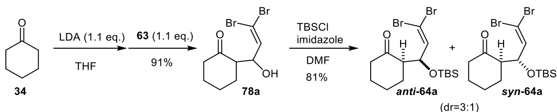
Scheme 1-13.
