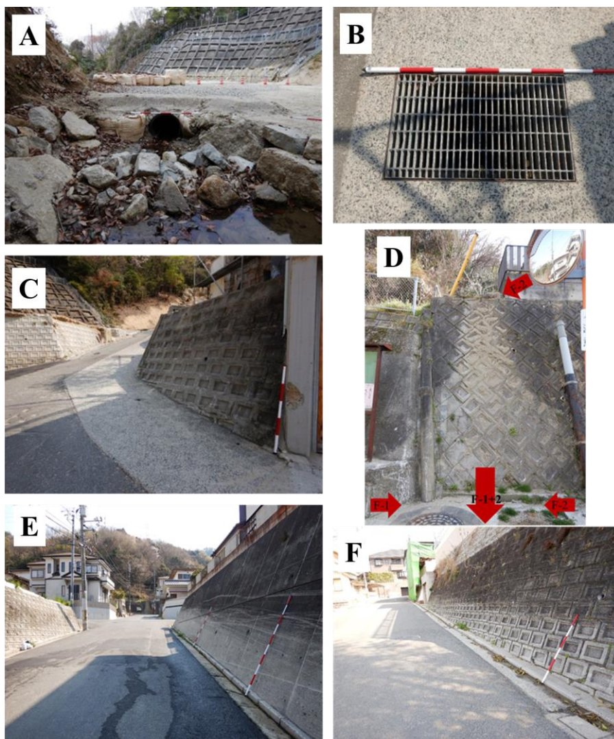
Fig. 3-7. Trace of debris flow and drainage
