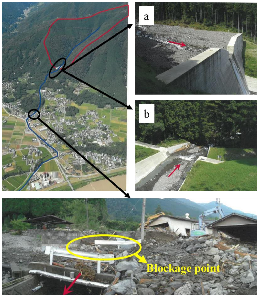
Fig. 1-8. Photographic of damaged area (Ibigawa, Japan)
