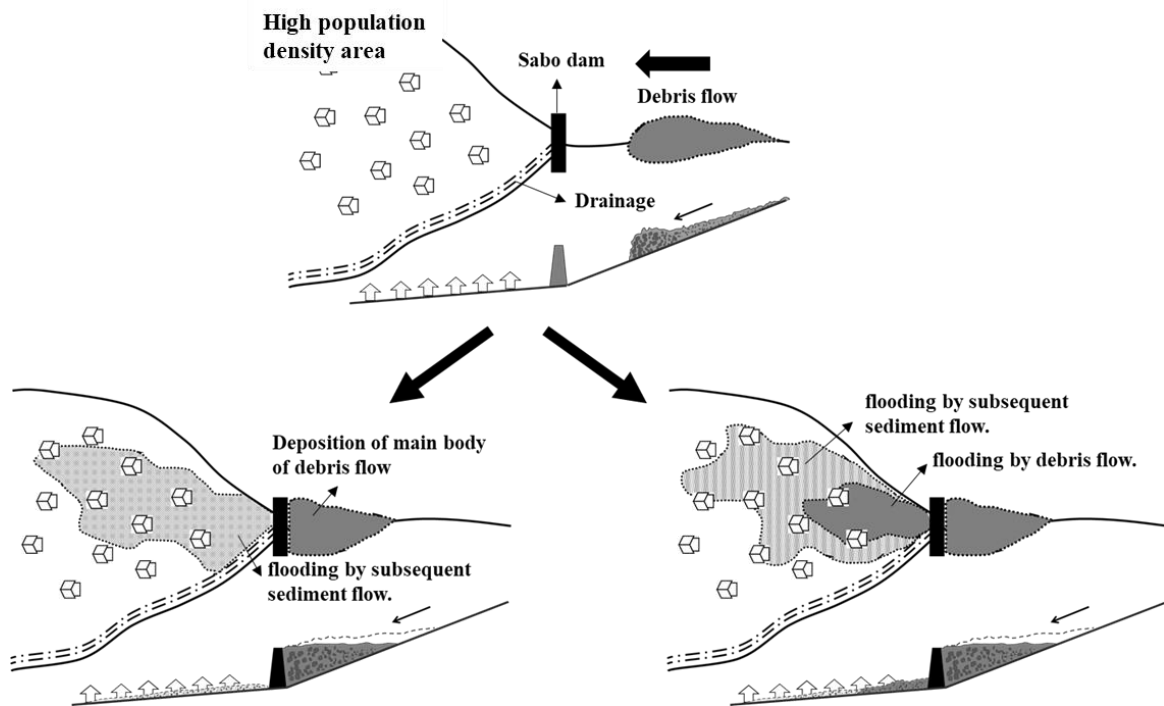
Fig. 1-3. Generation and kinds of SSF
