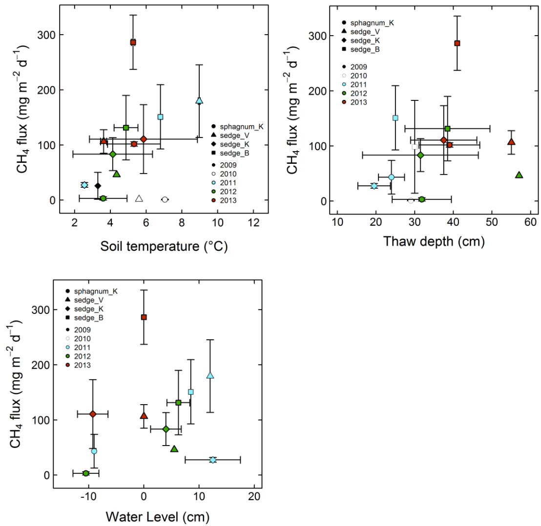
Fig. 3.6. Averaged CH 4 flux in each wet area in each year plotted against (a) soil temperature (10 cm in depth), (b) thaw depth, and (c) water level. Error bars represent standard deviations.
