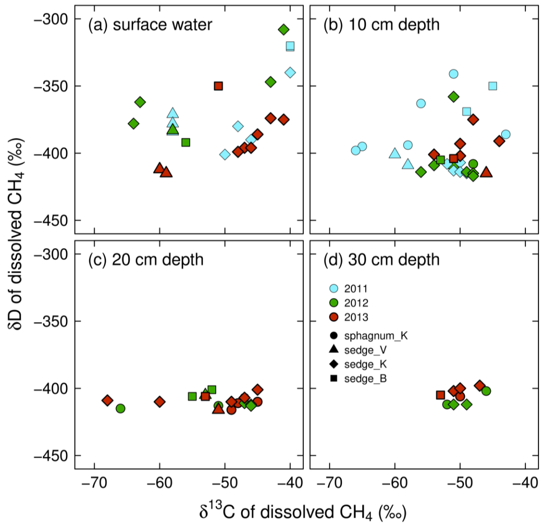
Fig. 4.1. In situ \delta^{13}\text{C} versus \delta\text{D} of dissolved \text{CH}_4 in (a) surface water and soil pore water at (b) 10 cm depth, (c) 20 cm depth, and (d) 30 cm depth from the wet event in 2011 to 2013. Individual \delta values are shown here. See Table 4.1 for averaged \delta values for each observation point and each year and Table 4.2 for individual numerical \delta values at 10 cm in depth in 2011.
