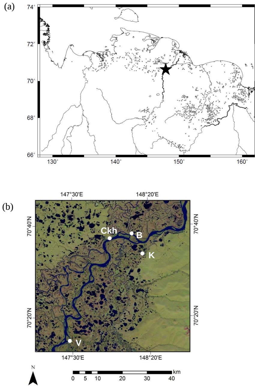
Fig. 2.1. Locations of study sites. (a) Location of study region in Northeastern Siberia (the Generic Mapping Tools 5.0.0). (b) Satellite image of Indigirka River lowland around Chokurdakh village (Ckh: 70° 37' N, 147° 55' E) from Landsat 8. Observation sites (V, K, B) were selected in this region alongside the main stem and a tributary of Indigirka River.
