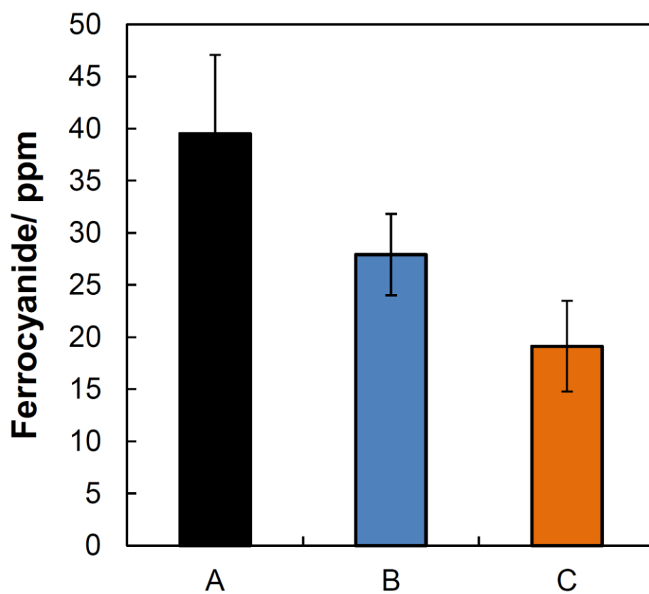
Fig. 14. Elution amount of ferrocyanide ion at pH 11 (containing 5 ppm of \text{Cs}^+ ). (A) PB-CF prepared at 0.35 V, (B) PAn-PB-CF prepared by 10 mM aniline solution, and (C) PAn-PB-CF prepared by 100 mM aniline solution.
