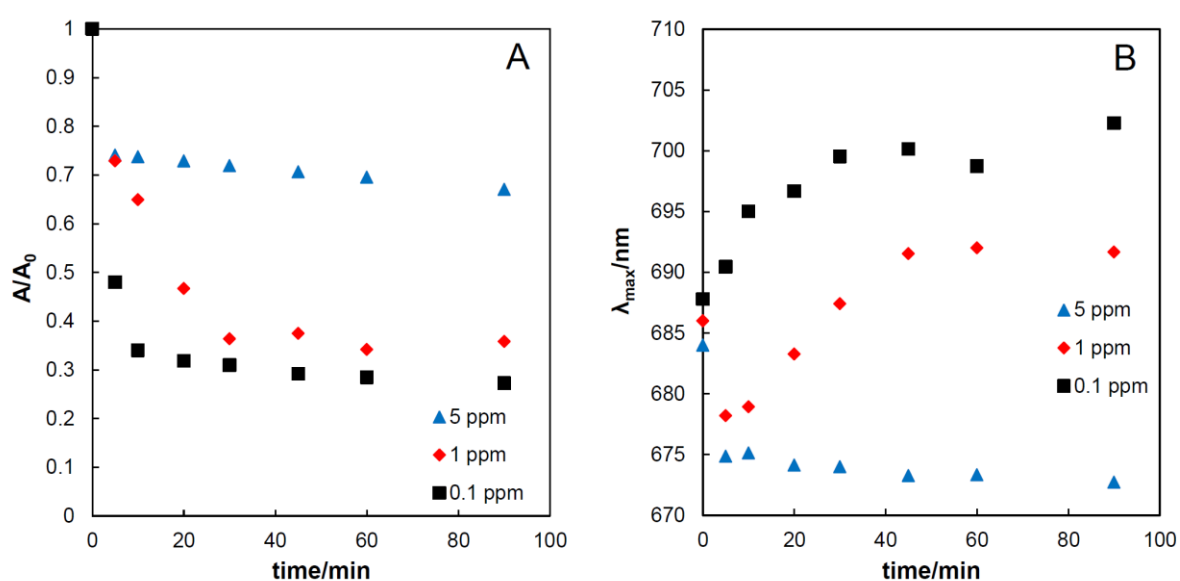
Fig. 5. Change of (A) maximum absorbance ratio, (B) maximum absorption wavelength, as a function of time after addition of 0.2 mL of 0.01 M NaOH in the presence of several \text{Cs}^+ concentrations.
