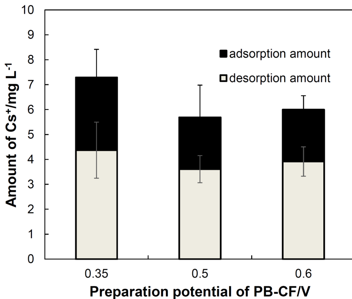
Fig. 5. Adsorption and desorption amount of \text{Cs}^+ from PB-CF prepared at several potentials. (Adsorption was performed in 10 mL of 10 ppm \text{Cs}^+ solution for 24 h, and desorption was performed in 10 mL of 0.5 M \text{NH}_4\text{Cl} solution for 3 h)
