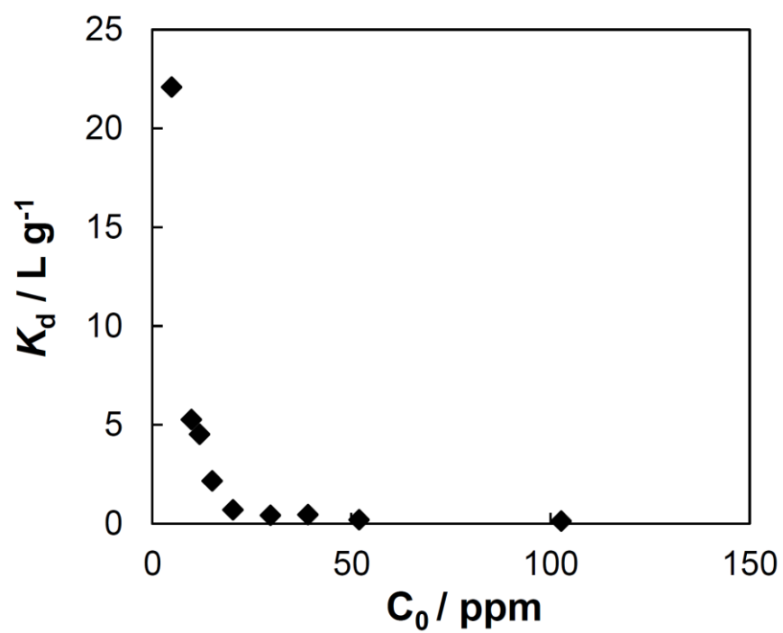
Fig. 13. Distribution coefficient ( K_d ) of PB-CF for Cs^+ in various initial concentrations (5-100 ppm).
