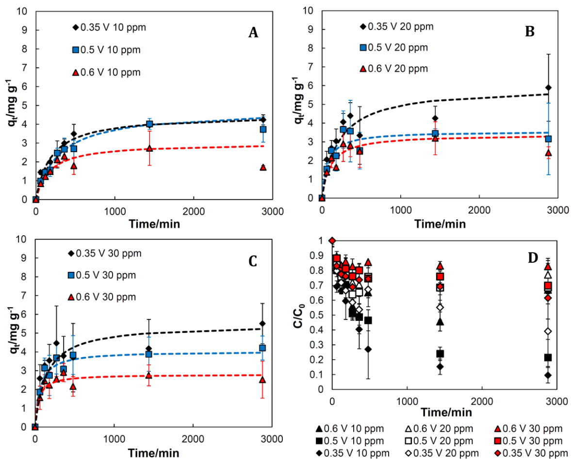
Fig. 2. Adsorption behaviors for \text{Cs}^+ on PB-CFs at several initial concentrations (diamond: PB-CF modified by potential of 0.35 V, square: PB-CF modified by potential of 0.5 V, triangle: PB-CF modified by potential of 0.6 V, dashed line: fitting for pseudo second order).
