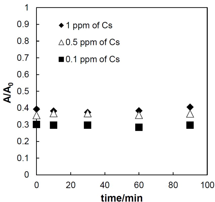
Fig. 4. Influence of contact times of several concentrations of \text{Cs}^+ on the degradation of PB.
