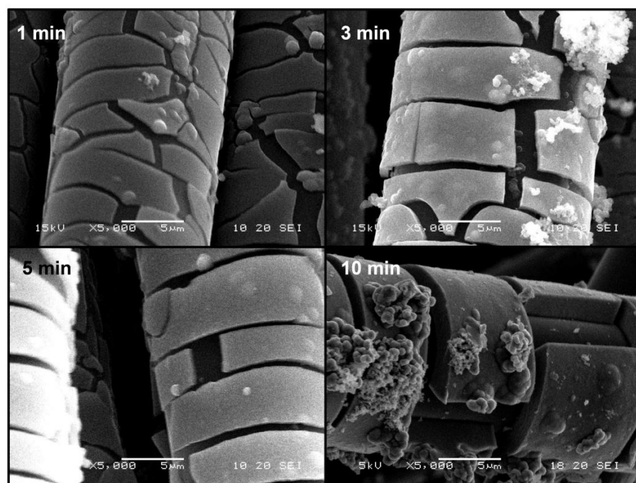
Fig. 7. SEM images of the PB-CF surface modified at 0.35 V for several minutes.
