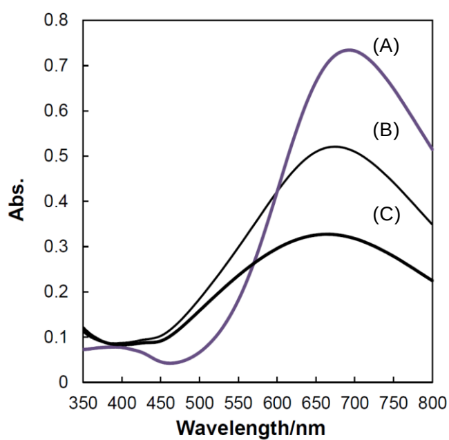
Fig. 7. Absorption spectrum of (A) 2 mM PB solution, (B) after the addition of 0.2 mL of 0.01 M NaOH in 5 ppm Cs + , and (C) after addition of 0.5 mL of 0.01 M NaOH in 5 ppm Cs + .
