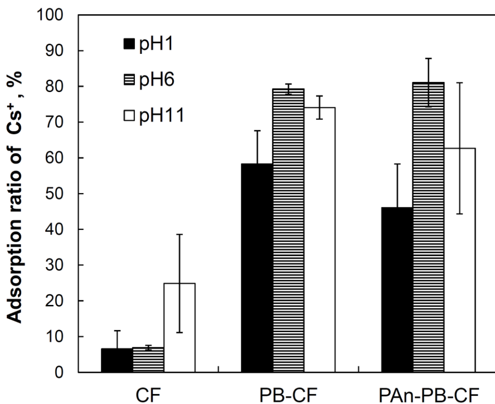
Fig. 8. Adsorption of \text{Cs}^+ using CF, PB-CF (PB modification potential: 0.35 V), and PAn-PB-CF in 5 ppm of CsCl solution.
