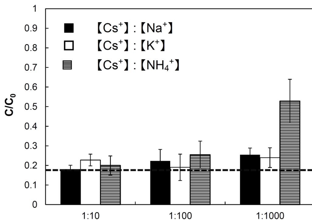
Fig. 4. \text{Cs}^+ adsorption with PB-CF in NaCl, KCl, and \text{NH}_4\text{Cl} solution (dashed line is adsorption ratio of \text{Cs}^+ without coexisting cation; ratio was calculated in units of mg/L).
