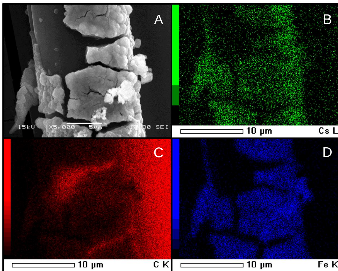
Fig. 12. EDS mapping images of PB-CF surface after 48 h of \text{Cs}^+ adsorption in the solution of pH 11. (A) SEM image of PB-CF, (B) Cs on PB-CF, (C) C on PB-CF, and (D) Fe on PB-CF.
