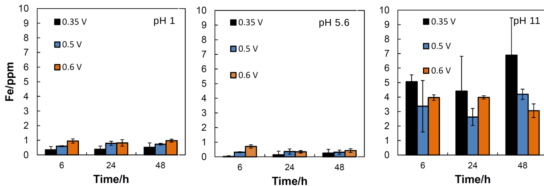
Fig. 12. Elution amount of iron ion from PB-CF after adsorption of \text{Cs}^+ in pH 1, 5.6, and 11.
