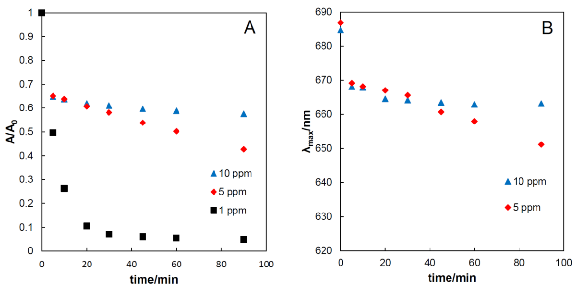
Fig. 8. Change of (A) maximum absorbance ratio, (B) maximum absorption wavelength as a function of time after the addition of 0.5 mL of 0.01 M NaOH at several \text{Cs}^+ concentrations.
