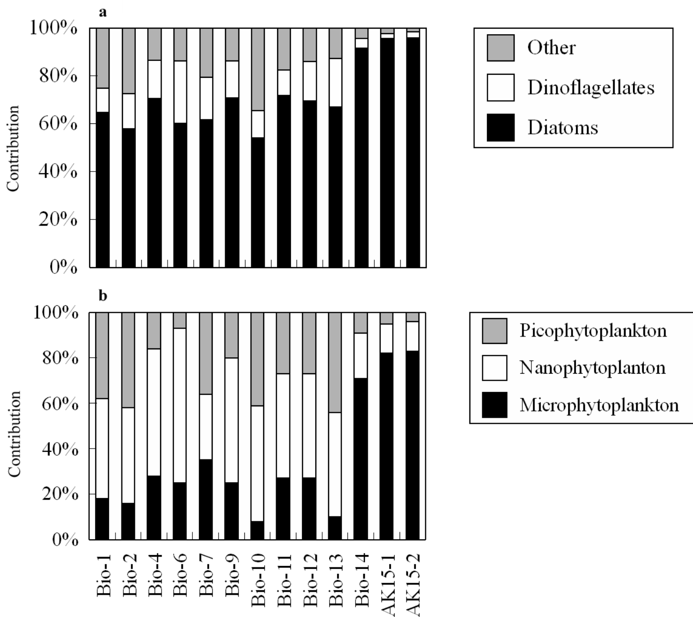
Figure 3. Relative contribution of phytoplankton groups to Chl a (a) at the class level class at the different sampling stations determined by multiple regression analysis based on diagnostic pigment signatures and (b) at the level of size class of phytoplankton determined by size-fractionated Chl a measurement.
