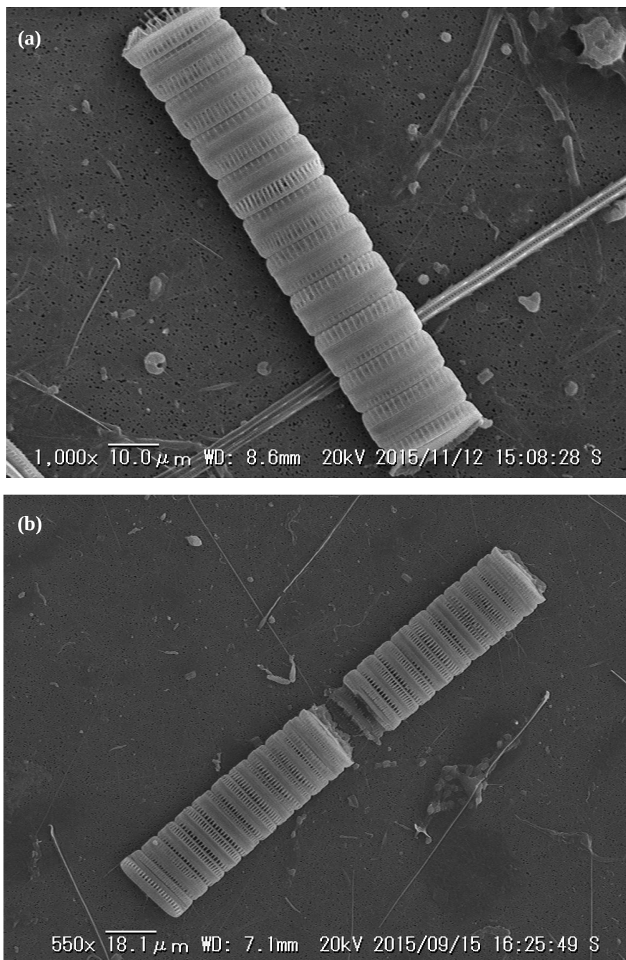
Figure 15. Electron micrographs of the diatom Neodenticula seminae in elongated chains from the +DFB bottles (a) at station C5 and (b) station A5.
