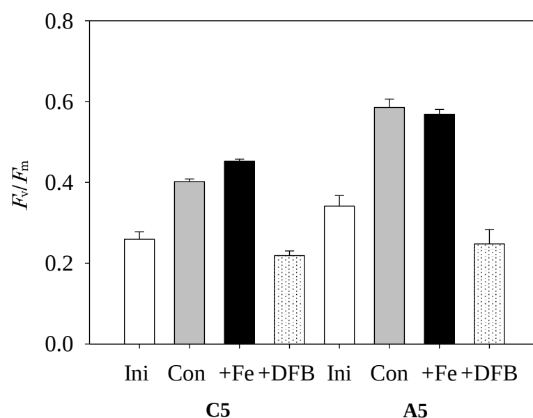
Figure 16. Maximum quantum yields of PSII ( F_v/F_m ) determined with PAM fluotometry of each treatment of the Fe enrichment incubation experiments.
