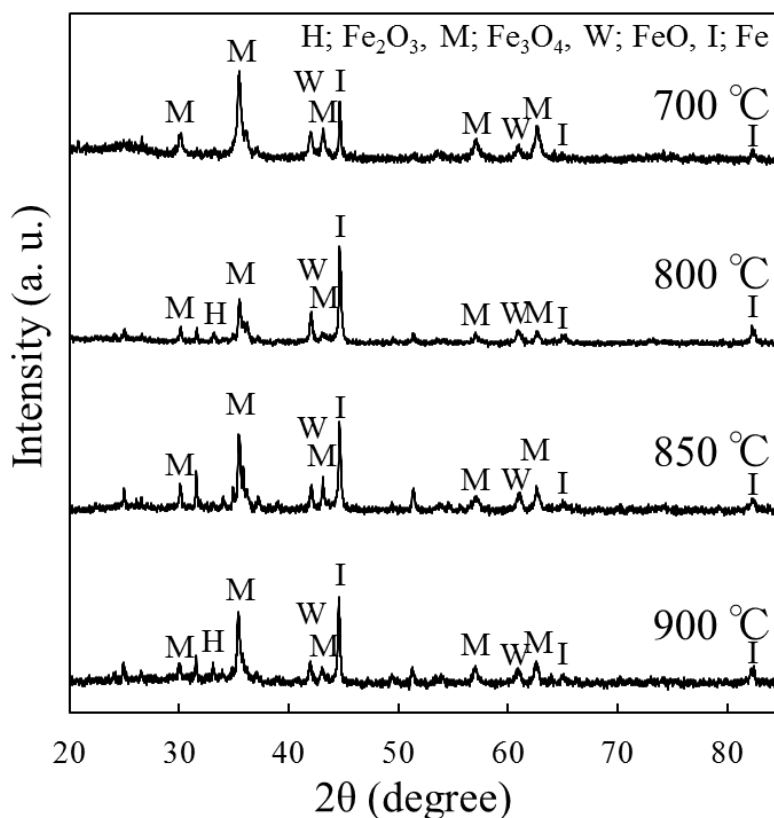
Figure 4-14 XRD patterns of the goethite ore after the CS experiments flowing 1 L \text{min}^{-1} of 25 vol% O_2 /Ar at 700, 800, 850, and 900^\circ\text{C} .
