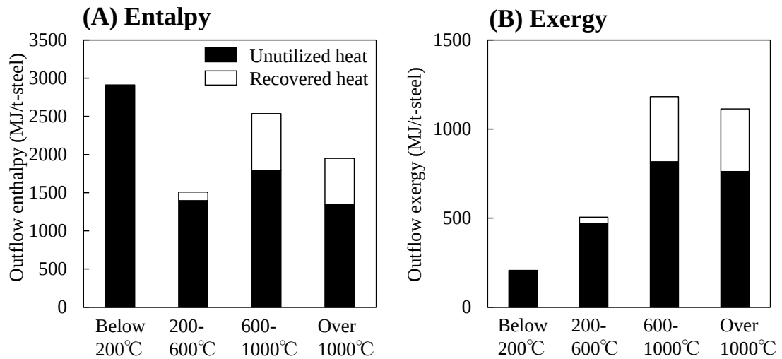
Figure 1-3 The amount of waste heat in the iron and steel industry [10].
