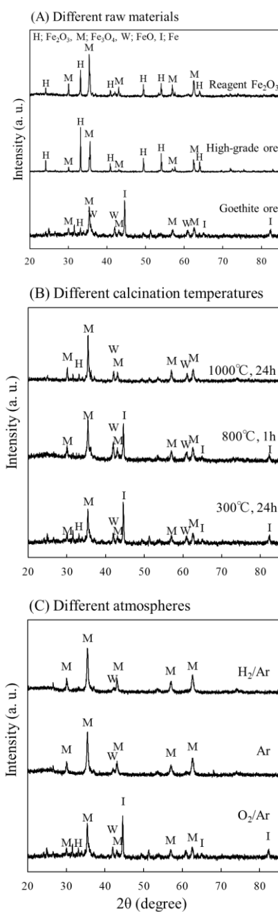
Figure 4-10. XRD patterns of the products from the combustion synthesis experiments. (A) Different raw materials: goethite ore, high-grade ore, and \text{Fe}_2\text{O}_3 reagent; (B) Different goethite ore calcination temperatures: 300, 800, and 1000 °C; and (C) Different atmospheres: 25 vol% \text{O}_2/\text{Ar} , Ar, and 20 vol% \text{H}_2/\text{Ar} were flowed to the carbon-infiltrated goethite ore.
