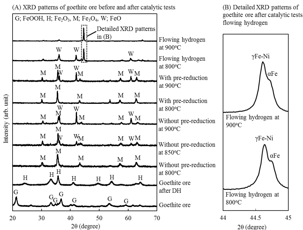
Figure 3-6 (A) XRD patterns of goethite ore, after DH, after the catalytic test at 800-900 °C without reduction ( \text{Ar}:\text{CH}_4:\text{CO}_2 = 8:1:1 ), after the catalytic test at 800 and 900 °C with pre-reduction ( \text{Ar}:\text{CH}_4:\text{CO}_2 = 8:1:1 ), and after the catalytic test at 800 and 900 °C with flowing hydrogen ( \text{Ar}:\text{H}_2:\text{CH}_4:\text{CO}_2 = 7:1:1:1 ). (B) Detailed XRD patterns of goethite ore after the catalytic test at 800 and 900 °C with flowing hydrogen ( \text{Ar}:\text{H}_2:\text{CH}_4:\text{CO}_2 = 7:1:1:1 ). The total gas flow rate to the ore catalyst was 30 L/(h·g cat ).
