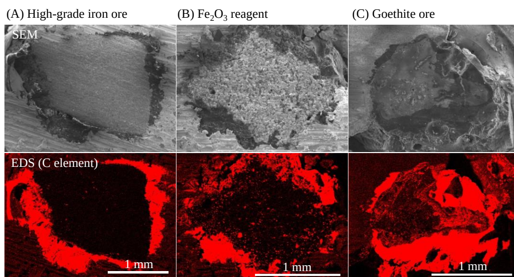
Figure 4-9. Cross-sectional SEM-EDS observations of carbon-infiltrated high-grade iron ore, \text{Fe}_2\text{O}_3 reagent, and goethite ore. The red areas in the EDS images correspond to carbon.
