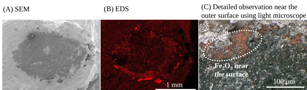
Figure 4-13 Cross-sectional observation of the goethite ore after CS experiments flowing 1 \text{ L min}^{-1} of 25 vol% \text{O}_2/\text{Ar} at 900^\circ\text{C} .
