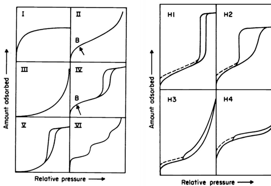
Figure 2-5 Types of physisorption isotherms and hysteresis loops [24]
