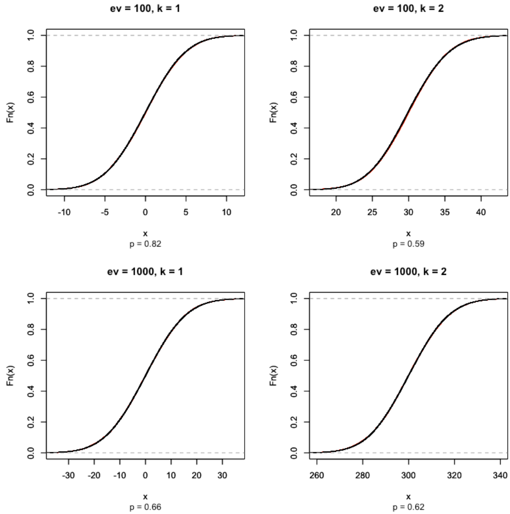
Fig. 2.1b. An empirical distribution of a simulated trait change by the two algorithms ( ev = 100, 1000 ). Red line corresponds to the A-1 algorithm and the black one to A-2. The x-axis indicates the trait change and y-axis indicates the cumulative density of the random variable.
