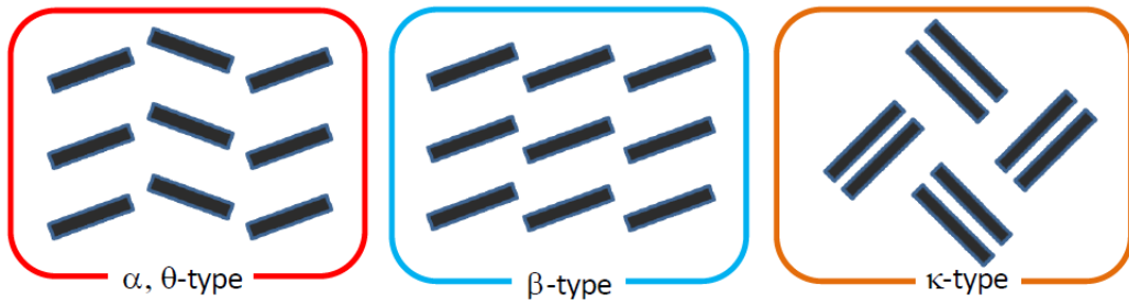
Figure 1.4: Arrangements of ET molecule in conducting sheet.
