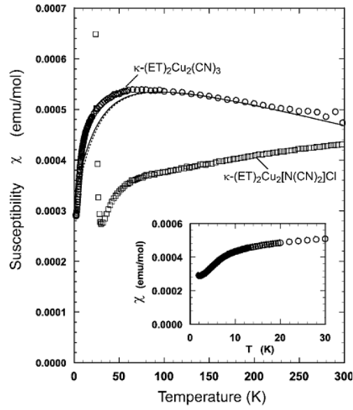
Figure 1.10: Magnetic susceptibility of \kappa\text{-(ET)}_2X ( X=\text{Cu}_2(\text{CN})_3 and \text{Cu[N(CN)}_2\text{]Cl} ). [11]
