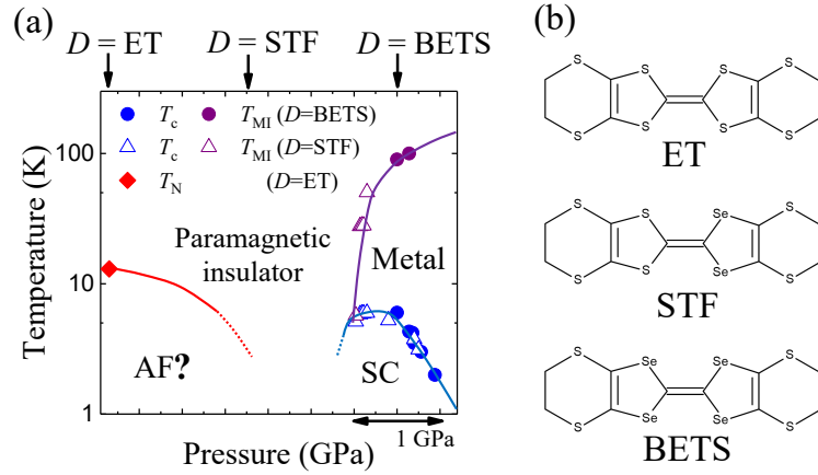
Figure 1.31: (a) Pressure-temperature phase diagram of \lambda - D_2\text{GaCl}_4 ( D = \text{ET}, \text{STF}, \text{and BETS} ). T_c , T_{MI} , and T_N represent the superconducting transition temperature, metal-insulator transition temperature, and Néel temperature, respectively. The data are cited from Refs. [31, 30, 32]. (b) Molecular structure of ET, STF, and BETS.
