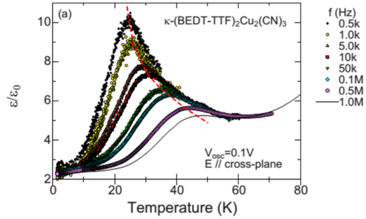
Figure 1.15: Temperature dependence of the dielectric constant with respect to various frequencies of \kappa\text{-(ET)}_2\text{Cu}_2(\text{CN})_3 . [14]
