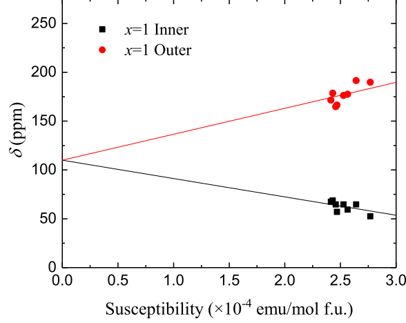
Figure 4.20: Temperature dependence of \delta - \chi plot for x = 1 sample.
