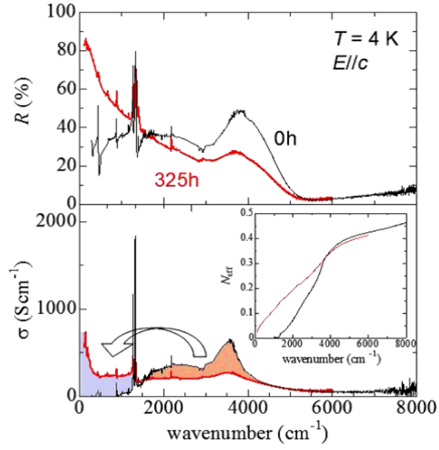
Figure 1.22: Infrared optical reflectivity and conductivity of \kappa -(ET) 2 Cu[N(CN) 2 ]Cl before and after X-ray irradiation. The inset of the lower panel indicates the effective number of carriers N_{eff} . [22]
