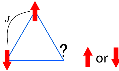
Figure 1.13: Antiferromagnetically interacting spins in a triangular lattice.
