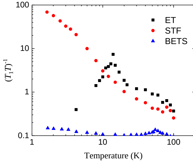
Figure 5.16: (T_1T)^{-1} of \lambda -ET, STF, and BETS salts as a function of temperature.
