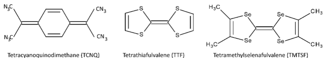
Figure 1.1: Molecular structure of TCNQ, TTF, and TMTSF.
