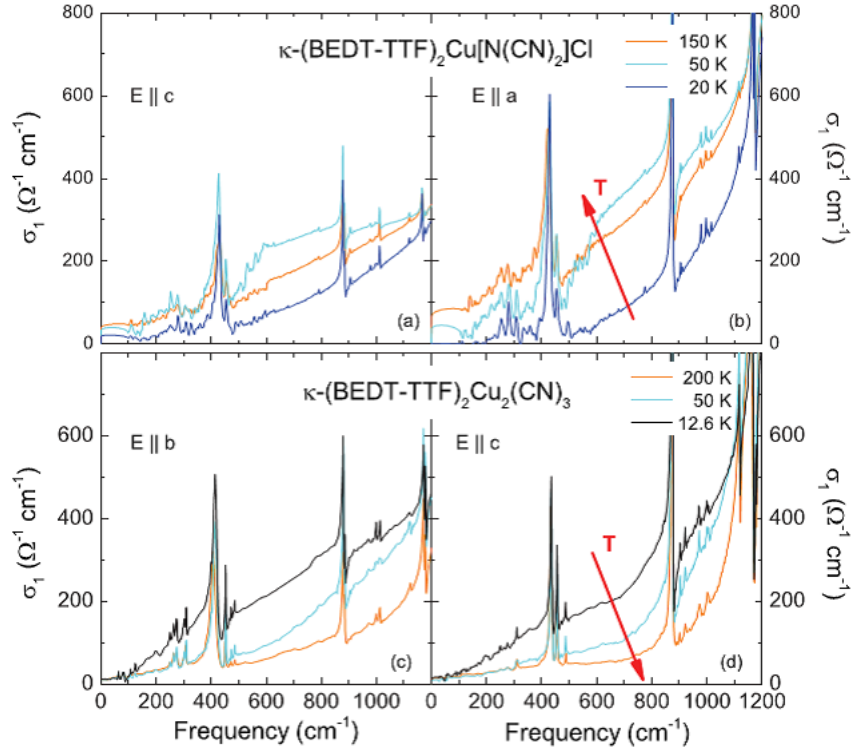
Figure 1.14: Optical conductivity of (a) and (b) \kappa -(ET) _2X ( X=\text{Cu}[\text{N}(\text{CN})_2]\text{Cl} and (c) and (d) \text{Cu}_2(\text{CN})_3 ) for the two in-plane polarizations.[13]
