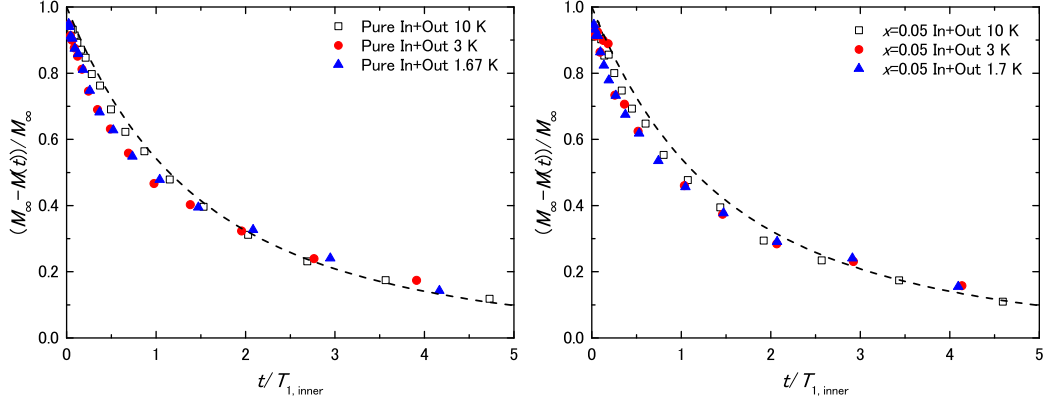
Figure 4.17: Recovery curve of pure sample at several temperatures. Figure 4.18: Recovery curve of x=0.05 sample at several temperatures.
