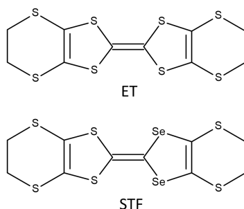
Figure 1.25: Molecular structure of ET and STF.
