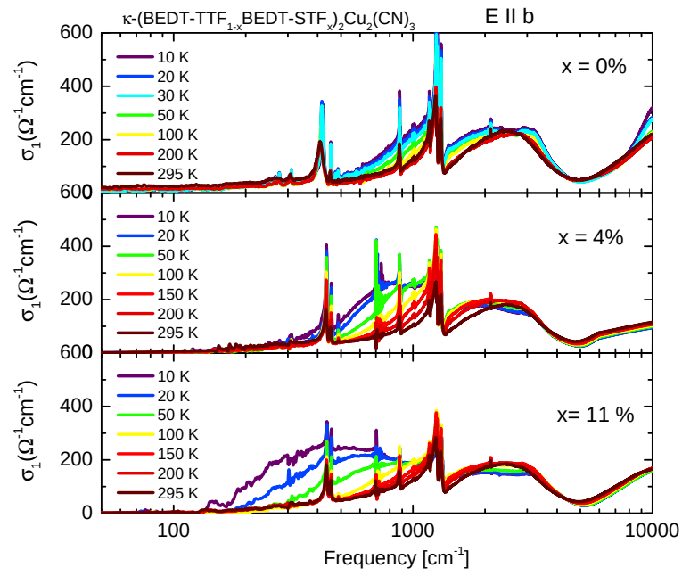
Figure 5.5: Optical conductivity of pure, x = 0.4 , x = 0.11 samples for E \parallel b .
