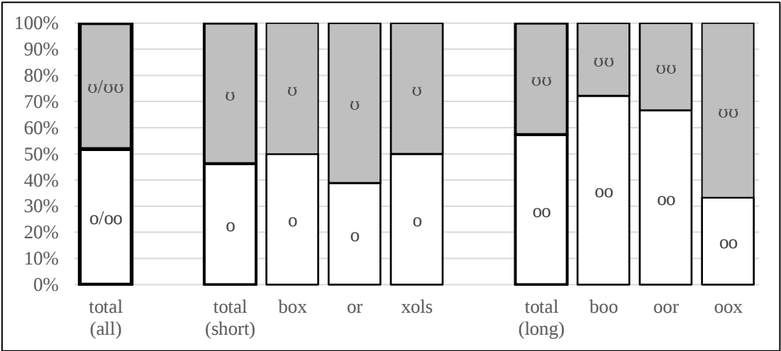
Figure 15. Judging of stimulus sounds /o/ and /oo/
