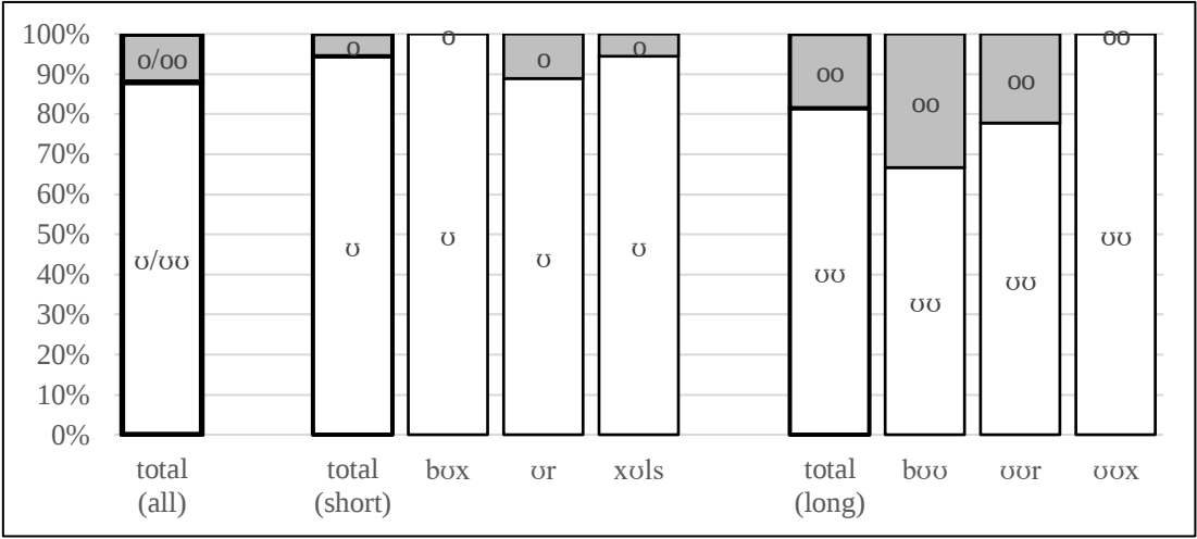
Figure 14. Judging of stimulus sounds /ʊ/ and /ʊʊ/
