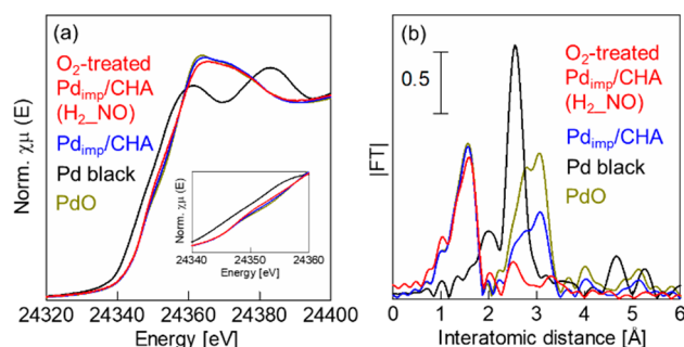
Figure 3. (a) Ex situ XANES and (b) FT of EXAFS spectra of Pd imp /CHA, O 2 -treated Pd imp /CHA(H 2 NO), and reference samples (Pd Black and PdO) obtained under ambient conditions (air at room temperature).
