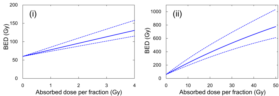
(B) p_{O_2} = 0.5\% for hypoxia
