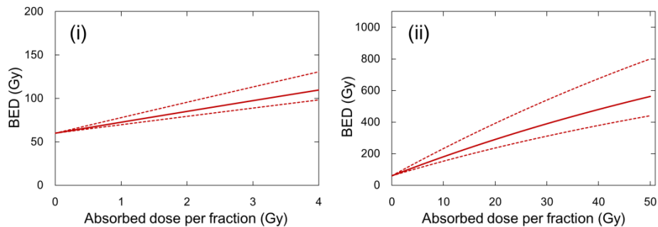
(C) p_{O_2} = 0\% for anoxia
