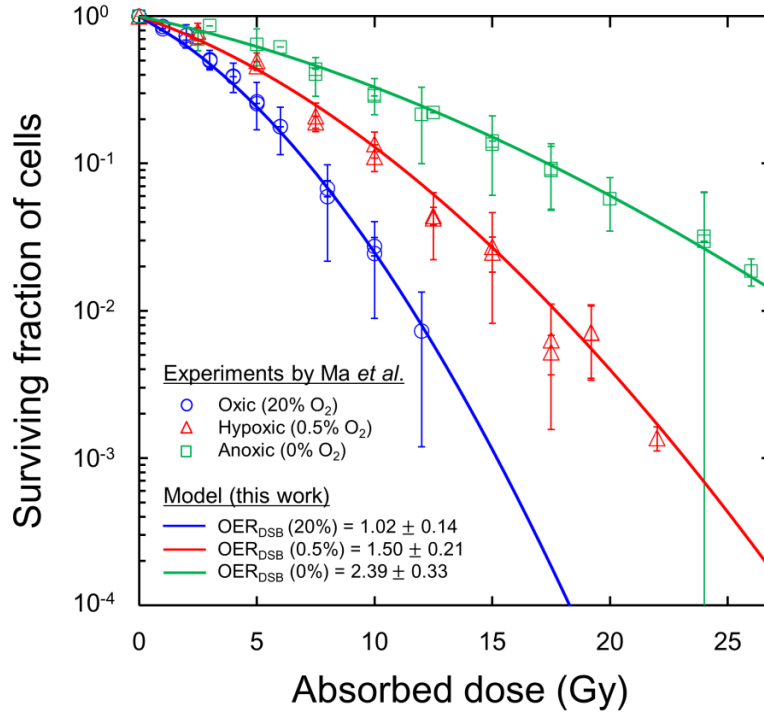
Fig. 1. Cell survival curve for various oxygen concentrations acutely created. The model parameters \alpha_0 , \beta_0 , \gamma , (a+c) , \text{OER}_{\text{DSB}}(0\%) and p_{\text{O}_2, \text{half}} which describe the survival curve are listed in Table I. In Fig. 1, the line and symbol represent the calculated curve and the experimental data, 14,15 respectively, for three oxygen pressures, i.e., p_{\text{O}_2} = 0\% , 0.5\% and 20\% . Note that the cell-cycle is in a logarithmic growth phase in the cell growth curve.
