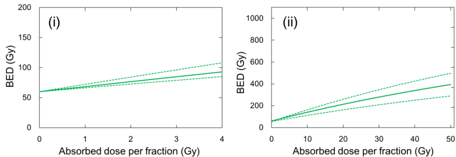
Fig. 5. BED as functions of dose per fraction and oxygen concentration: (A) oxia, (B) hypoxia and (C) anoxia. Left and right panels are the range of low dose per fraction and that of the wide dose range. A realistic clinical case to eliminate NSCLC in the external radiotherapy with 6MV-linac X-rays at 2.5 Gy/min is assumed. Solid line and dotted line represent the mean value and the 68% uncertainty, which are calculated by using the set of model parameters in H1299 cells as reported previously. 35
