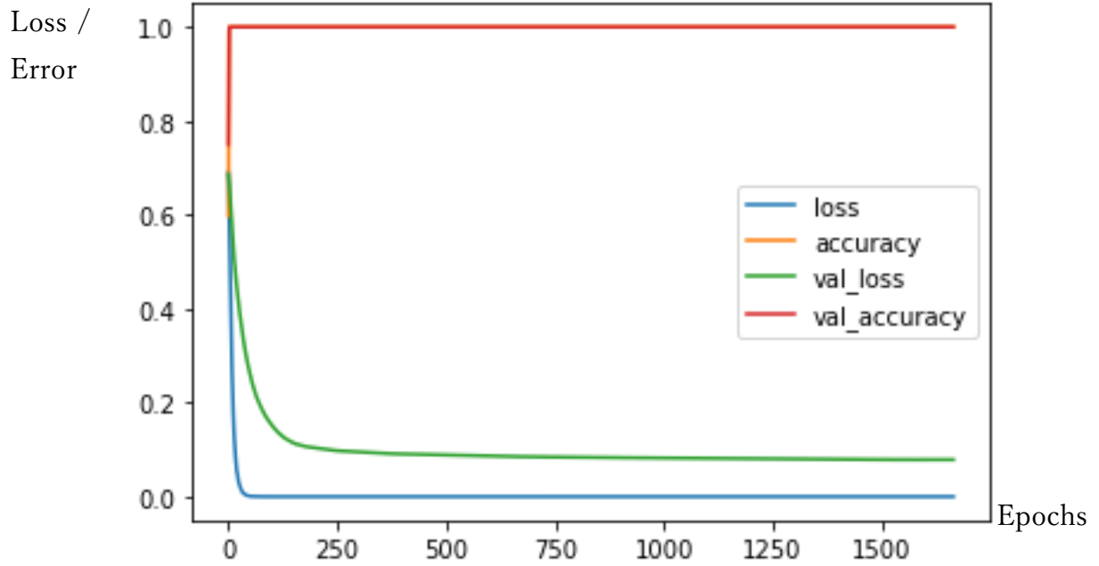
Figure 2: Neural network training performance (Early stopping at epoch 01666)
