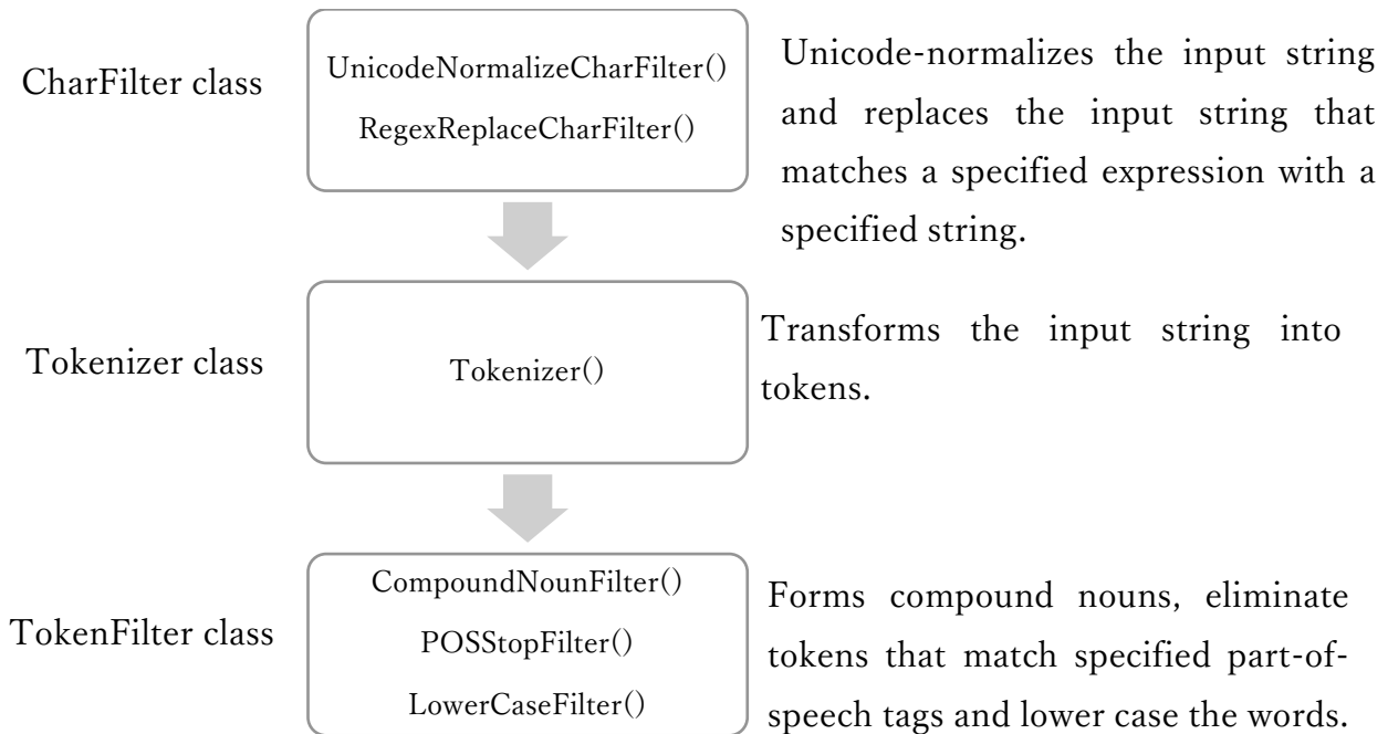
Figure 1: Analyzer framework of Janome (Uchida, 2020)
