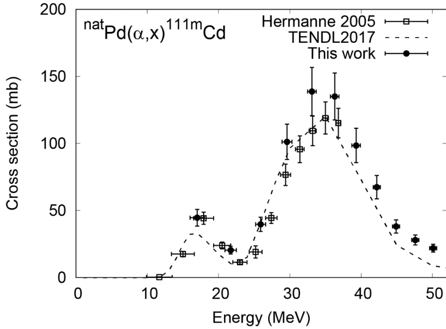
Fig. 2. The excitation function of the ^{nat}\text{Pd}(\alpha, x)^{111m}\text{Cd} reaction.
