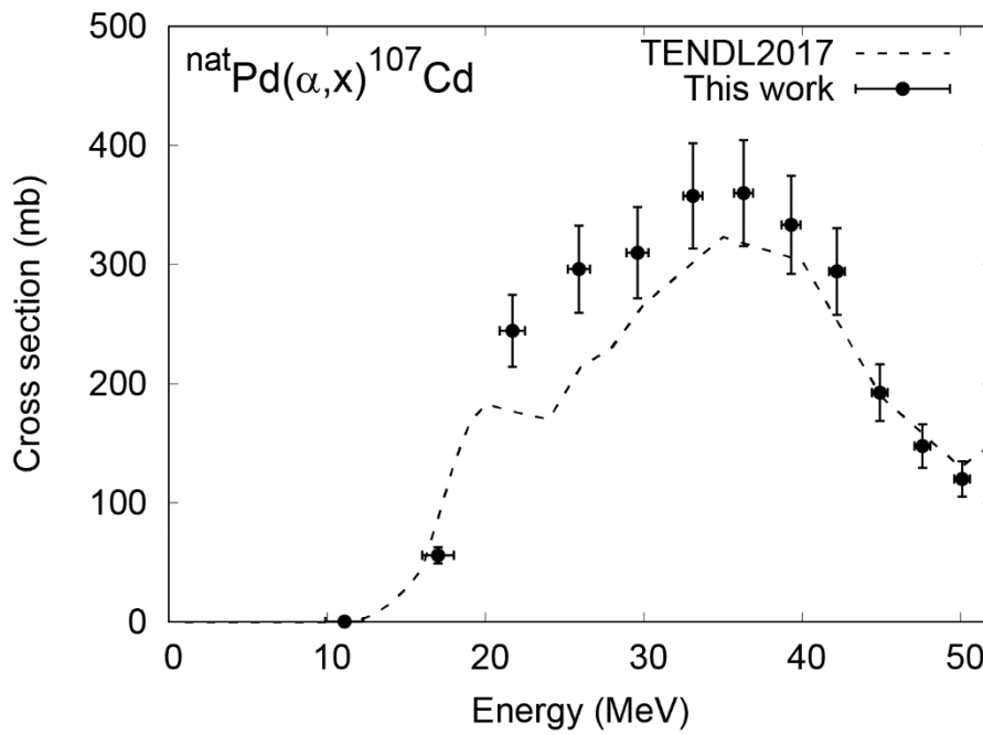
Fig. 4. The excitation function of the ^{nat}\text{Pd}(\alpha, x)^{107}\text{Cd} reaction.
