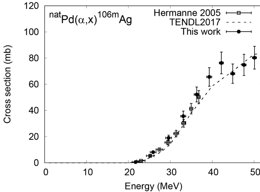
Fig. 9: The excitation function of the ^{nat}\text{Pd}(\alpha, x)^{106m}\text{Ag} reaction.
