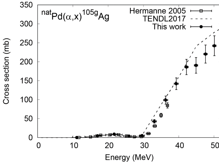
Fig. 10. The excitation function of the ^{nat}\text{Pd}(\alpha, x)^{105g}\text{Ag} reaction.
