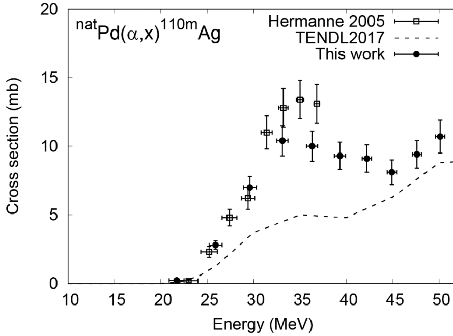
Fig. 8. The excitation function of the ^{nat}\text{Pd}(\alpha, x)^{110\text{m}}\text{Ag} reaction.
