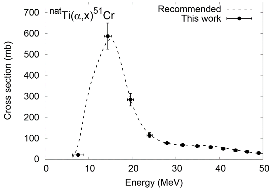
Fig. 1. Comparison of the recommended excitation function of the ^{nat}\text{Ti}(\alpha, x)^{51}\text{Cr} monitor reaction with the experimental cross section values.
