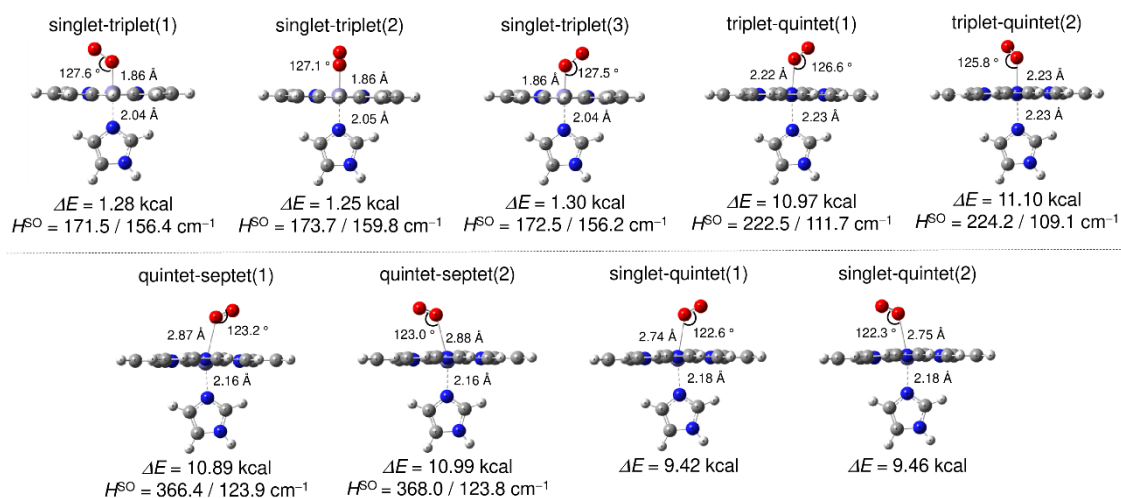
Figure 3: Spin-inversion structures optimized on the mixed-spin potential energy surfaces. Geometric parameters and relative energies ( \Delta E in kcal/mol) measured from the most stable singlet minimum structure are also presented. Spin-orbit coupling constants (maximum and averaged values in cm -1 , see text for detail) calculated at the spin-inversion structure are also shown.
