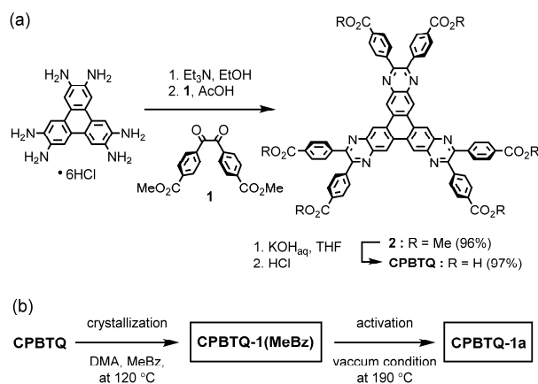
Scheme 1. (a) Synthesis and (b) crystallization of CPBTQ
