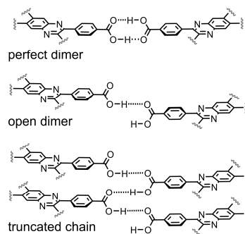
Figure 3. H-bonding patterns of carboxy groups observed in a crystal structure of CPBTQ-1(MeBz) .
