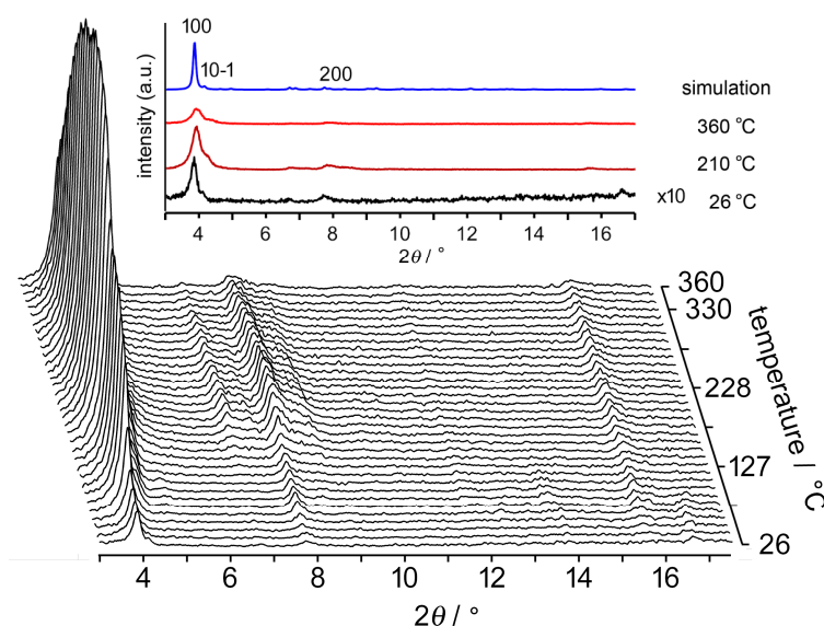
Figure 6. Variable temperature (VT) PXRD patterns of crystalline bulk of as-formed CPBTQ-1 . Temperature was increased at the rate of 1\text{ }^{\circ}\text{C min}^{-1} . PXRD patterns were recorded from 3^{\circ} to 18^{\circ} of 2\theta with the scan rate of 3^{\circ}\text{min}^{-1} . Therefore, each scan has a temperature gradient of 5\text{ }^{\circ}\text{C} . The inserted PXRD pattern at 26\text{ }^{\circ}\text{C} is magnified 10 times for clarity.
