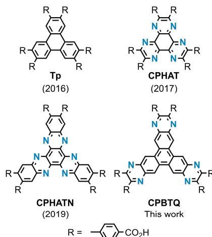
Chart 1. C_3 -symmetric \pi -conjugated molecules ( C_3\text{PI} ) without and with incorporated pyrazine rings as a building blocks to construct porous hydrogen-bonded organic frameworks.
