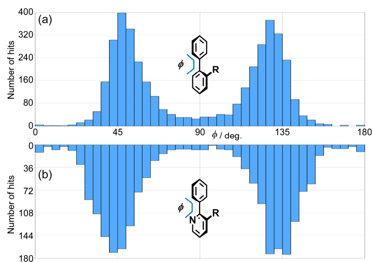
Figure 5. Dihedral angle distribution of (a) phenyl-benzene and (b) phenyl-pyridine systems possessing substituents at the ortho -position of the phenyl group.
