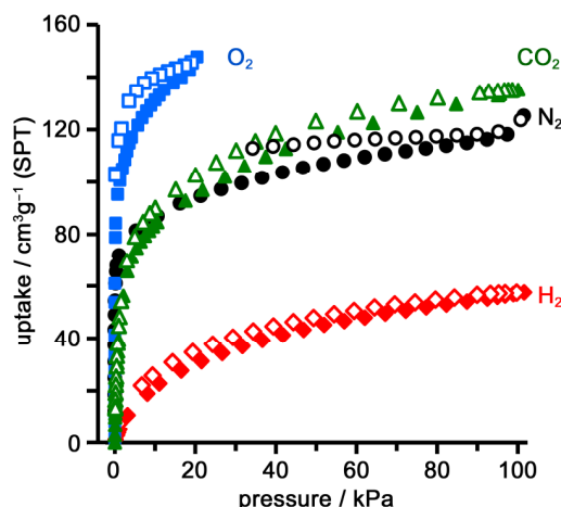
Figure 7. Gas sorption isotherms of CPBTQ-1a at low temperature. Nitrogen (black circle) at 77K, carbon dioxide (green triangle) at 195 K, oxygen (blue square) at 77K, and hydrogen (red diamond) at 77K. Solid symbol: absorption. Open symbol: desorption.
