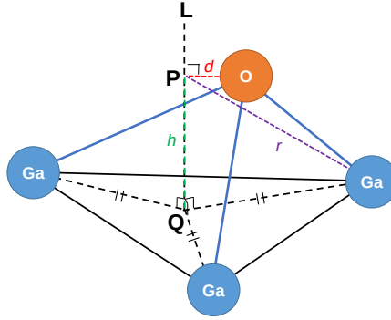
Fig. 7. Definition of coordination environment descriptors.
