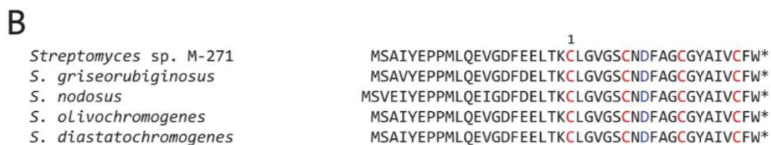
Figure 3-2-1-1. Msl -like clusters. (A) The gene organizations of the clusters. Identities to Msl proteins from Streptomyces sp. M-271 are shown in parentheses. (B) Sequence alignment of precursor peptides.
