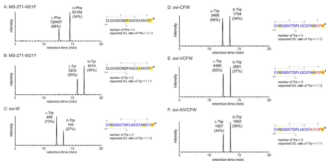
Figure 3-2-3-3 Chiral analysis of MS-271 derivatives. (A) Phe in MS-271-W21F, (B) Tyr in MS-271- W21Y, (C) Trp in svi-W, (D) Trp in svi-CFW, (E) Trp in svi-VCFW, and (F) Trp in svi-AIVCFW. The LC-MS chromatograms of L-FDLA derivatives of Phe, Tyr, and Trp were monitored at m/z 458, 474, and 497, respectively. Peak areas in UV traces at 340 nm are shown in the chromatograms. The amino acids subjected to chiral analysis are highlighted in yellow in the structures.
