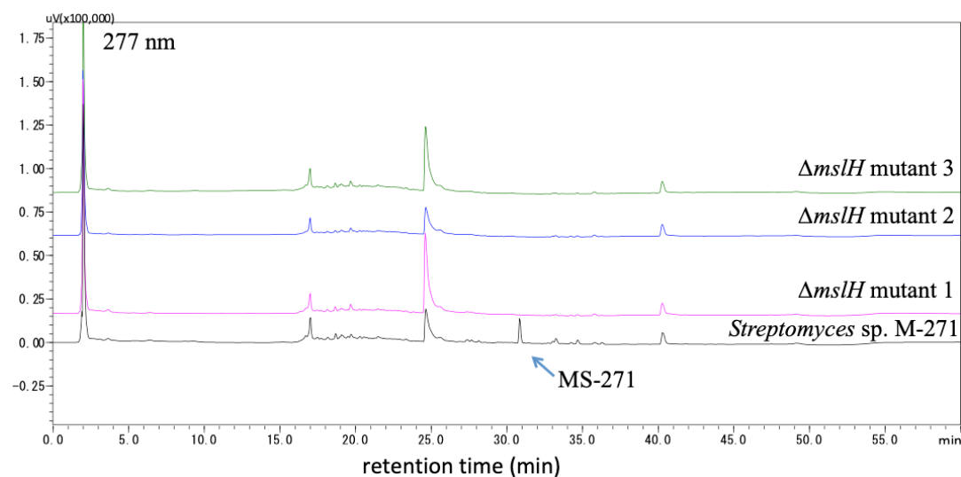
Figure 2-2-1-3. HPLC analysis of the extracts of three \Delta mslH mutants and wild type.
