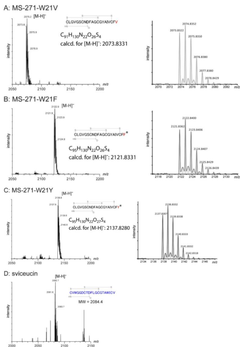
Figure 3-2-3-2 Mass spectra (ESI-negative, low-resolution [left] and high-resolution [right] data) of MS-271 derivatives: (A) MS-271-W21V, (B) MS-271-W21F, (C) MS-271-W21Y, (D) sviceucin, (E) svi-W, (F) svi-CFW, (G) svi-VCFW, and (H) svi-AIVCFW. D-Amino acid-containing products confirmed by chiral analysis are marked with an asterisk.
