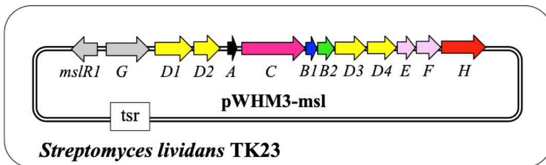
Figure 2-2-2-1 The plasmid containing the putative MS-271 cluster was expressed in S. lividans .
