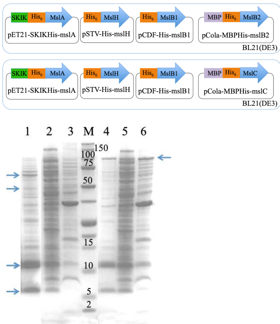
Figure 3-2-1-8 Plasmid sets and Tricine-SDS-PAGE analysis of recombinant proteins (MslA 5.8 kDa, MslH 49.1 kDa, MslB1 10.4 kDa and MslB2 64.5 kDa or MslC 109.8 kDa). 1, purified fractions of MslA, -H, -B1 and -B2 coexpression; 2, soluble fractions of MslA, -H, -B1 and -B2 coexpression; 3, insoluble fractions of MslA, -H, -B1 and -B2 coexpression; M, marker; 4, purified fraction of MslA, -H, -B1 and -C coexpression; 5, soluble fractions of MslA, -H, -B1 and -C coexpression; 6, insoluble fractions of MslA, -H, -B1 and -C coexpression.
