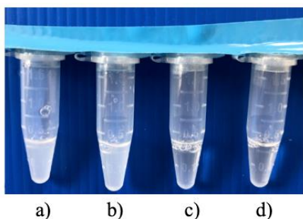
Figure 3-2-2-3 Left: LC-MS analysis (ESI negative ion mode, monitored at m/z 497) of in vitro assay. L-FDLA derivatives of Trp in MslA by in vitro reaction of a) mslA , b) mslA and mslB1 , c) mslA and mslH , d) mslA , mslB1 and mslH . Right: corresponding appearance of in vitro reactions.
