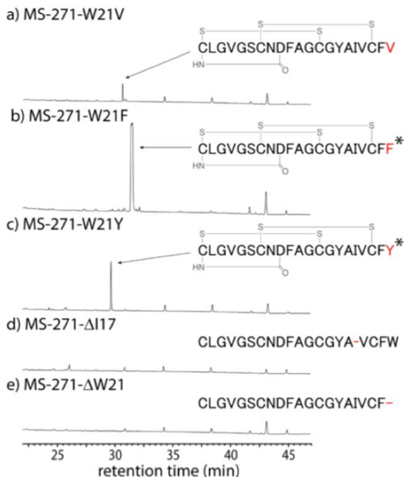
Figure 3-2-3-1 LC-MS analysis (UV absorbance monitored at 210 nm) of metabolites produced by heterologous production of the msl cluster with mslA mutant plasmids, a) pWHM3- msl -MS-271-W21V, b) pWHM3- msl -MS-271-W21F, c) pWHM3- msl -MS-271-W21Y, d) pWHM3- msl -MS-271-ΔI17, e) pWHM3- msl -MS-271-ΔW21, f) pWHM3- msl -svi, g) pWHM3- msl -svi-W, h) pWHM3- msl -svi-CFW, i) pWHM3- msl -svi-VCFW, and j) pWHM3- msl -svi-AIVCFW. The mutated amino acids in MS-271 derivative are shown in red. Sviveucin- and MS-271-derived sequences in the hybrid lasso peptides are shown in blue and red, respectively. The D-amino acid-containing products confirmed by chiral analysis are marked with an asterisk.
