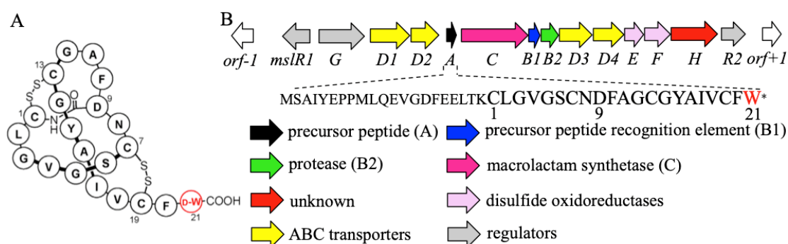
Figure 2-2-1-1 (A) Structure and (B) biosynthetic gene cluster ( msl ) of MS-271
