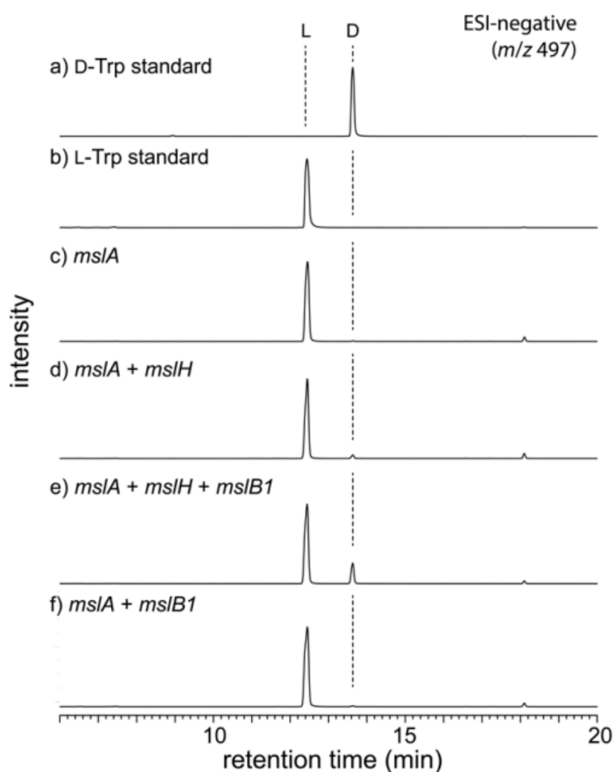
Figure 3-2-1-7 LC-MS analysis (ESI negative ion mode, monitored at m/z 497) of in vivo assay. L-FDLA derivatives of a) D-Trp standard and b) L-Trp standard. L-FDLA derivatives of Trp in MslA by heterologous expression of c) mslA alone, d) mslA and mslH , e) mslA , mslH , and mslB1 , and f) mslA and mslB1 .
