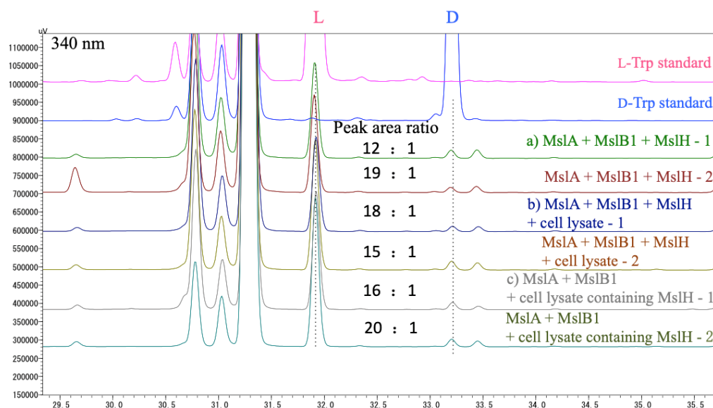
Figure 3-2-2-1 HPLC analysis of MslA, MslB1, MslH reaction with cell lysate. Each experiment was performed in duplicate.
