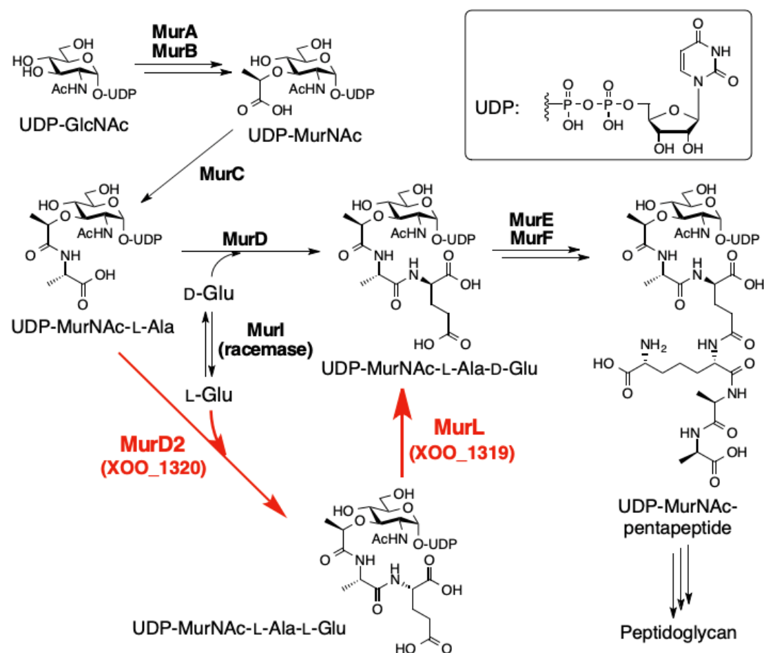
Figure 1-4-2. Peptidoglycan biosynthetic pathways of MurD/MurI and MurD2/MurL.
