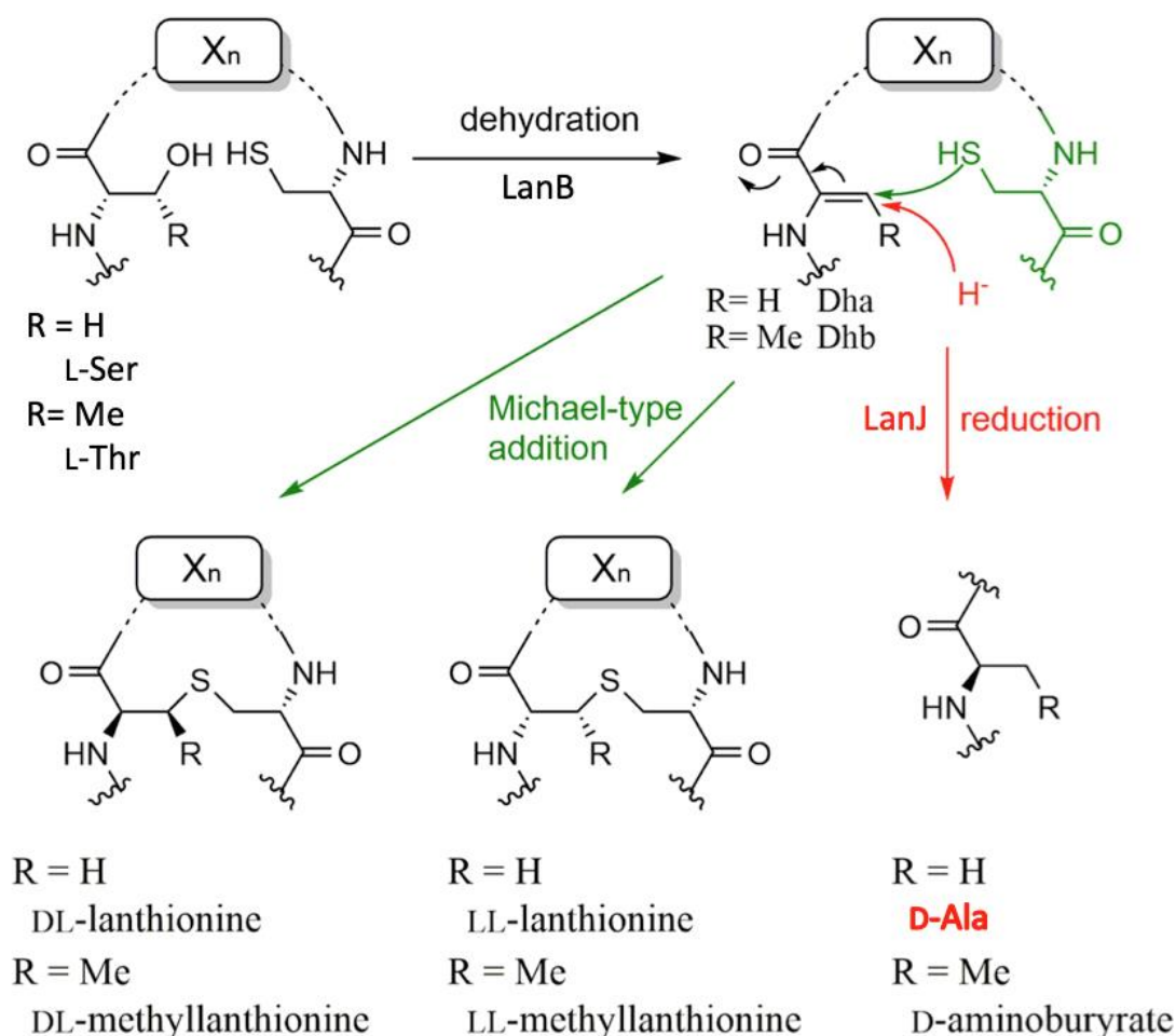
Figure 1-3-4. Formation of D-Ala in the maturation of lanthipeptides.
