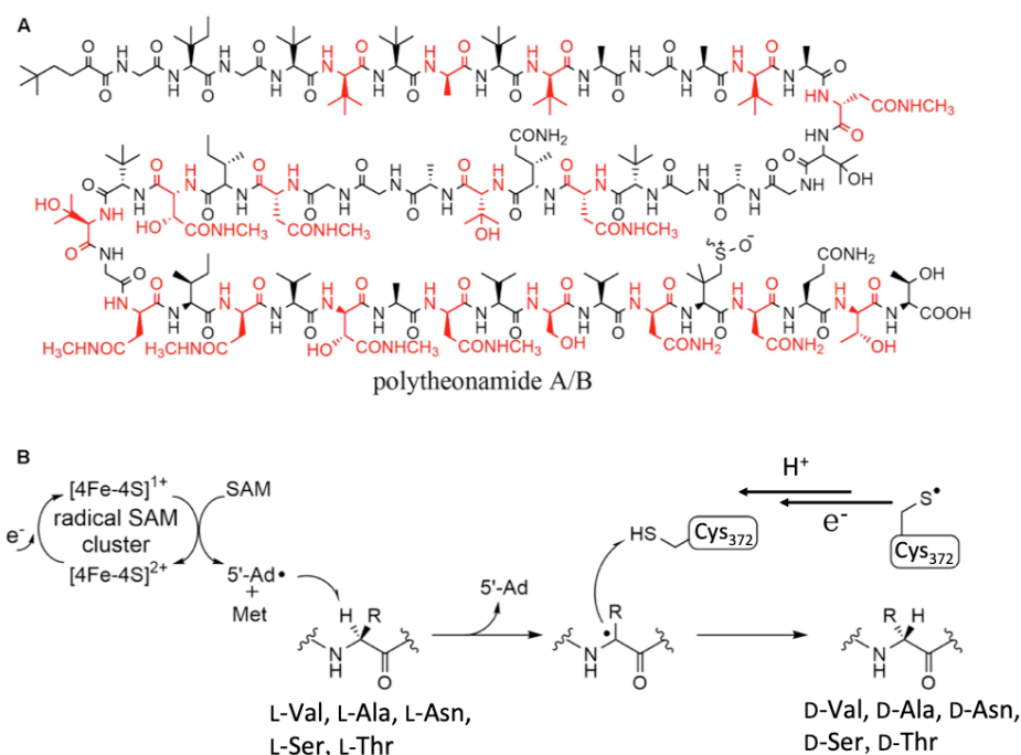
Figure 1-3-1 (A) structures of polytheonamides (A/B only differing in sulfoxide configuration). D-amino acids are shown in red. (B) proposed mechanism for the radical SAM peptide epimerase PoyD.
