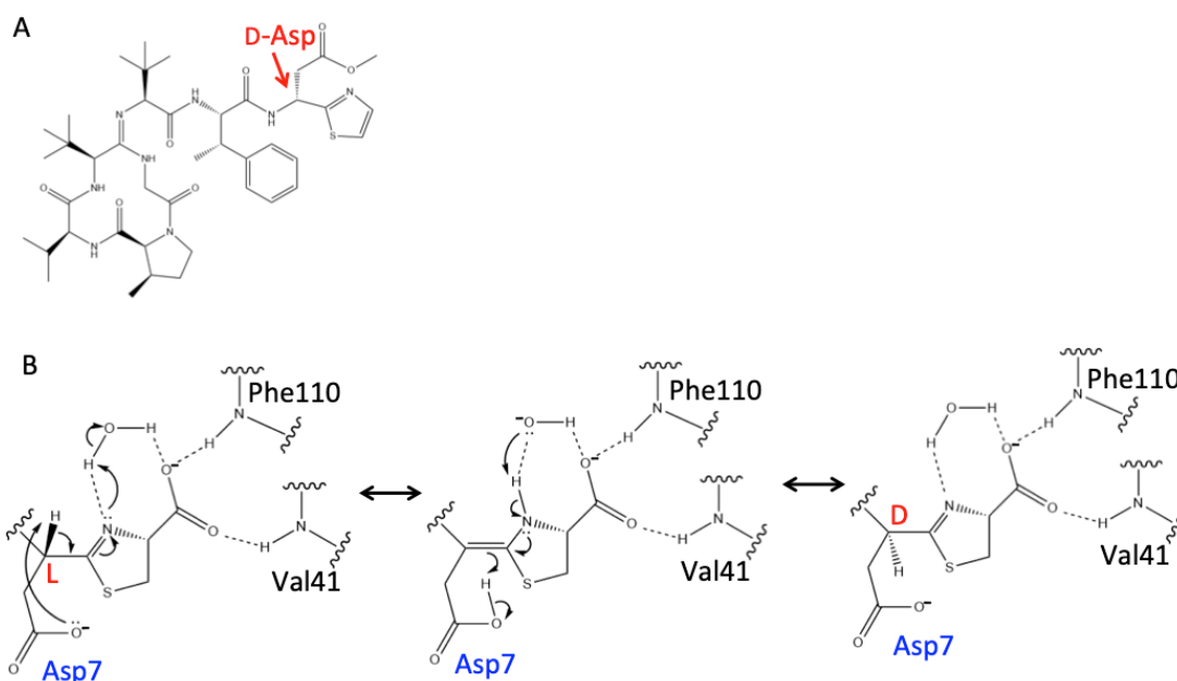
Figure 1-3-3. (A) D-Asp at position 7 in bottromycin A2
