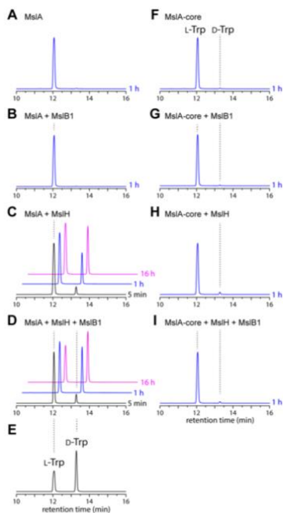
Figure 3-2-2-5 LC-MS analysis (ESI negative ion mode, monitored at m/z 497) of L- FDLA-Trp derived from in vitro reactions. The reaction time is shown next to each trace. (A) MslA only, (B) MslA + MslB1, (C) MslA + MslH, (D) MslA + MslH + MslB1, (E) L- and D-Trp standards, (F) MslA-core only, (G) MslA-core + MslB1, (H) MslA-core + MslH, and (I) MslA-core + MslH + MslB1.
