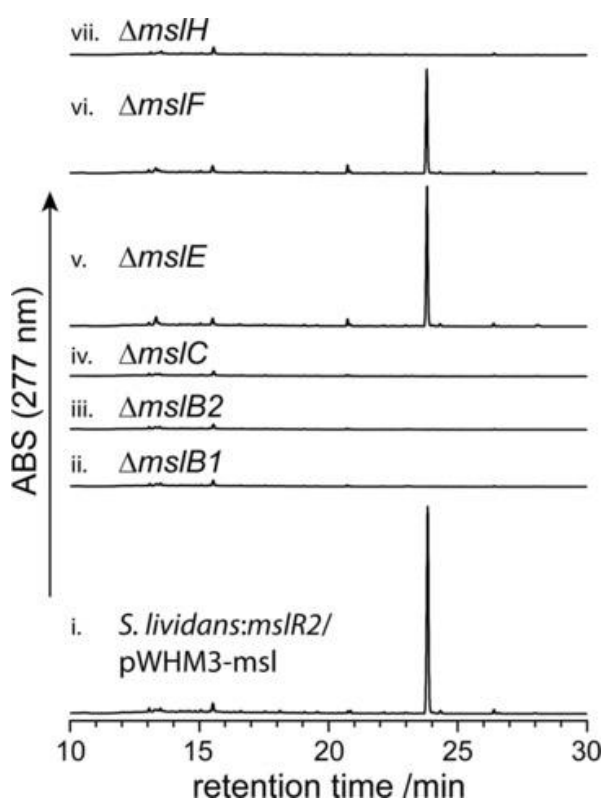
Figure 2-2-4-2 LC-MS analysis of metabolites produced by the mutants i) S. lividans : mslR2 /pWHM3- msl , ii) /pWHM3- msl - \Delta mslB1 , iii) /pWHM3- msl - \Delta mslB2 , iv) /pWHM3- msl - \Delta mslC , v) /pWHM3- msl - \Delta mslE , vi) /pWHM3- msl - \Delta mslF , and vii) /pWHM3- msl - \Delta mslH .
