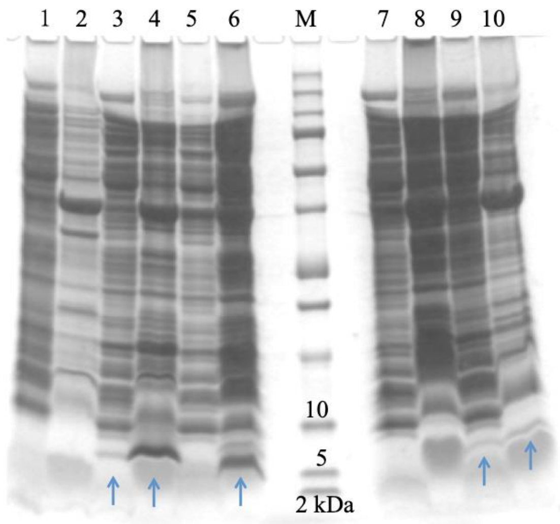
Figure 3-2-1-3 Tricine-SDS-PAGE analysis of recombinant MslA. Soluble fractions of E. coli BL21(DE3) harboring (1) empty pET24b as a control; (3) pET24-SKIKHis-mslA; (5) pET24-SKIK-mslA; (7) pRSF-SKIK-mslA; (9) pRSF-SKIKHis-MslA. Insoluble fractions of E. coli BL21(DE3) harboring (2) empty pET24b as a control; (4) pET24-SKIKHis-mslA; (6) pET24-SKIK-mslA; (8) pRSF-SKIK-mslA; (10) pRSF-SKIKHis-mslA. M, marker. After IPTG was added, induction was performed at 16 °C overnight.
