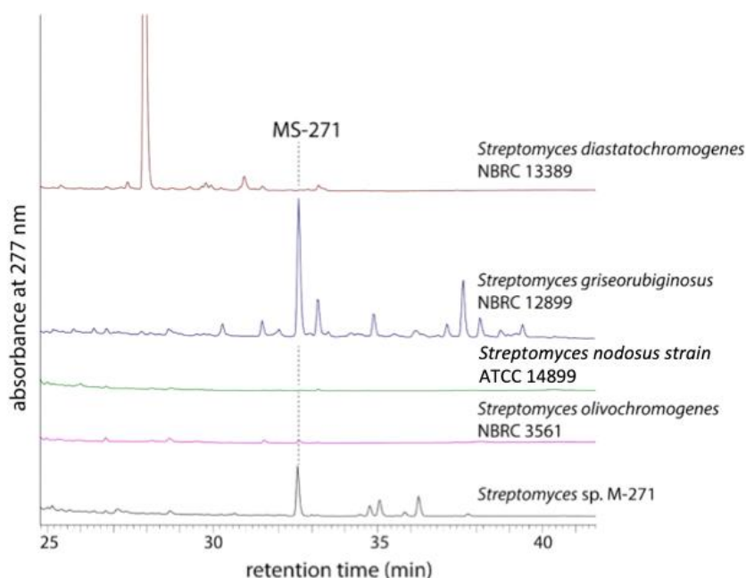
Figure 3-2-1-2 Production of MS-271 by Streptomyces strains harboring msl -like gene clusters.
