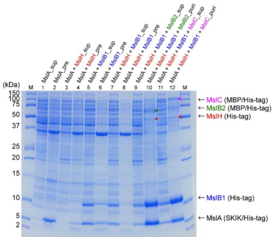
Figure 3-2-1-10 Tricine-SDS-PAGE analysis of recombinant MslA (5.8 kDa), MslB1 (10.4 kDa), MslH (49 kDa), MslB2 (65 kDa), and MslC (110 kDa) in in vivo expressions. The odd and even lane numbers show supernatant (sup) and precipitate (pre) fractions of cell extracts of the transformants expressing MslA (Lanes 1 and 2),
