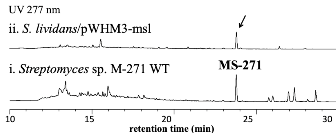
Figure 2-2-2-2 LC-MS analysis of products accumulated in the cultures. i) Streptomyces sp. M-271 wild type. ii) S. lividans /pWHM3-msl.
