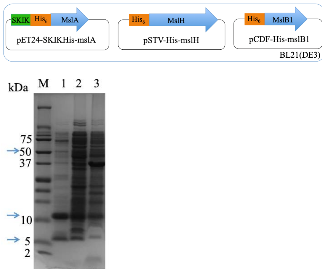
Figure 3-2-1-6 Plasmid set and Tricine-SDS-PAGE analysis of recombinant MslA (5.8 kDa), MslH (49.1 kDa) and MslB1 (10.4 kDa). M, marker; 1, purified His-tagged MslA, MslH and MslB1; 2, soluble fractions; 3, insoluble fractions.
