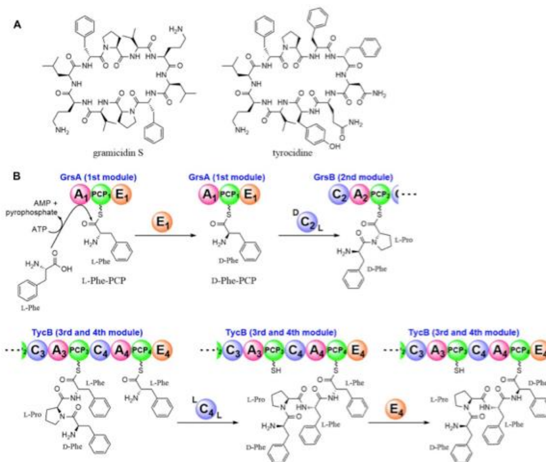
Figure 1-4-3. Epimerization by NRPS.
