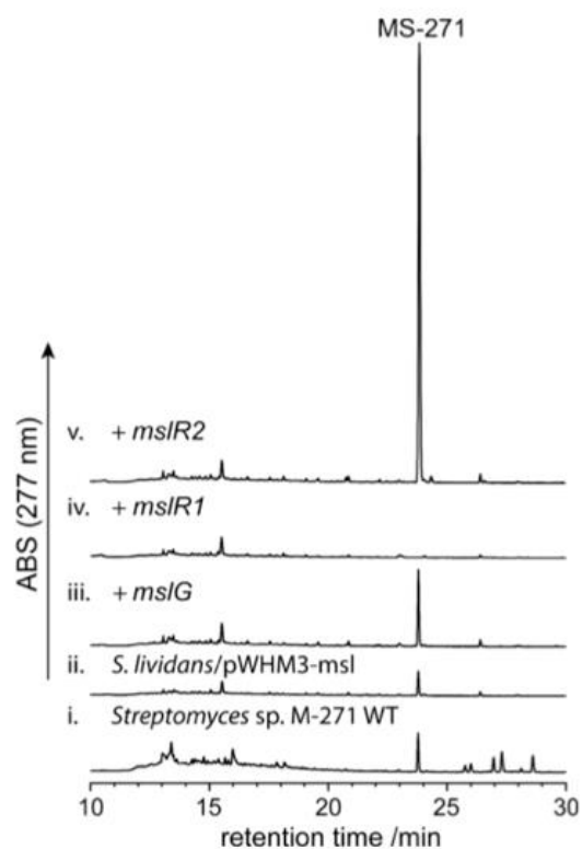
Figure 2-2-3-2 LC-MS analysis of products accumulated in the cultures. i) Streptomyces sp. M-271 wild type, ii) S. lividans /pWHM3- msl . iii) S. lividans:mslG /pWHM3- msl , iv) S. lividans:mslR1 /pWHM3- msl , v) S. lividans:mslR2 /pWHM3- msl .
