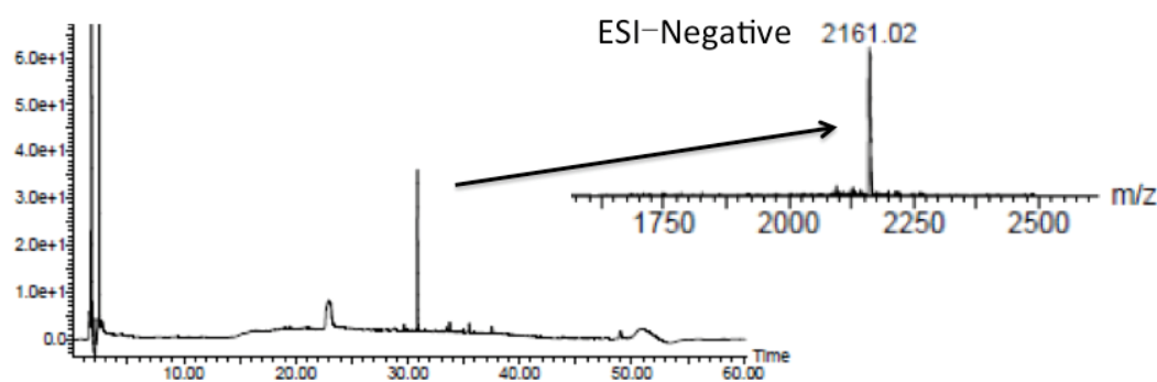
Figure 2-2-1-4. LC-MS analysis of compound in the peak with a RT at 30.8 min.
