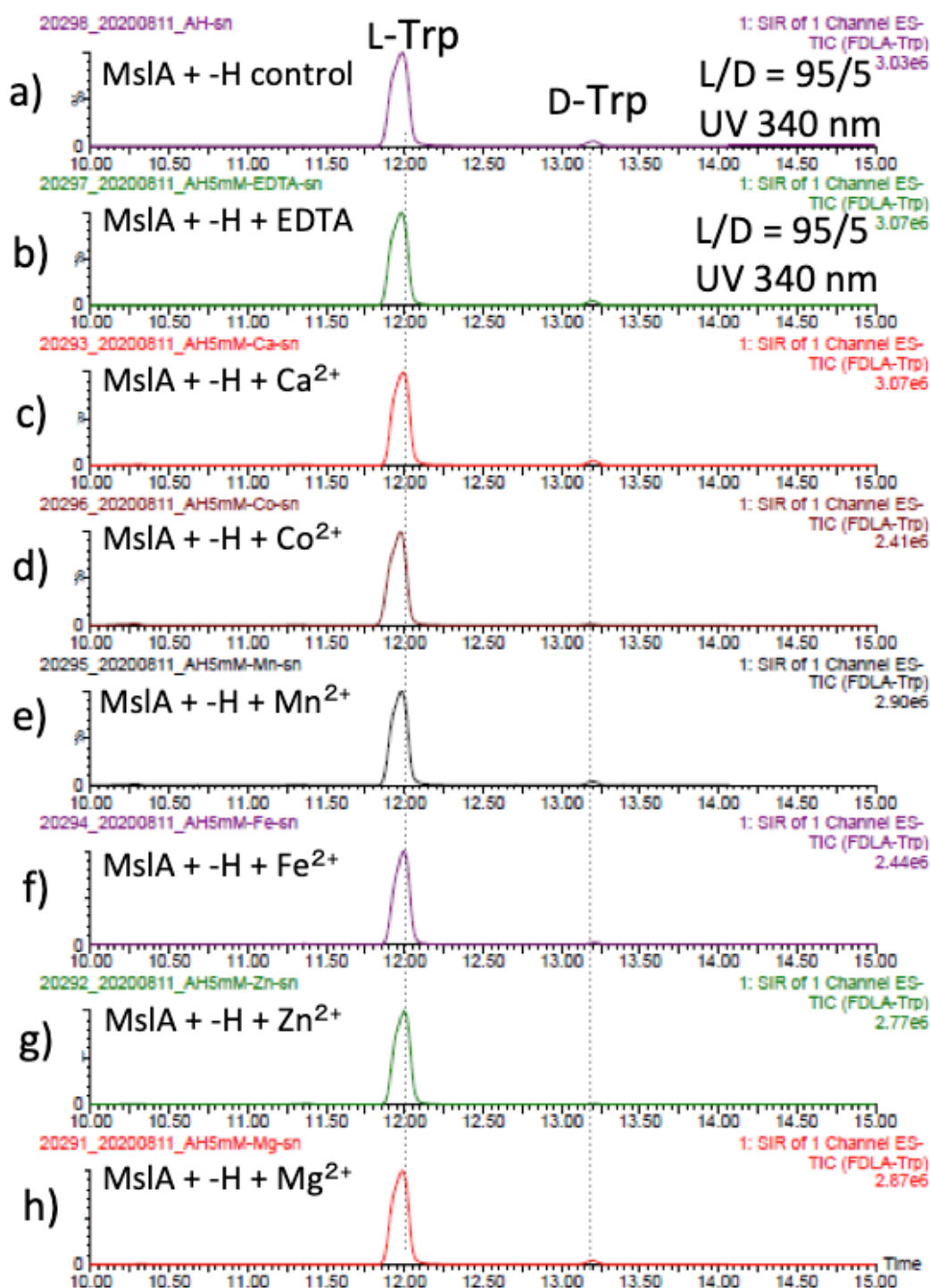
Figure 3-2-2-7 LC-MS analysis (ESI negative ion mode, monitored at m/z 497) of in vitro assay. L-FDLA derivatives of Trp in MslA by in vitro reaction of MslH further supplemented with b) EDTA, c) \text{Ca}^{2+} , d) \text{Co}^{2+} , e) \text{Mn}^{2+} , f) \text{Fe}^{2+} , g) \text{Zn}^{2+} , h) \text{Mg}^{2+} . a) is a control experiment.
