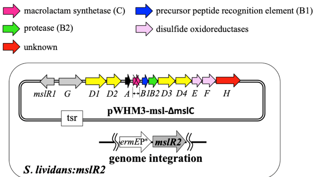
Figure 2-2-4-1 S. lividans : m slR2 harboring an in-frame deletion plasmid lacking one of modification enzyme genes.
