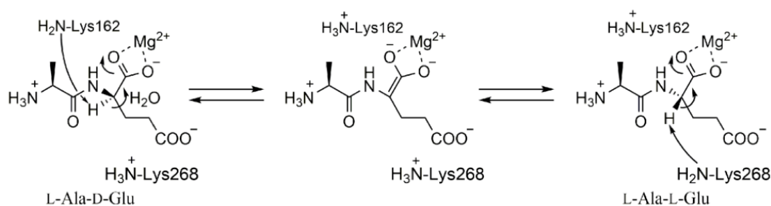
Figure 1-4-1. Reaction of L-Ala-D/L-Glu epimerases.
