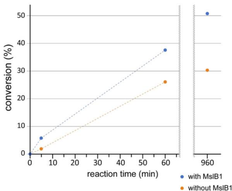
Figure 3-2-2-6 Plot of reaction time (5 min, 60 min, and 16 h) versus conversion from MslA to its epimer by MslH reaction in the presence and absence of MslB1. The conversion (%) was calculated based on the peak area of chromatograms of UV absorbance monitored at 340 nm.
