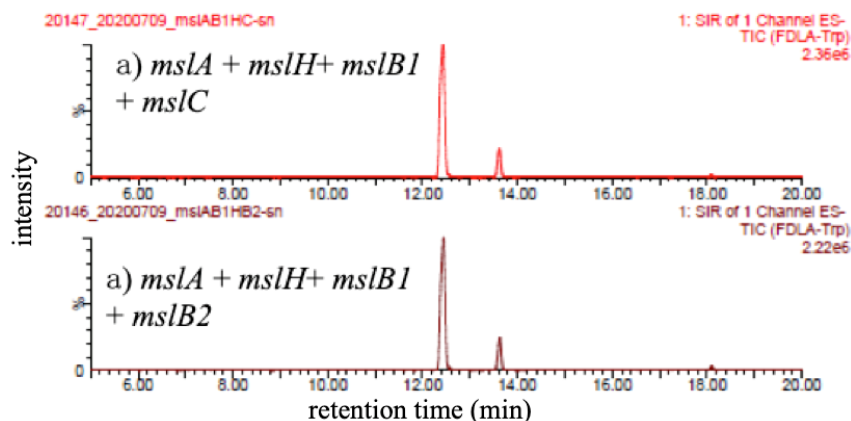
Figure 3-2-1-9 LC-MS analysis (ESI negative ion mode, monitored at m/z 497) of in vivo assay. L-FDLA derivatives of Trp in MslA by heterologous expression of a) mslA , mslH , mslB1 and mslC , and b) mslA , mslH , mslB1 and mslB2 .
