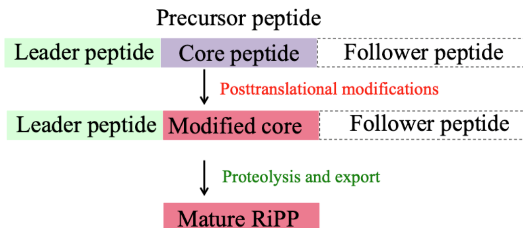
Figure 1-1-1. General biosynthetic pathway for RiPPs.
