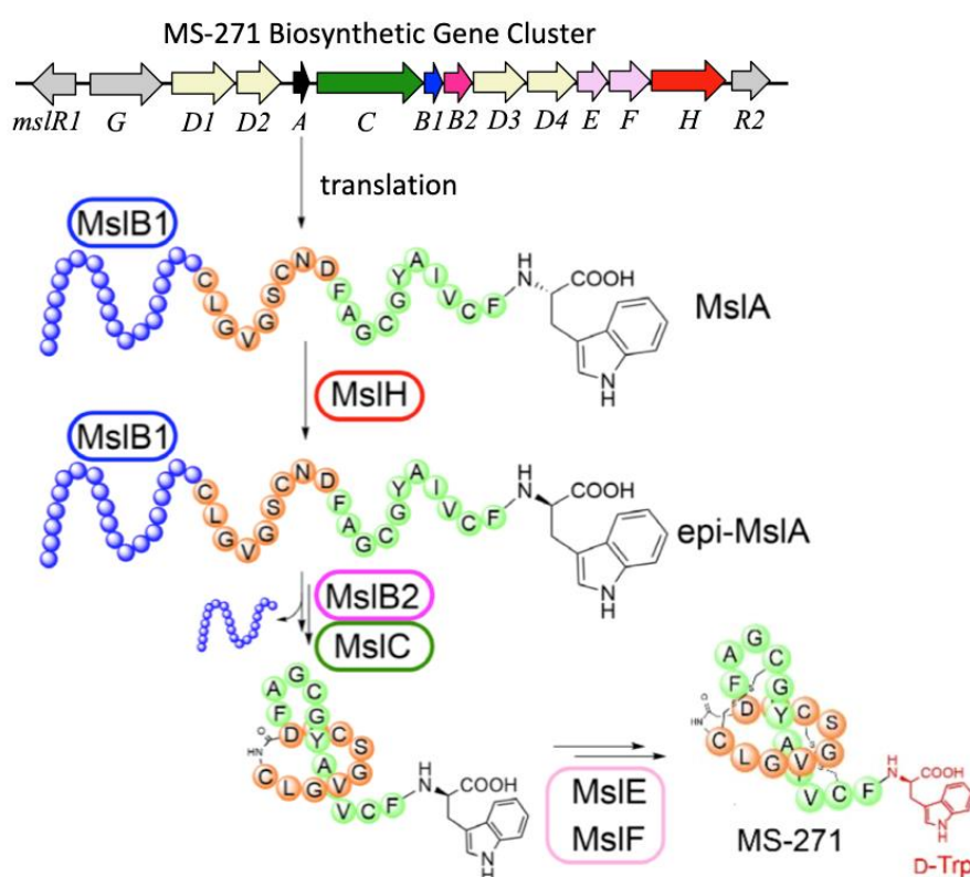
Figure 3-3-1 Biosynthesis of MS-271. MslB1 tightly binds to the leader peptide region (blue) in MslA and enhances the MslH reaction.
