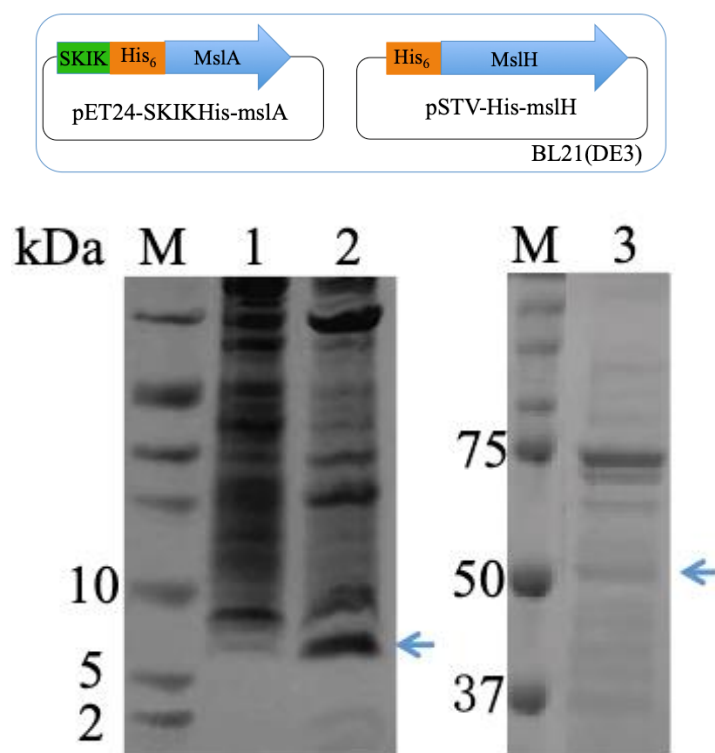
Figure 3-2-1-5 Plasmid set and Tricine-SDS-PAGE analysis of recombinant MslA and MslH. 1, soluble fractions; 2, insoluble fractions containing MslA (5.8 kDa); 3, purified MslH (49.1 kDa) with a low purity.
