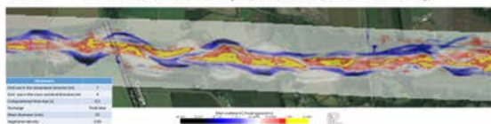
Figure 12 Contour map of elevation change by computation (after series of flooding)
