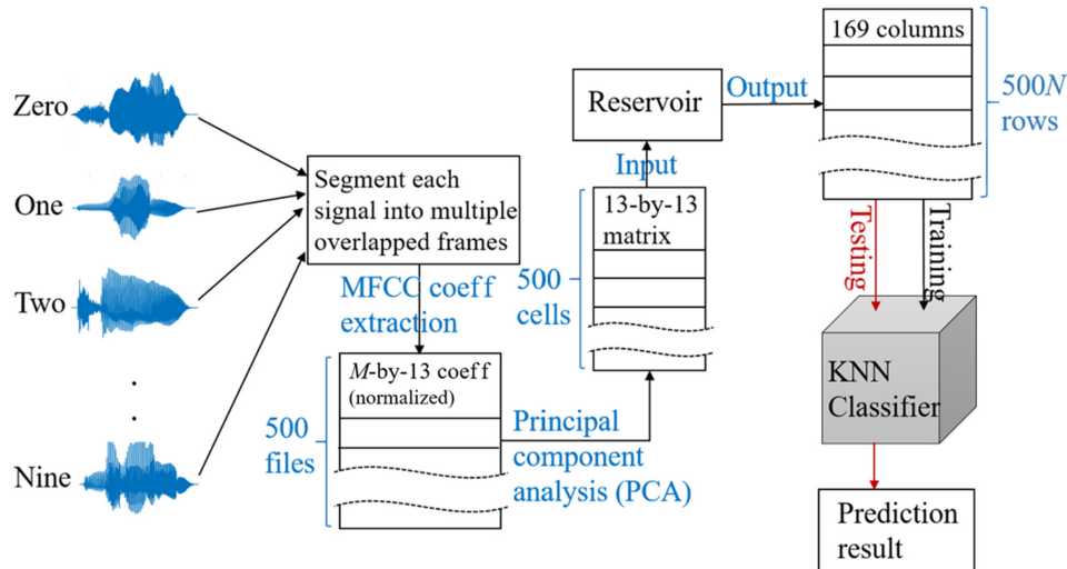
FIG. 10. Schematic of the isolated-word recognition process. M \times 13 features are extracted separately for each of the 500 audio signals, where M is the number of segmented frames. After principal component analysis, all coefficient matrixes with different sizes are organized into the same size of 13 \times 13 (i.e., 169 coefficients) for one speech sample. Reservoir of N nodes would give a reservoir state of 500 \times 169 \times N data items. We rearrange the reservoir state into 500 cells (each given the same label) and use them for training and testing sets. Detailed description of this classification process is given in Fig. 11.
