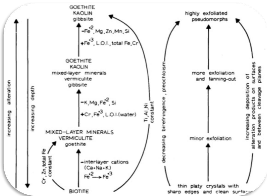
Figure 4. 4. Pathways for biotite alteration deduced from morphological, mineralogical, and chemical studies of specimens from deeply weathered profiles (From Gilkes and Suddhiprakarn, 1979)
