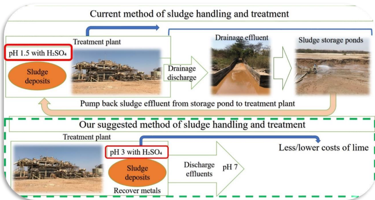
Fig. 6.8. Metal recovery from sludge through acid treatment
