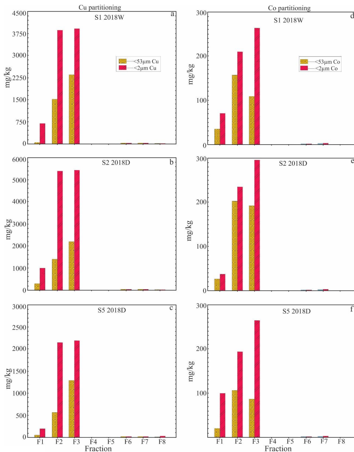
Figure 4. 9. Sequential extraction results of solid sludge. For individual fraction phases, refer to Table 7 and for sample location, refer to Fig. 3.3b and Table 8.
