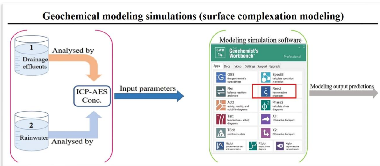
Fig. 6.1: Surface complexation model simulation for predicting optimal pH of wastewater treatment and metal stability conditions by rainwater percolations
