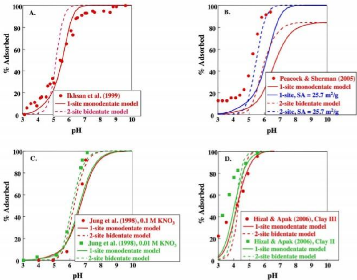
Figure 2. 6. Comparisons 1-site and 2-site kaolinite models with previously reported data. The 1-site model includes a monodentate Cu complex on a variable charge site. The 2-site model includes a bidentate Cu complex on a variable charge site and an ion exchange site that does not bind Cu (Lund et al., 2008)
