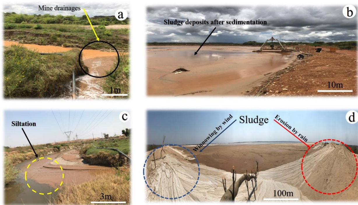
Fig.1.1.1. a) Mine drainage; b) sludge storage site; c) drainage siltation by sludge effluents from mining sources; d) sludge solid surface erosion by rainfall or winnowing by wind
