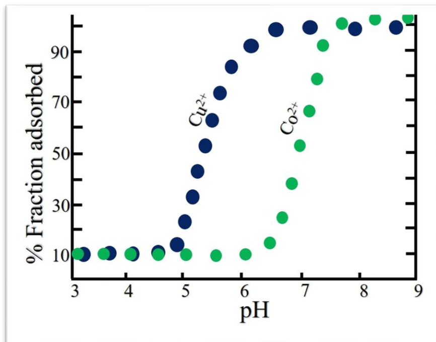
Fig. 5.6. Batch adsorption experiment results of binary system of \text{Cu}^{2+} and \text{Co}^{2+} onto kaolinite in sludge
