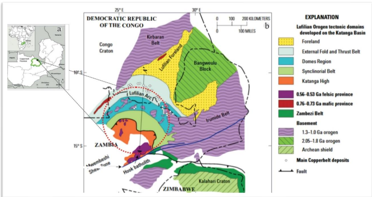
Figure 3.1. Regional setting of the Zambian Copperbelt (McGowan et al., 2006)
