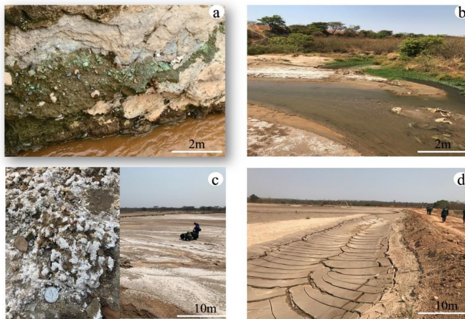
Fig. 3.6. a) Malachite precipitates along drainage; b-c) efflorescent salts precipitates along drainage and ponds; d) mud cracks formation at storage ponds
