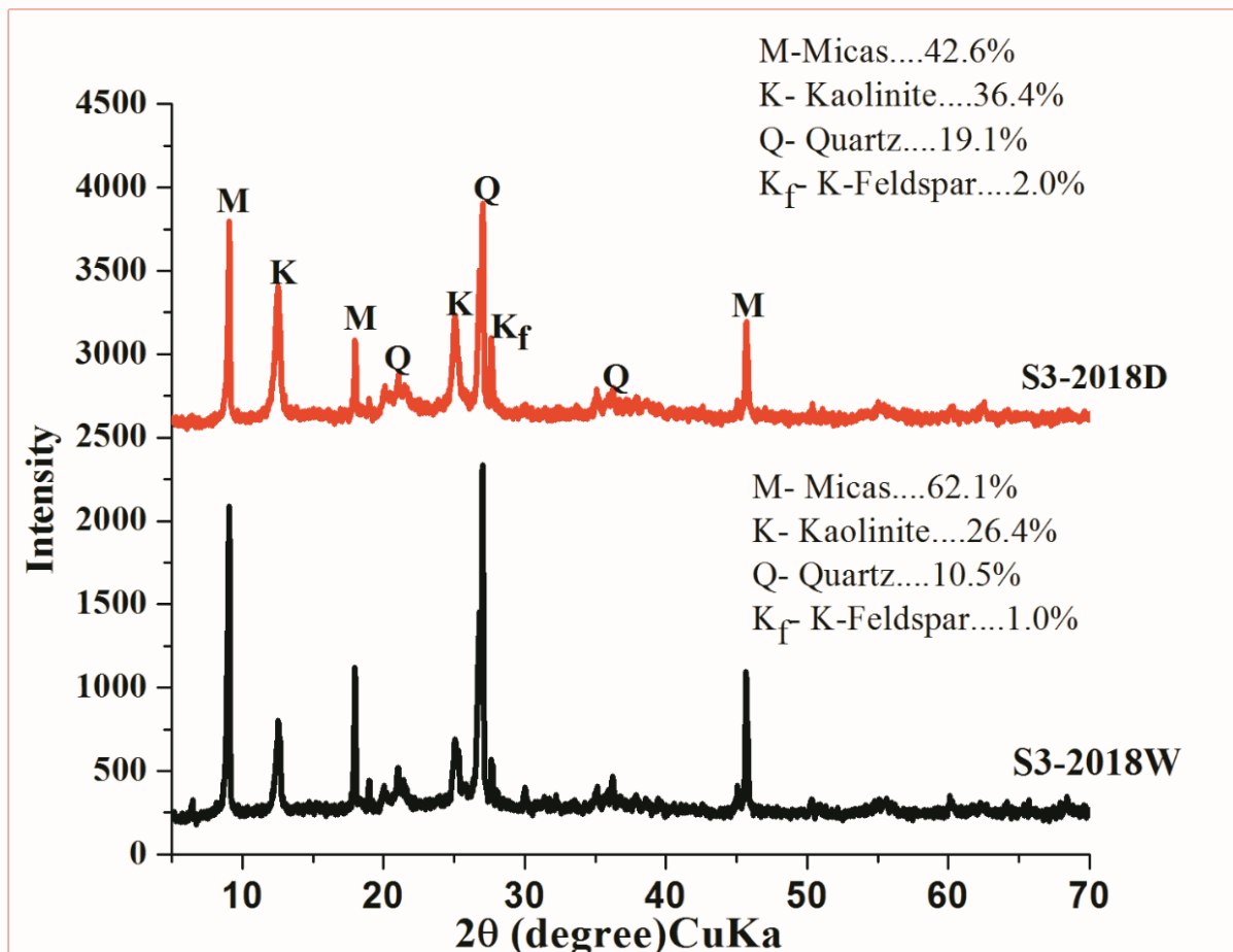
Figure 4. 3. XRD patterns of sludge
