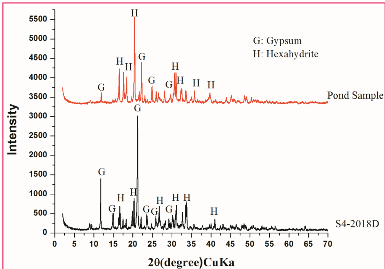
Figure 4. 8. XRD patterns of gypsum and hexahydrate formed during dry season and devoid of metals due to adsorption processes in sludge associated with the host minerals such as HFO and kaolinite which bind the metals making them not easily releasable during salt precipitations
