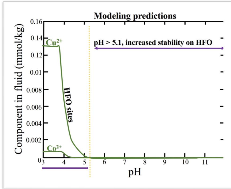
Fig. 6.7. Optimal pH of \text{Cu}^{2+} and \text{Co}^{2+} ions stability onto HFO surface
