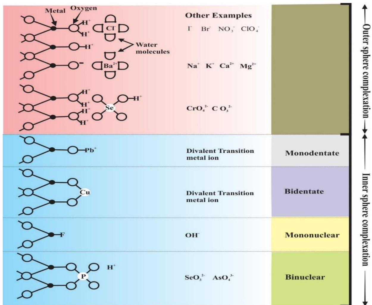
Figure 2. 3. Adsorption mechanisms and types of binding species (modified after Hayes, 1987)
