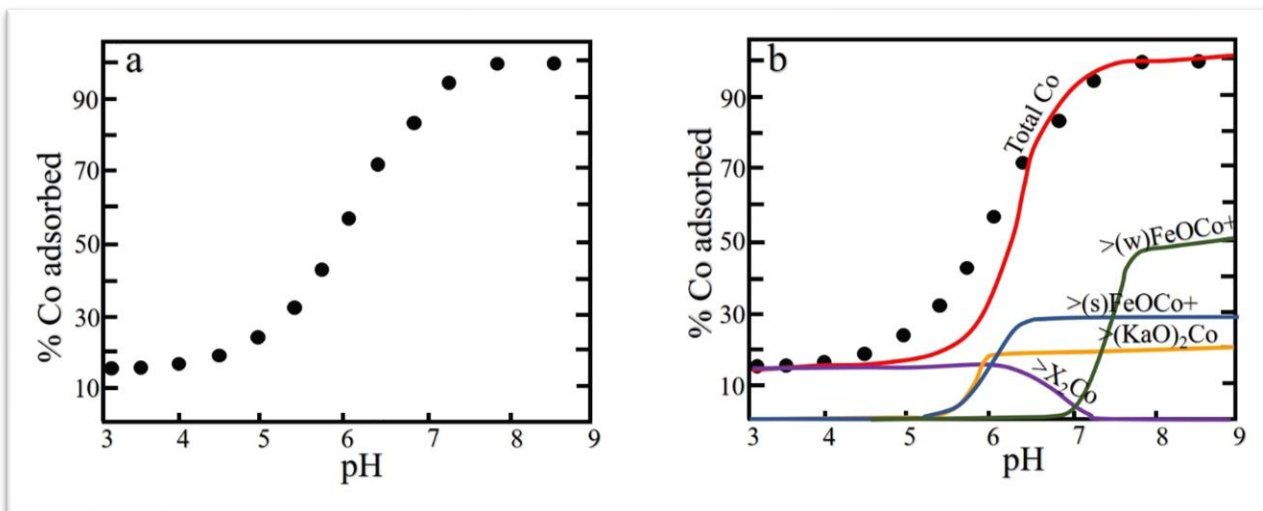
Fig. 5.5. Single system Co^{2+} adsorption onto mixture of kaolinite + HFO in sludge: a) Batch Co^{2+} adsorption behaviour; b) SCM prediction of surface species of Co^{2+} adsorption onto sludge mixture
