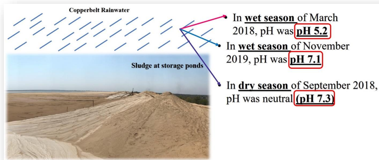
Fig. 6.5. Assessment of metal stability conditions through rainwater percolation onto sludges
