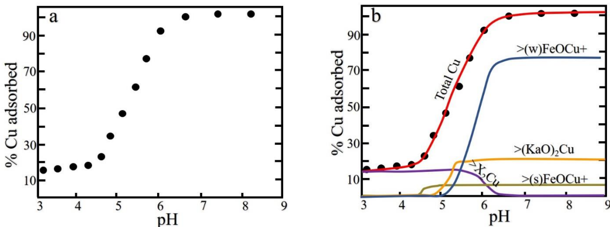
Fig. 5.4. Single system Cu 2+ adsorption onto mixture of kaolinite + HFO in sludge: a) Batch Cu 2+ adsorption behaviour; b) SCM prediction of surface species of Cu 2+ adsorption onto sludge mixture
