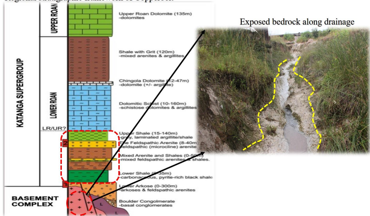
Figure 3.2. Regional stratigraphy of the Zambian Copperbelt (modified after Rainaud et al., 2005)
