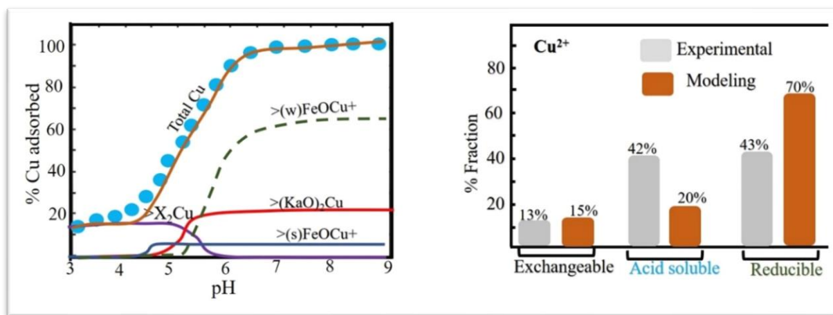
Fig. 5.8. Interpretation of sequential extraction from SCM predictions of \text{Cu}^{2+} species onto sludge with HFO (i.e., kaolinite + HFO)
