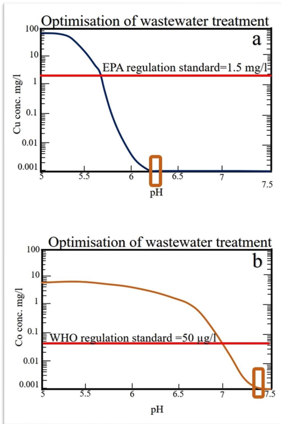
Fig. 6.3. SCM prediction of wastewater treatment optimisation; a) \text{Cu}^{2+} ions and b) \text{Co}^{2+} ions
