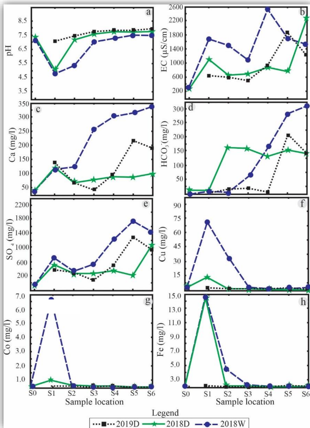
Figure 4. 1. Hydrogeochemical data of sludge effluents; (a) pH; (b) EC; (c) Ca 2+ ; (d) HCO 3 - ; (e) SO 4 2- ; (f) Cu 2+ ; (g) Co 2+ ; (h) Fe 2+ . Abbreviations: 2018D, 2019D, 2018W are sampling dates (i.e., in Years) and seasons (W-wet season) and (D-dry season). S1 – S6 are drainage sample location (refer to Fig. 1b).
