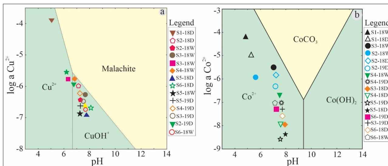
Figure 4. 2. Metals solubility diagrams plotted as a function of pH at 25°C of: (a) Cu and (b) Co. Abbreviation of symbols; S1 – S6 are sampled location (refer to Fig. 1b); 18W, D and 19D are sampling dates (i.e., in Years) and seasons (e.g., - wet season) and (e.g., D-dry season).
