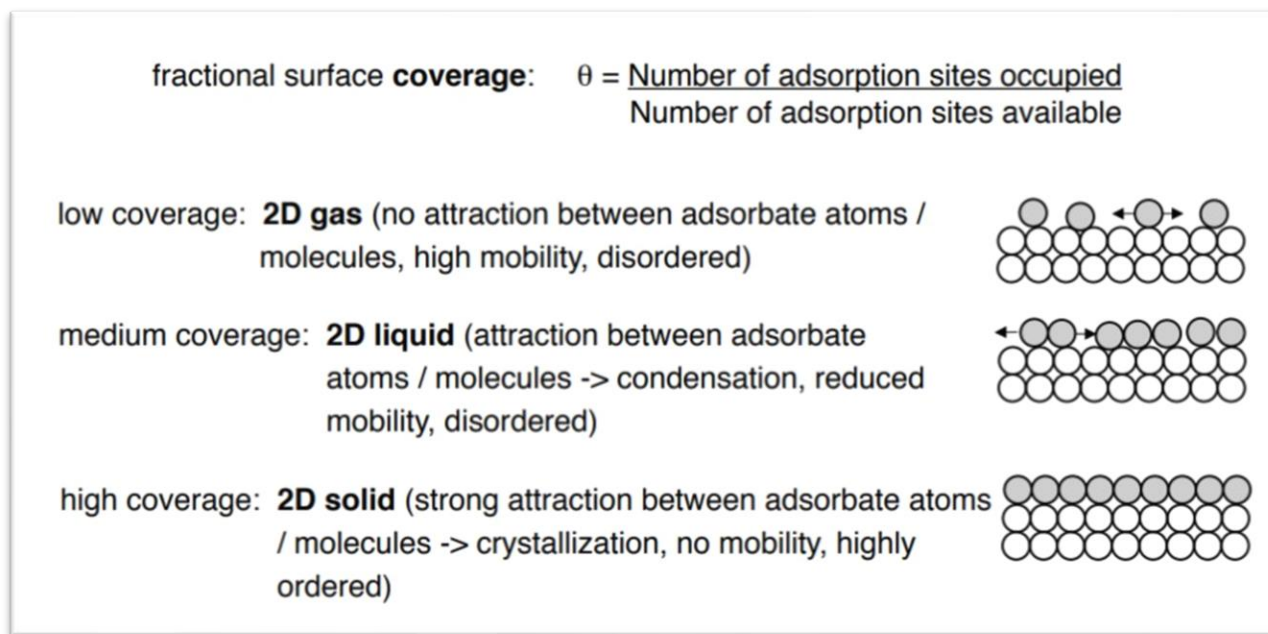
Figure 2. 4. Description of adsorption properties of metal adsorption. Courtesy of Prof. Dr Ulrich Jonas; Macromolecular chemistry- University of Siegen
