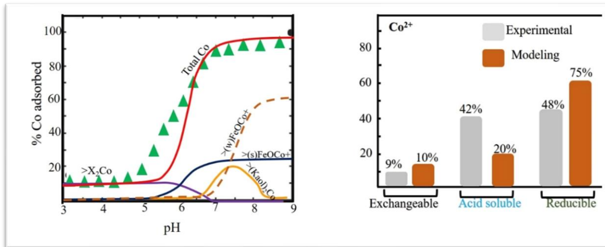
Fig. 5.9. Interpretation of sequential extraction from SCM predictions of \text{Co}^{2+} species onto sludge with HFO (i.e., kaolinite + HFO)
