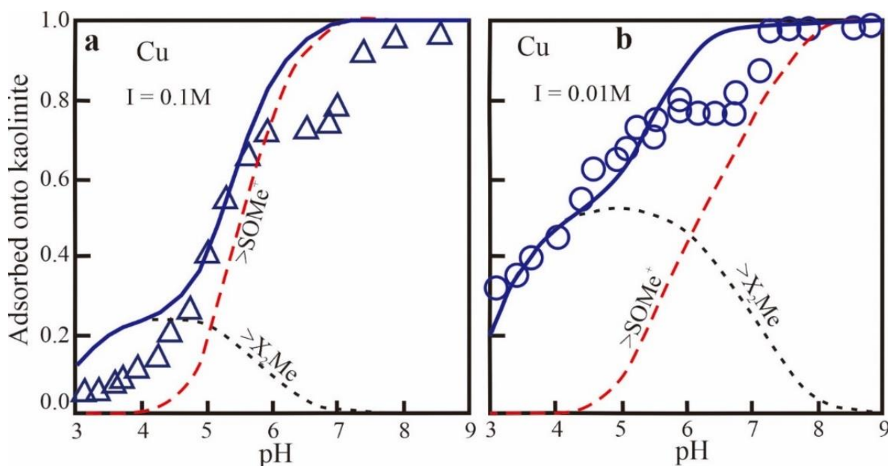
Figure 2. 5. The distribution of modeled surface complexation species of Cu (II) onto kaolinite at different ionic strengths (Modified from Gu and Evan, 2008).
