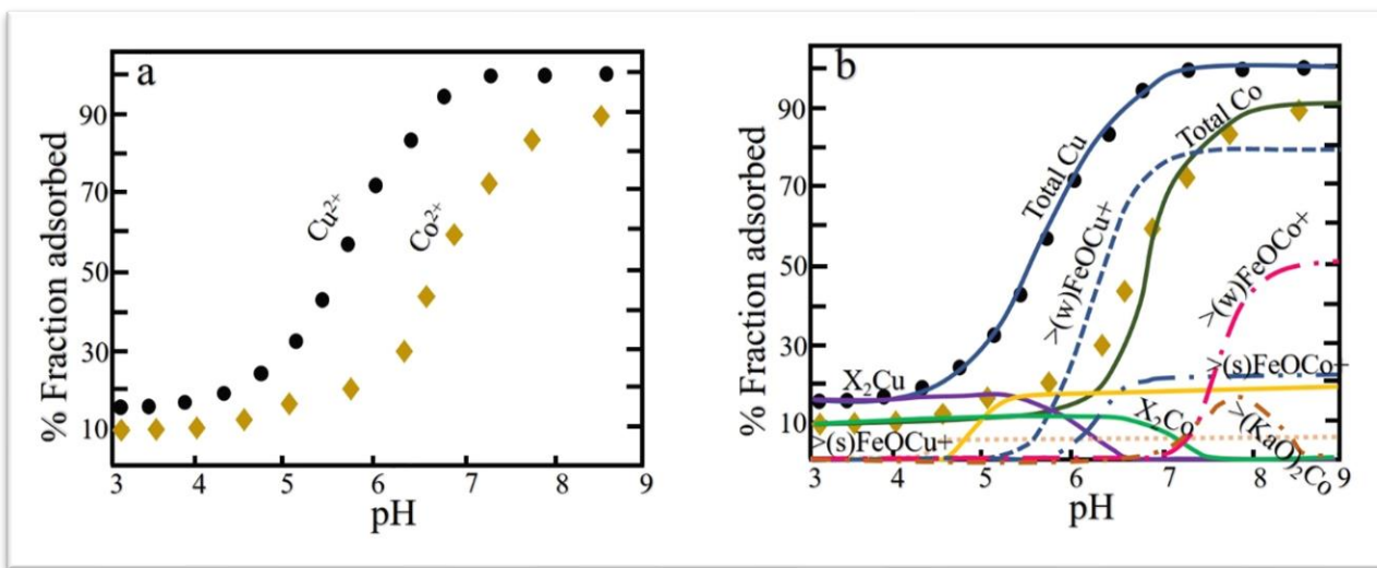
Figure 5.7. a) Batch adsorption results of binary system of Cu^{2+} and Co^{2+} onto sludge containing kaolinite and HFO; b) SCM prediction of surfaces species Model parameters for kaolinite are listed in Table 10 and HFO from Dzombak and Morel (1990). Experimental data (dots) and solid line and dotted lines are kaolinite and HFO predictions. Experiment conducted at 0.05M ionic strength.
