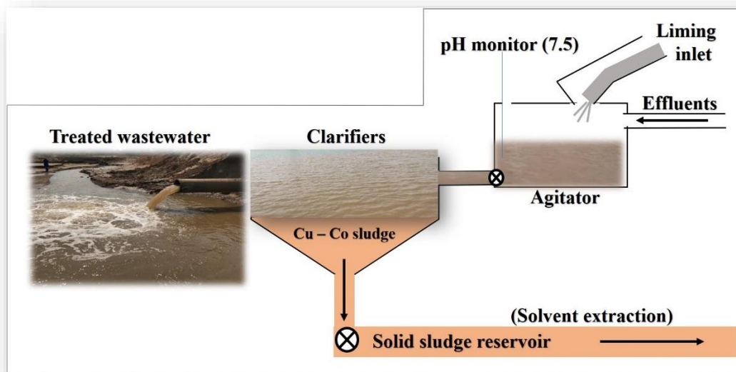
Fig. 6.4. Proposed wastewater treatment optimisation at the mine site
