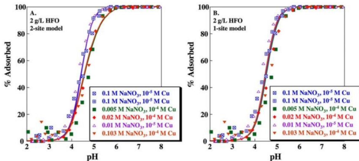
Figure 2. 8. Cu adsorption as a function of pH on HFO. Solid concentration is 2 g/L. Lines indicate fits for (A) Dzombak and Morel (1990), 2-site HFO model and (B) Sverjensky and Sahai (1996), 1-site HFO model calculated using parameters shown in Tables 4 and 5
