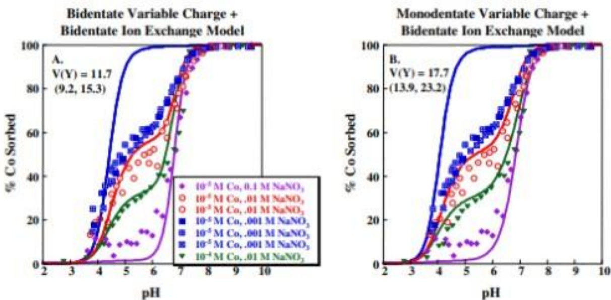
Figure 2. 7. Co sorption as a function of pH on 5 g/L Wards kaolinite with 104 or 105 M Co and 0.1–0.001 M NaNO 3 . Lines indicate fits predicted for models calibrated using KGa-1b data with an ion exchange site and (A) a bidentate Co complex on the variable charge site or (B) a monodentate Co complex on the variable charge site (Landry et al., 2009)
