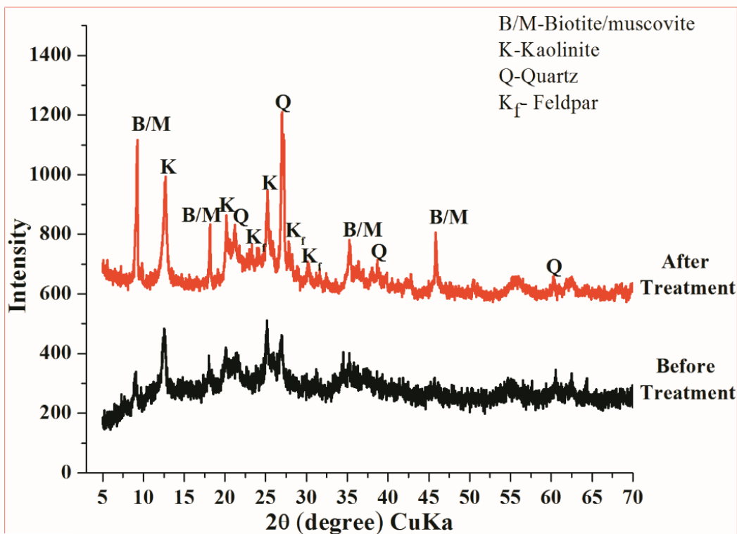
Figure 4. 6. XRD pattern of surface coated sludge before and after treatment. The coating material is HFO precipitate from the weathering of biotite
