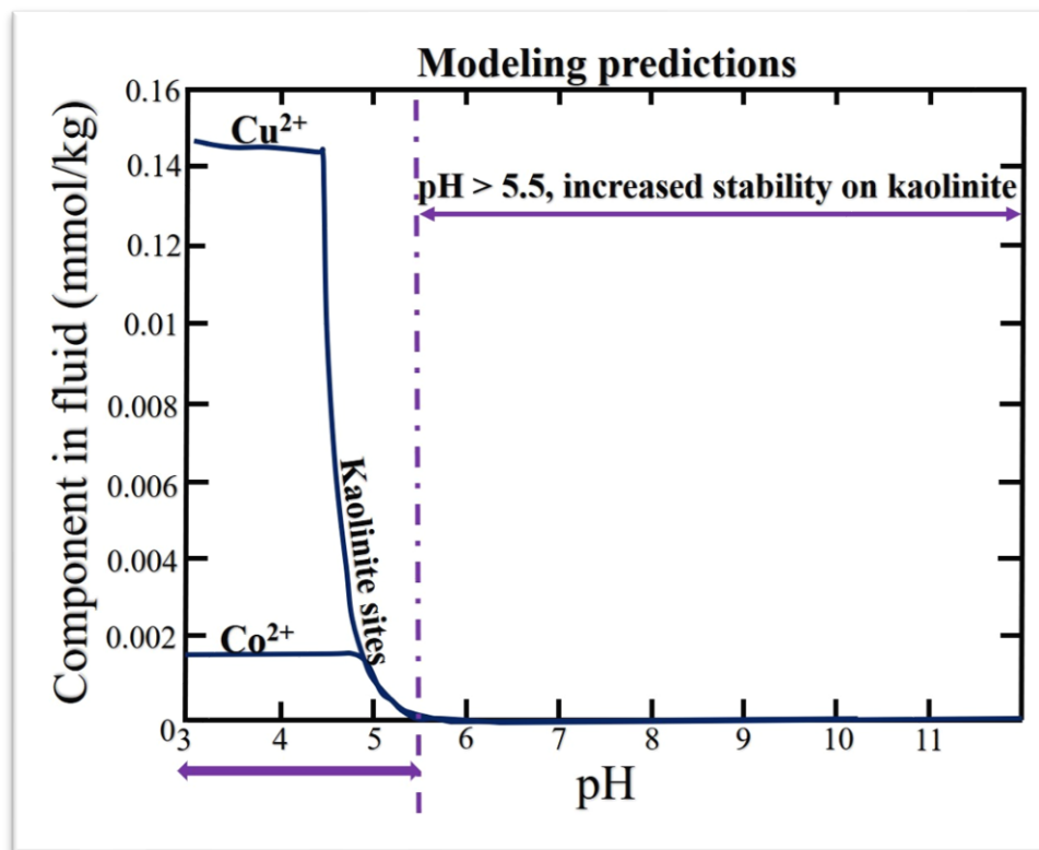
Fig. 6.6. Optimal pH of \text{Cu}^{2+} and \text{Co}^{2+} ion stability onto kaolinite surfaces
