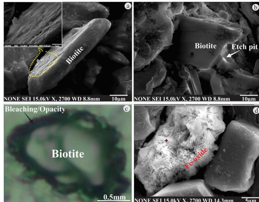
Figure 4. 5. (a) Exfoliation layers formed by the layered weathering of biotite grains, (b) Etched pits formed by edge weathering of biotite grains, (c) Bleaching and opacity of biotite grain surfaces due to coatings with non-crystalline material (i.e., HFO) during and after biotite weathering, (d) HFO precipitate formation from oxidations of \text{Fe}^{2+}/\text{Fe}^{3+} ions released from biotite weathering. Abbreviations: HFO-hydrous ferric oxide
