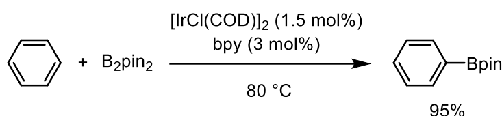
Scheme 15. Ishiyama-Miyaura-Hartwig borylation
