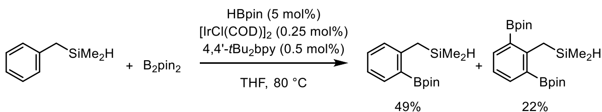
Scheme 16. Silyl-directed Ir-catalyzed ortho -borylation
