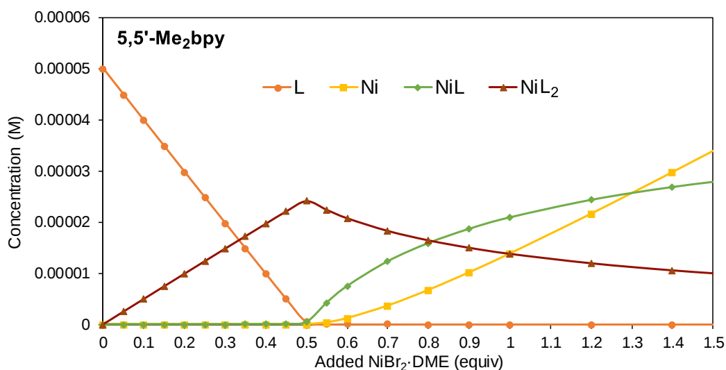
Figure 22. Concentration profiles with 5,5'-Me 2 bpy (without NiL 3 ). \Delta G_1 = -47.88 kJ/mol, \Delta G_2 = -45.83 kJ/mol, R^2 = 0.99874 .
