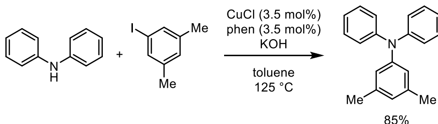
Scheme 2. Cu-phen catalyzed Ullmann coupling
