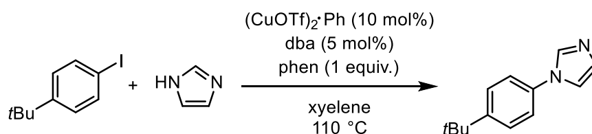
Scheme 3. Cu-catalyzed coupling of aryl halides and imidazoles
