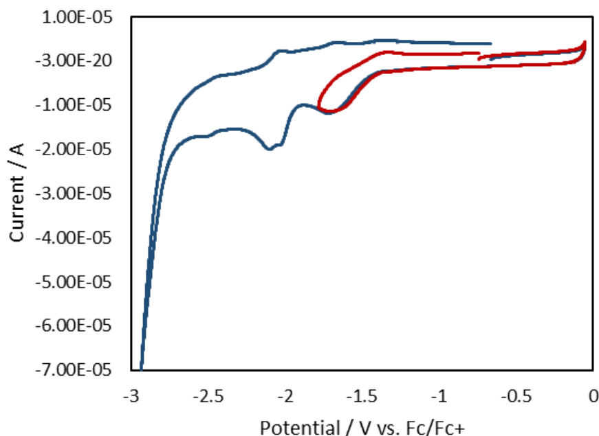
Figure 15. CV of a 100 mM nBu 4 NBr in DMA solution containing 1.0 mM NiBr 2 ·DME and 1.0 mM L5 (completely dissolved). The scan rate was \nu = 0.1 \text{ V s}^{-1} .
