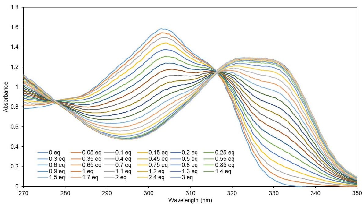
Figure 29. Absorption data for the titration test between L3 and \text{NiBr}_2 \cdot \text{DME} in DMA
