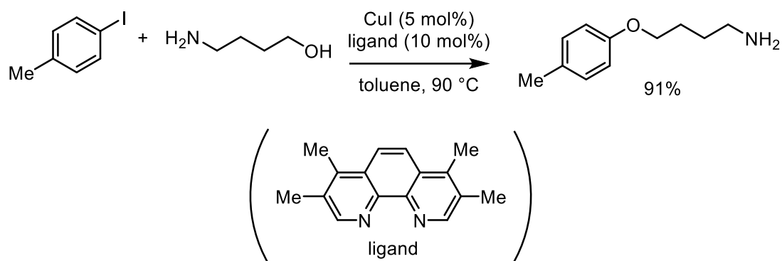
Scheme 4. Cu-catalyzed O-arylation of amino alcohols
