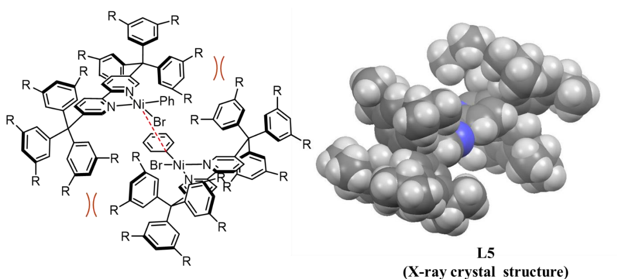
Figure 10. Bimetallic interaction between two [\text{NiL}(\text{Ar})\text{Br}] species in the case of dsbpy ligands
