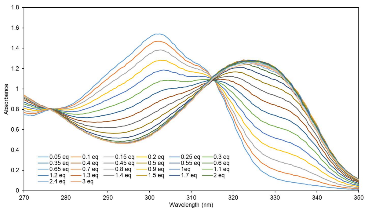
Figure 26. Absorption data for the titration test between L2 and \text{NiBr}_2 \cdot \text{DME} in DMA
