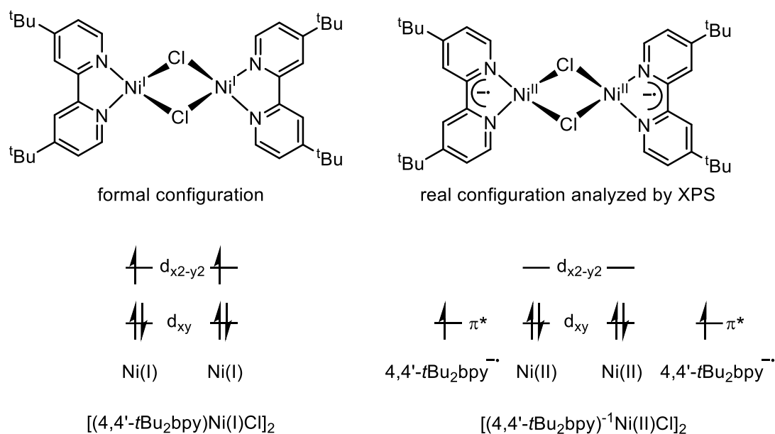
Figure 3. The electron configuration of [(4,4'\text{-tBu}_2\text{bpy})\text{NiCl}]_2
