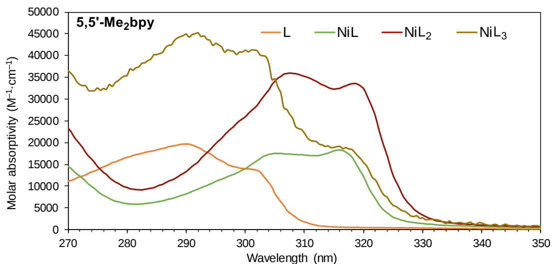
Figure 18. Calculated molar absorptivity curves with 5,5'-Me 2 bpy
