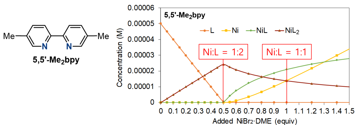
Figure 4. The concentration profile for Ni species with 5,5'-Me 2 bpy
