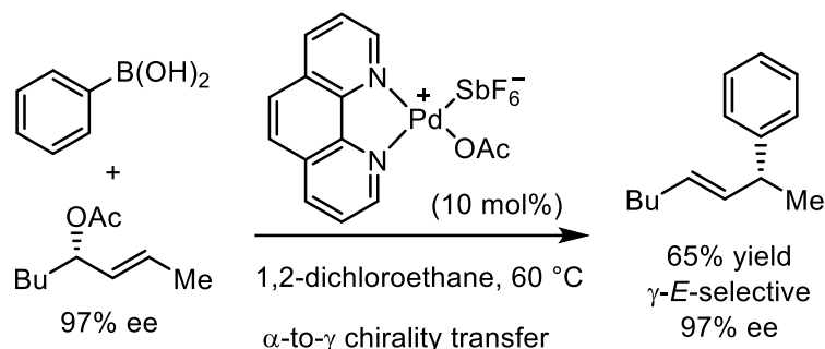
Scheme 11. Pd-catalyzed \gamma -E-selective coupling reaction of aryl boronic acids and vinyl acetates
