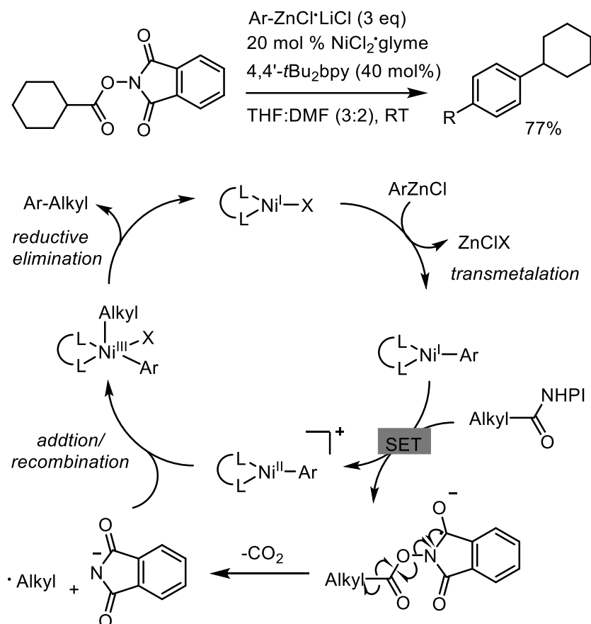
Scheme 21. Decarboxylative cross-coupling reaction using redox active esters
