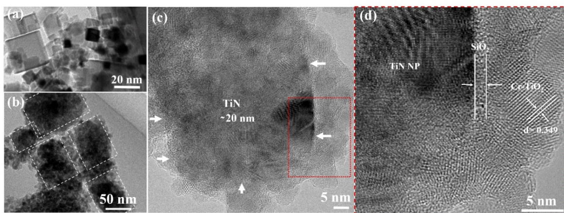
Figure 3. TEM images of (a) TiN NPs and (b) TSCT, where white boxes show TiN NPs covered with Cr-TiO 2 NPs. (c) HRTEM image of TSCT and (d) enlarged view of (c).
