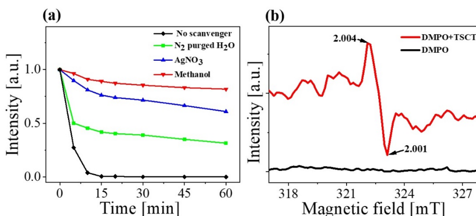
Figure 11. (a) Effect of different radical scavenger or quencher on the degradation process of methyl orange (MO) in presence of TSCT. (b) EPR spectra of 5, 5-Dimethyl-1-pyrroline N-oxide (DMPO) and an aqueous TSCT suspension to which DMPO and ethanol have been added.
