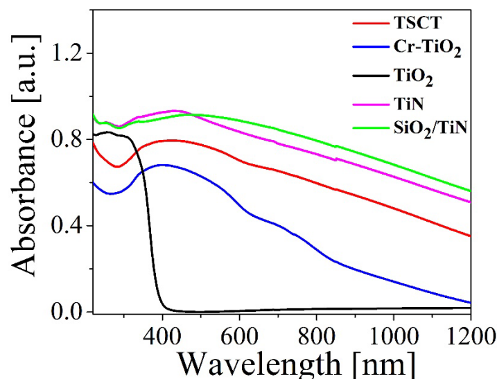
Figure 5. Absorbance spectra of TSCT, Cr-TiO 2 , TiO 2 , uncoated TiN and SiO 2 /TiN NPs.
