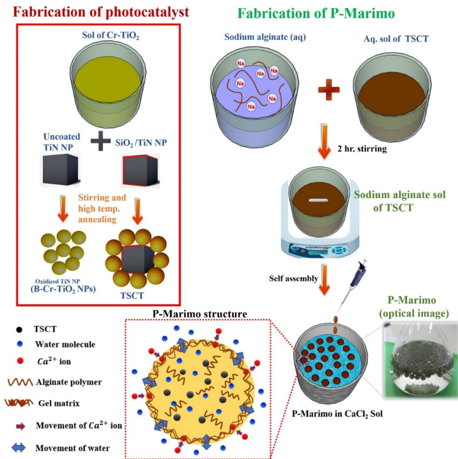
Figure 1. Schematic representation of TiN/SiO 2 /Cr-TiO 2 (TSCT) and B-Cr-TiO 2 nanostructure fabrication using with and without SiO 2 cladded TiN NPs, respectively. Fabrication of TSCT P-Marimo structure is also shown.
