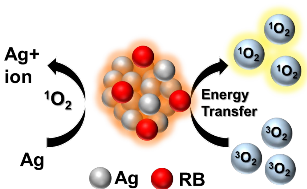
Scheme 1. Silver nanoclusters/rose bengal (AgNCs/RB) nanocomposite-based photosensitizer with dual antibacterial effects ( ^1\text{O}_2 and \text{Ag}^+ ions)
