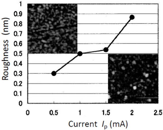
Figure 1. Root-mean-square surface roughness of GST films with thicknesses of 60 \pm 10 nm as a function of the plasma current I_p at V = 2.5 kV. The upper-left and the lower-right photographs exemplified the surfaces (side lengths of 500 nm) at I_p = 0.5 and 2 mA with black-white amplitudes of 3 and 6 nm, respectively.
