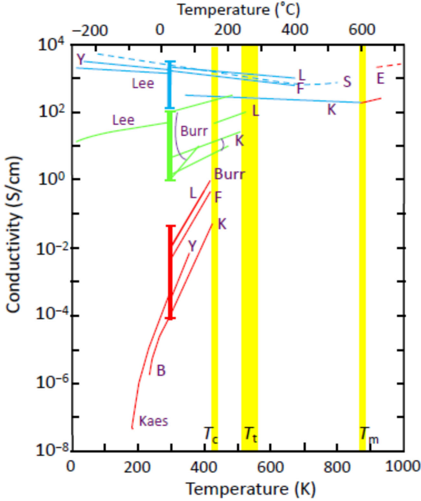
Figure 2. Temperature variations of electrical conductivities in amorphous (red), cubic (green), hexagonal (blue) and liquid (red) GST; B for Baily et al., [28] Burr et al., [17] E for Endo et al., [30] F for Friedrich et al., [24] Kaes et al., [31] K for Kato and Tanaka, [7] L for Lankhorst et al., [27] Lee et al., [6] S for Shelimova et al., [25] Y for Yamanaka et al. [26] Burr and L for amorphous films mostly overlap. Solid and dashed lines in the hexagonal [6,7,24-27] and liquid [7,30] phases are obtained, respectively, for films and for bulk samples. The two lines for the cubic films, Burr and K, are obtained upon cooling processes after annealing at different temperatures (140 – 250°C). Three error bars represent data scattering in amorphous, cubic and hexagonal films at room temperature, [15,22,29,31-33] and three yellow bands show the crystallization ( T_c ), transformation ( T_t ), and melting ( T_m ) temperatures. [1,2]
