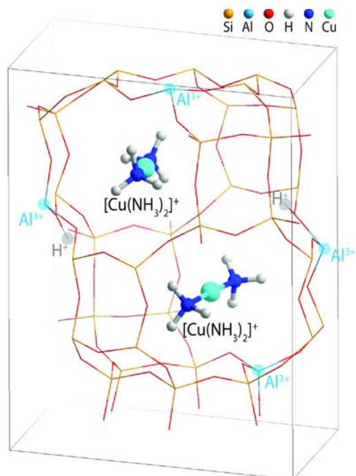
Fig. 1 Computational model of CHA unit cell with two [\text{Cu}(\text{NH}_3)_2]^+ cations and two Brønsted protons in the cage (36T, Si/Al=8).
