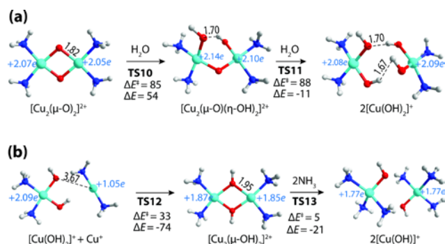
Fig. 6 (a) \text{H}_2\text{O} -assisted decomposition of a dimeric [\text{Cu}_2(\mu\text{-O})_2]^{2+} into two mononuclear [\text{Cu}(\text{OH})_2]^{+} intermediates; (b) \text{NH}_3 solvation assisted formation of two [\text{Cu}(\text{OH})]^{+} sites from the reaction of [\text{Cu}(\text{OH})_2]^{+} and Cu(I) ions. Zeolite frameworks are omitted for clarity. Atomic distances are given in Å. The Bader charges of Cu are normalized with reference to the bulk CuO (+2.00 e).
