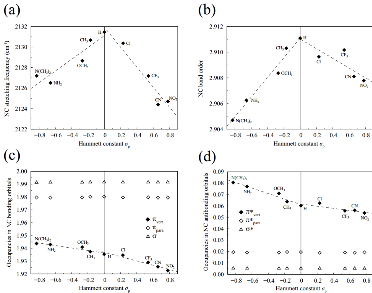
Figure 2. The calculated results for isolated X-C 6 H 4 -NC molecules: (a) NC stretching frequency, (b) NC bond order, (c) NBO occupancies in NC bonding orbitals ( \sigma and \pi ), and (d) NBO occupancies in NC antibonding orbitals ( \sigma^* and \pi^* ) for isolated X-C 6 H 4 -NC molecules, as a function of the Hammett constants.
