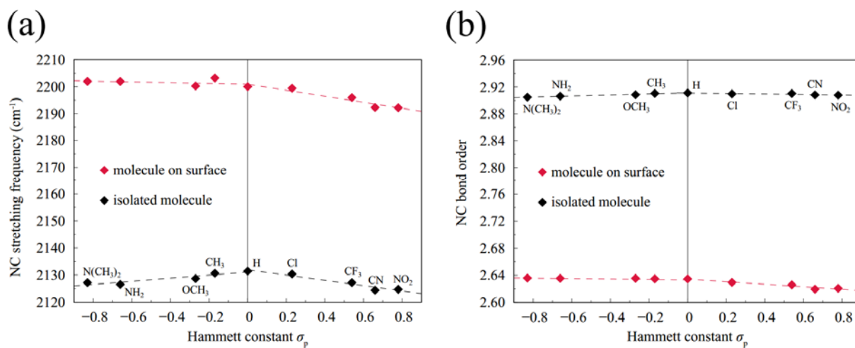
Figure 4. Variations of (a) NC stretching frequency and (b) NC bond order, plotted for X-C_6H_4-NC molecules as an isolated molecule (black), and those adsorbed on the Pt(111) surface (red) as a function of Hammett constant. The dashed lines represent the linear fit for the respective positive and negative regions of the Hammett constants.
