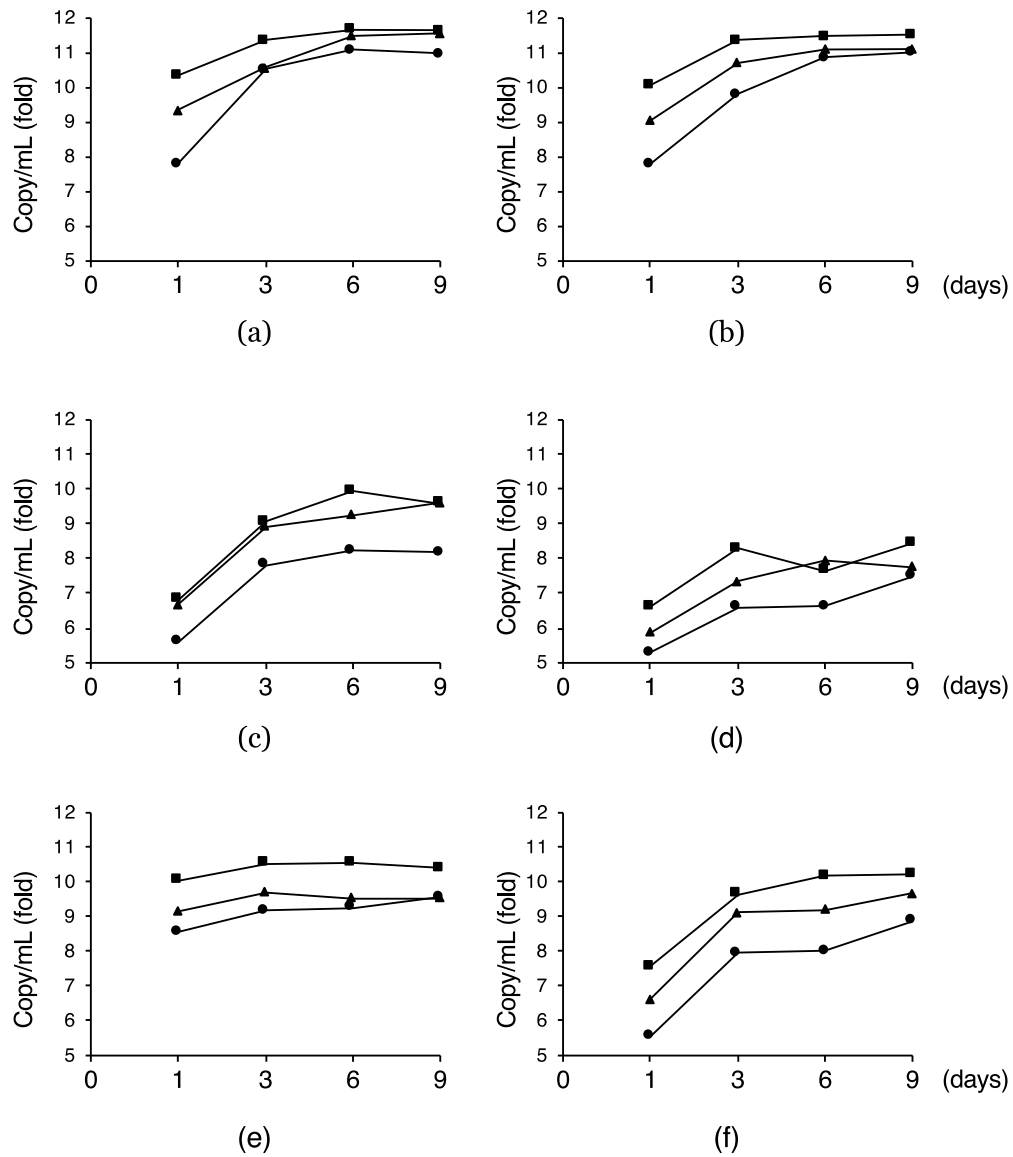
Figure 1. Time course analyses of HAdV DNA copy number at the indicated times by real-time PCR (1, 3, 6 and 9 days) after HAdV-B3 (a), HAdV-D8 (b), HAdV-D37 (c), HAdV-D53 (d), HAdV-D54 (e) and HAdV-D56 (f) infection (multiplicity of infection = 0.1; ●, 1; ▲, 10; ■) in A549 cells.
