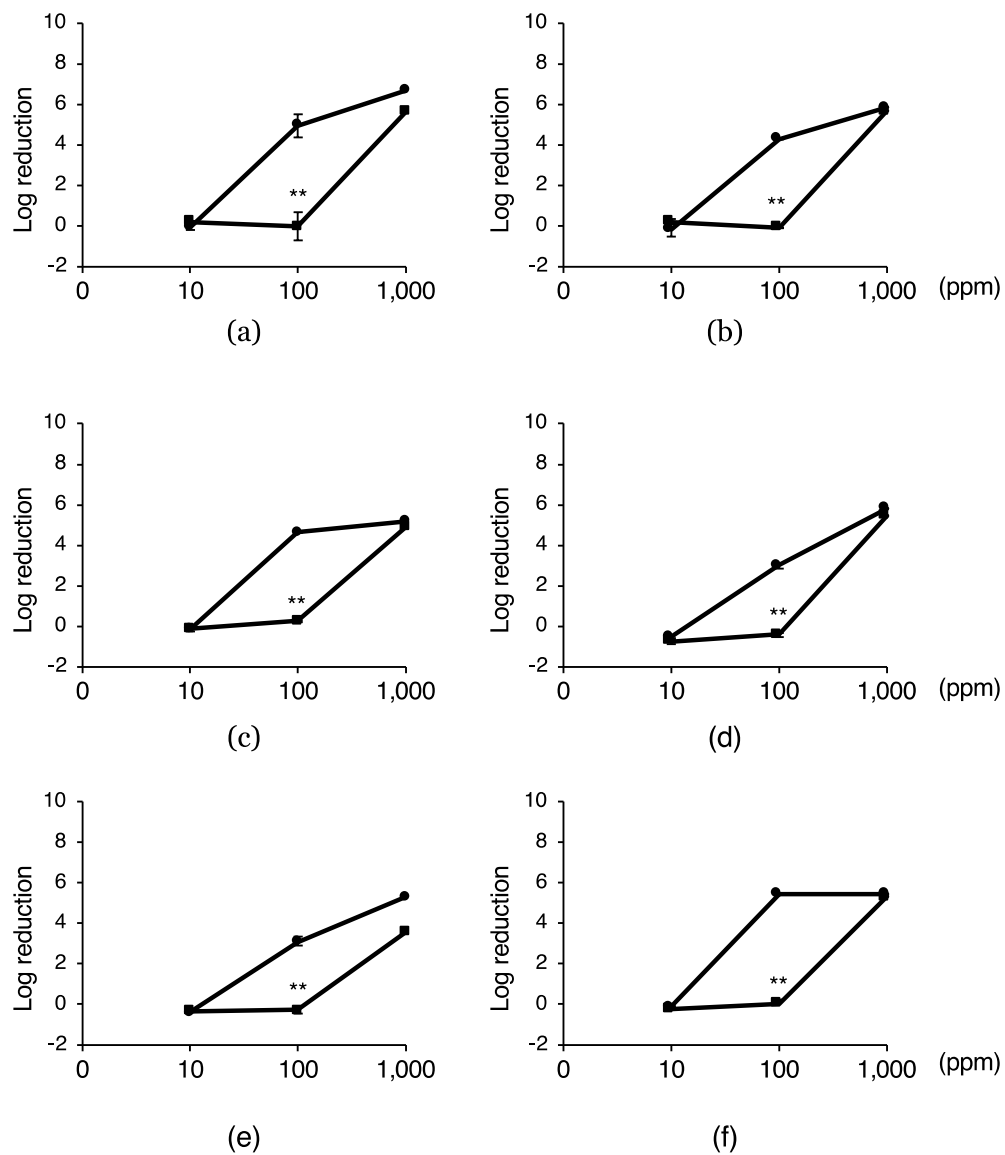
Figure 3. Effect of various concentration potassium peroxymonosulfate (circle) and sodium hypochlorite (square) on the inactivation of HAdV-B3 (a), HAdV-D8 (b), HAdV-D37 (c), HAdV-D53 (d), HAdV-D54 (e) and HAdV-D56 (f) for 1min. ** P < 0.01 vs potassium peroxymonosulfate. Data are presented as mean and standard deviation (n=3).
