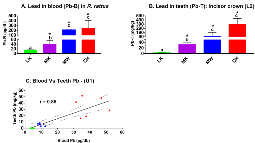
Fig 3.2.5. Mean \pm SD of Pb-B and Pb-T of environmentally Pb exposed Rattus rattus rats. A. Lead level in blood (Pb-B) in rats sampled from Lukanga (LK; n = 2 ); Makululu (MK; n = 5 ); Mutwe Wansofu (MW; n = 3 ) and Chowa (CH; n = 5 ). B. Lead in teeth (Pb-T) in rats sampled from LK ( n = 2 ); MK ( n = 5 ); MW ( n = 3 ) and CH ( n = 5 ); ( a,b, c, d, e represent p < 0.05 , Tukey's multiple comparison test). Significant difference between the control and exposure groups, * at p < 0.05 , Turkey's multiple comparison test. C. Log transformed Pearson's correlations of Pb-B Vs Pb-T in environmentally exposed Rattus rattus rats ( r = 0.85 , p < 0.05 ).
