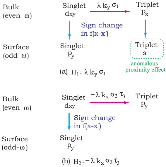
FIG. 4. The pairing correlations appearing in a d_{xy} -wave superconductor. At the surface of a d_{xy} -wave superconductor, an odd-frequency spin-singlet p_y -wave pairing correlation always appears as a result of the sign change in the d_{xy} -wave pairing correlation under x \leftrightarrow x' . In (a), a spin-orbit interaction \lambda k_y \hat{\sigma}_1 induces spin-triplet p_x -wave pairing correlation in bulk. An odd-frequency spin-triplet s -wave component appears at the surface as a result of the sign change of the p_x -wave pairing correlation. In (b), -\lambda k_x \hat{\sigma}_2 \hat{\tau}_3 induces a spin-triplet p_y -wave pairing correlation in bulk, while this interaction does not generate an odd-frequency spin-triplet s -wave correlation at the surface.
