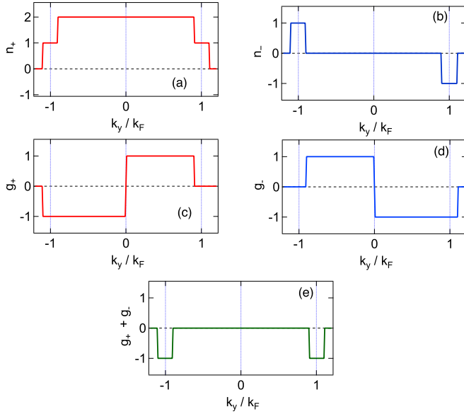
FIG. 3. In (a), n_+(k_y) represents the number of propagating channels at k_y . n_-(k_y) in (b) is an odd function of k_y . The chiral eigenvalues of the ZESs g_+ and g_- are plotted in (c) and (d), respectively. In (e), the summation of the chiral eigenvalues g_+ + g_- is shown. n_-(k_y) in (b) and g_+ + g_- in (e) are nonzero at (I) and (III) in Fig. 2(a).
