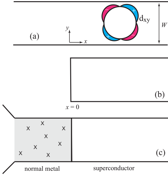
FIG. 1. Schematic pictures of superconducting proximity structures. A spin-singlet d_{xy} -wave superconductor is infinitely long in the x direction in (a). The width of the superconductor is W in the y direction. The Green's function at a surface is calculated for a semi-infinite superconductor as shown in (b). We attach a normal metal to a superconductor at x = 0 in (c), where “cross” symbols represent impurities. A Cooper pair penetrates into the normal metal and causes the proximity effect.
