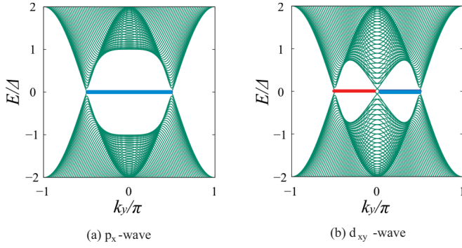
FIG. 5. The eigenvalues of the BdG Hamiltonian on a two-dimensional tight-binding model are plotted as a function of the wave number in the y direction. The results for a p_x -wave superconductor in (a) have nodes at k_y = \pm k_F with k_F = \pi/2 . The surface Andreev bound states are degenerate at E = 0 as indicated by a line between the two nodal points. All of the ZESs belong to the same chiral eigenvalue of \tilde{\Gamma}_{\text{BDI}} . In (b), the results for a d_{xy} -wave superconductor are shown. An additional nodal point appears at k_y = 0 . ZESs for k_y > 0 and those for k_y < 0 belong to the opposite chiral eigenvalue of \tilde{\Gamma}_{\text{BDI}} .
