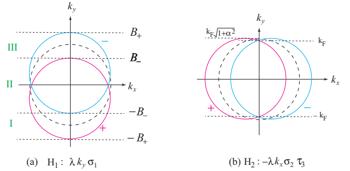
FIG. 2. The two Fermi surfaces for H_1 and those for H_2 are illustrated in (a) and (b), respectively. In (a), the lower (upper) circle indicated by “+” (“-”) represents a Fermi surface calculated from \xi_{1,+}(\mathbf{k}) = 0 [ \xi_{1,-}(\mathbf{k}) = 0 ]. In (b), the left (right) circle represents a Fermi surface calculated from \xi_{2,+}(\mathbf{k}) = 0 [ \xi_{2,-}(\mathbf{k}) = 0 ].
