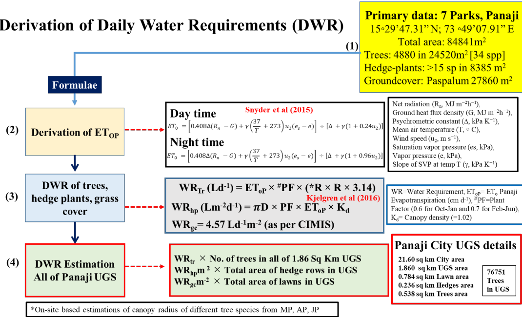
Fig 3. Derivation of daily water requirements of trees, hedge-plants and grass cover using field data and the local evapotranspiration rate derived during this study
